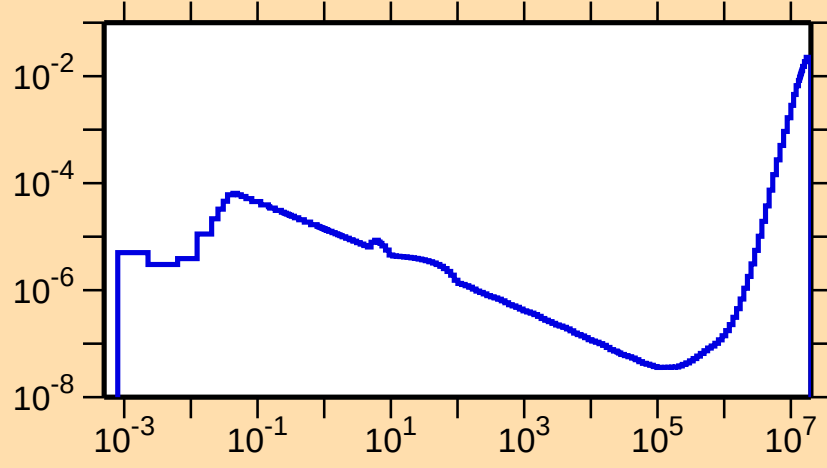
\sigma vs. E for ^{165}\text{W}(n,p\alpha)
