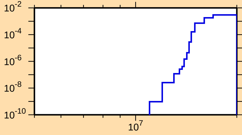
\sigma vs. E for ^{165}\text{W}(n,2n\alpha)
