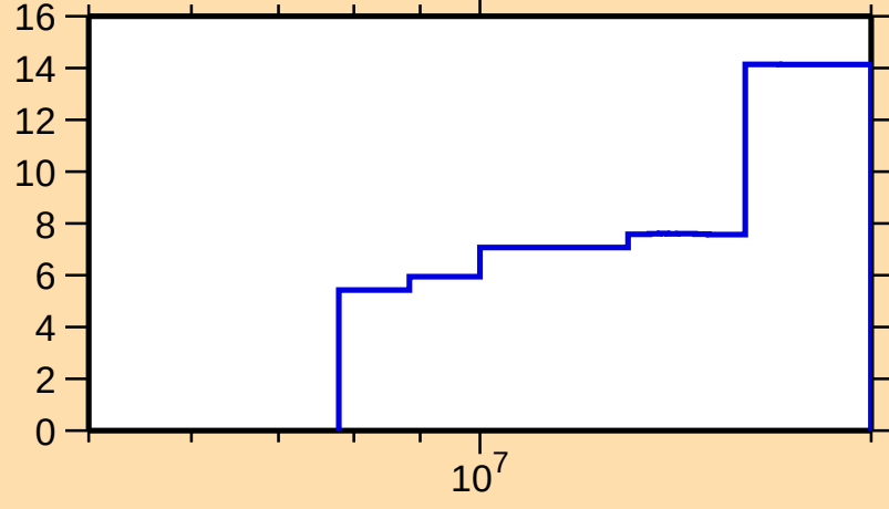
\Delta\sigma/\sigma vs. E for ^{165}\text{W}(n,\text{tot.})
