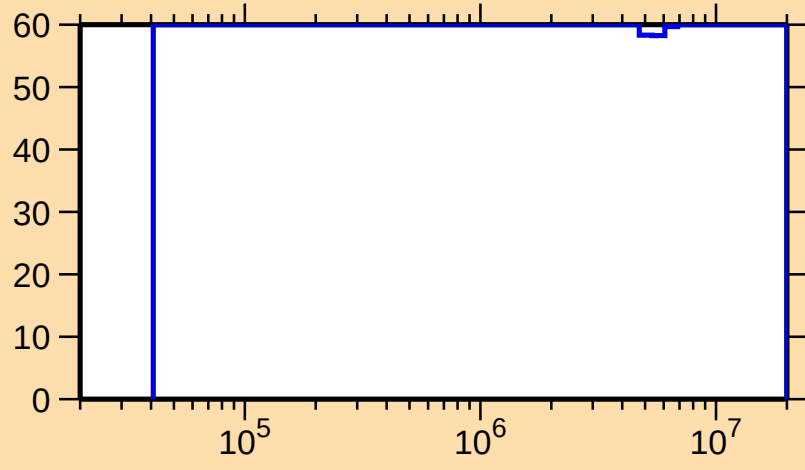
\Delta\sigma/\sigma vs. E for ^{165}\text{W}(n,\text{inel.})
