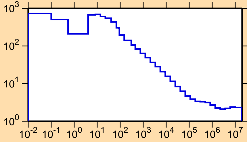
\sigma vs. E for ^{165}\text{W}(n,\text{nonel.})
