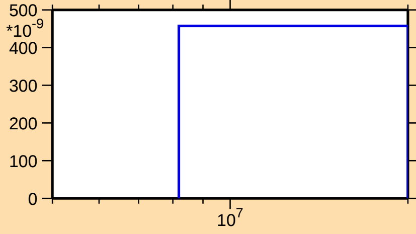
\sigma vs. E for ^{165}\text{W}(n,\text{pt})
