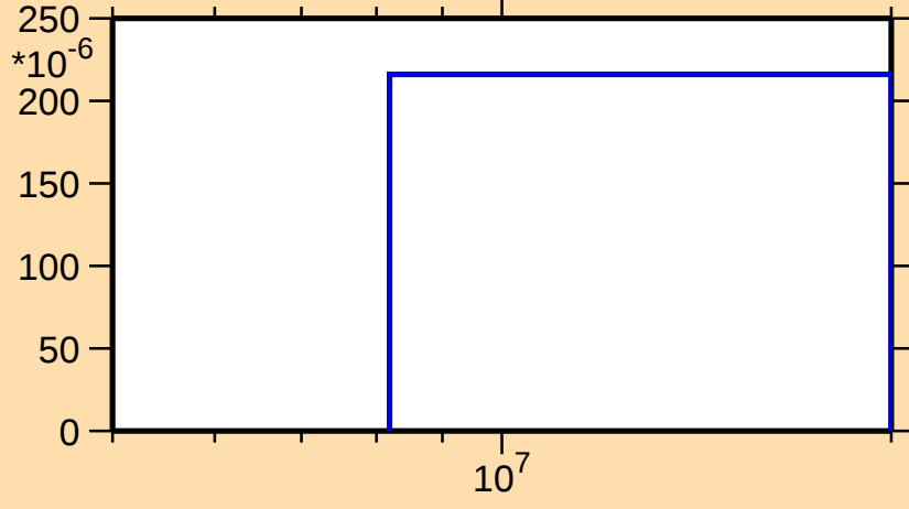
\sigma vs. E for ^{165}\text{W}(n,2np)
