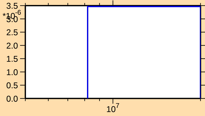
\sigma vs. E for ^{165}\text{W}(n,\text{pd})
