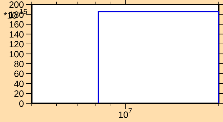
\sigma vs. E for ^{165}\text{W}(n,nt)
