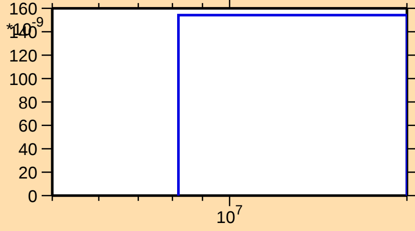
\sigma vs. E for ^{165}\text{W}(n,\text{nd})
