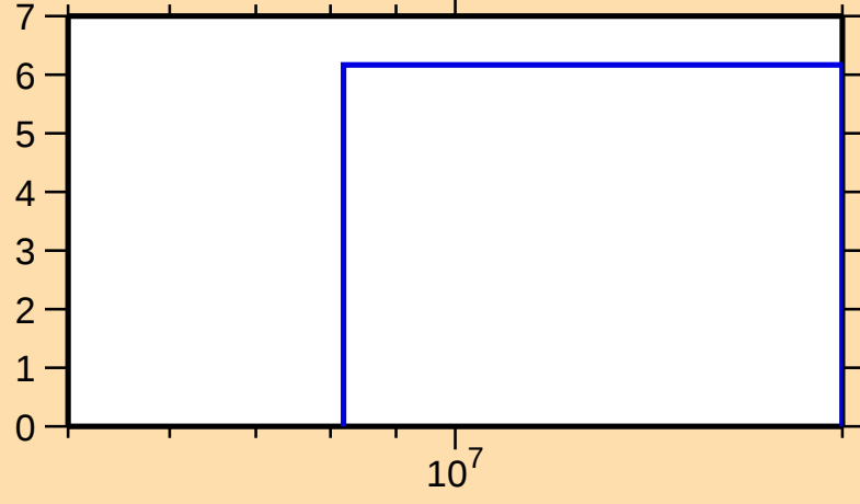
\Delta\sigma/\sigma vs. E for ^{165}\text{W}(n,\text{tot.})
