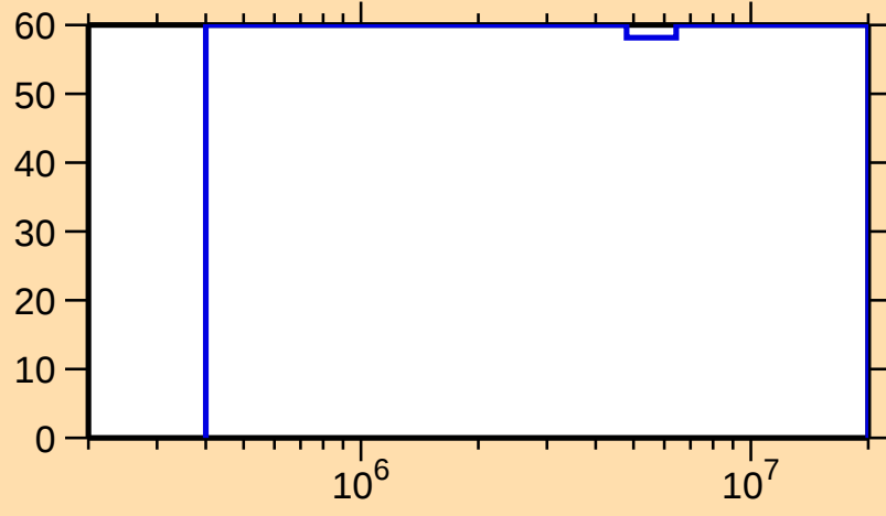
\Delta\sigma/\sigma vs. E for ^{165}\text{W}(\text{n,inel.})
