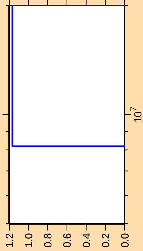
\Delta\sigma/\sigma vs. E for ^{165}\text{W}(n,nt)
