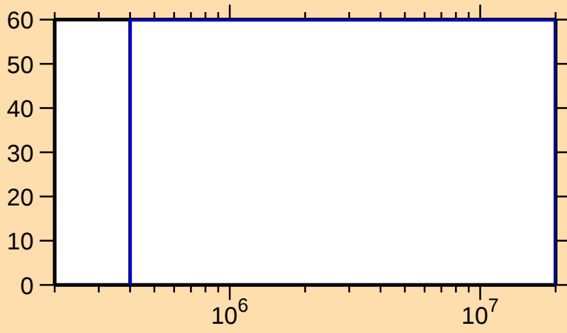
\Delta\sigma/\sigma vs. E for ^{165}\text{W}(n,n_1)
