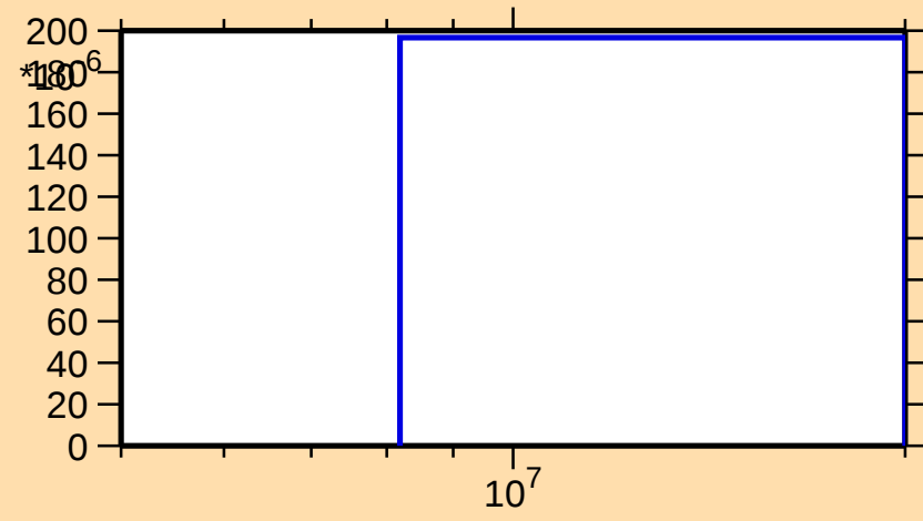
\sigma vs. E for ^{165}\text{W}(n,2n\alpha)
