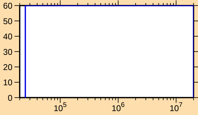
\Delta\sigma/\sigma vs. E for ^{165}\text{W}(n,n_1)
