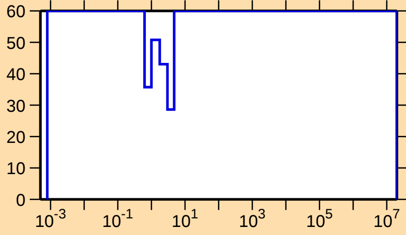
\Delta\sigma/\sigma vs. E for ^{165}\text{W}(n,\gamma)
