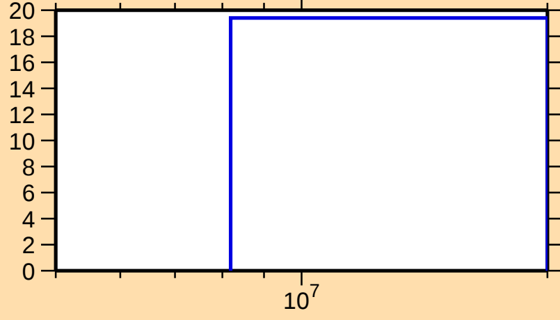
\Delta\sigma/\sigma vs. E for ^{165}\text{W}(n,\text{nonel.})
