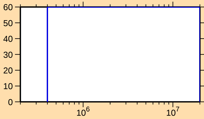
\Delta\sigma/\sigma vs. E for ^{165}\text{W}(n,n\text{cont.})
