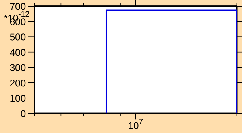
\sigma vs. E for ^{165}\text{W}(\text{mt } 34)
