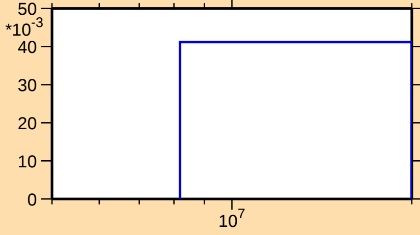
\sigma vs. E for ^{165}\text{W}(n,2n)
