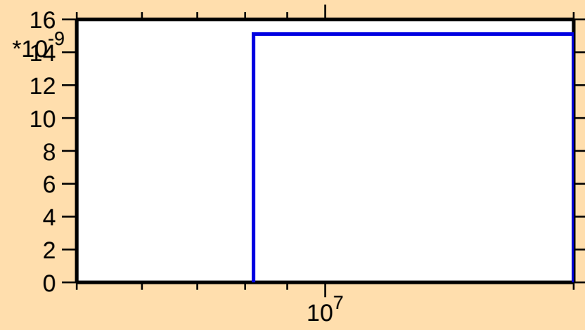
\sigma vs. E for ^{165}\text{W}(\text{mt117})
