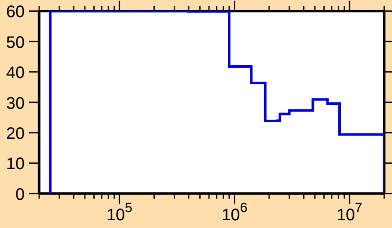
\Delta\sigma/\sigma vs. E for ^{165}\text{W}(n,\text{nonel.})
