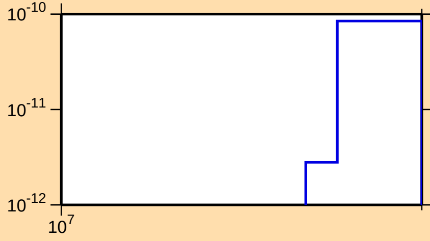
\sigma vs. E for ^{166}\text{W}(\text{mt } 34)
