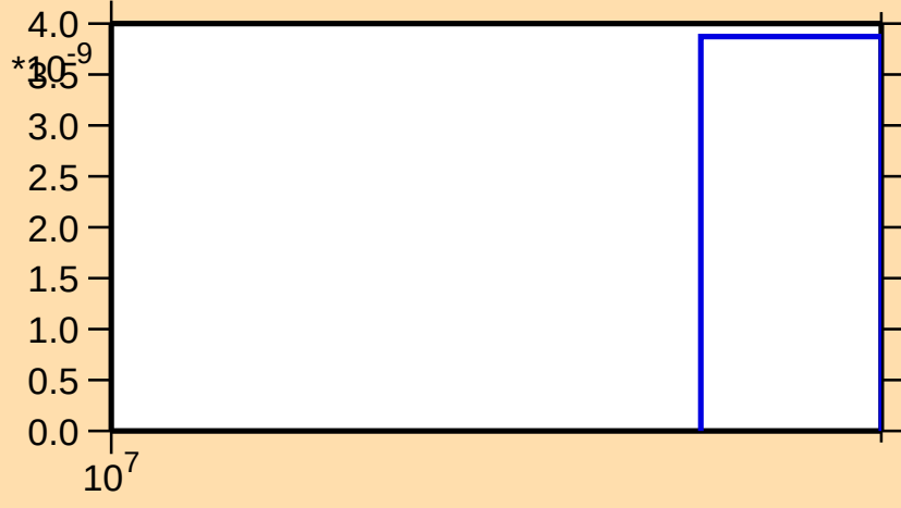
\sigma vs. E for ^{166}\text{W}(n,3n)
