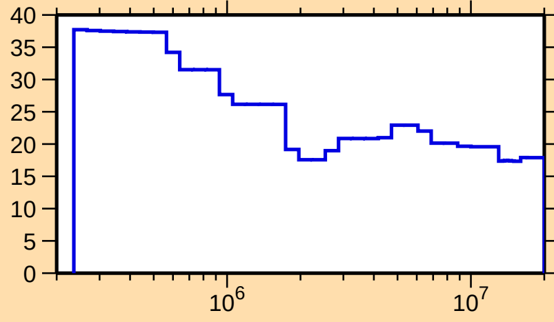
\Delta\sigma/\sigma vs. E for ^{166}\text{W}(\text{n,nonel.})
