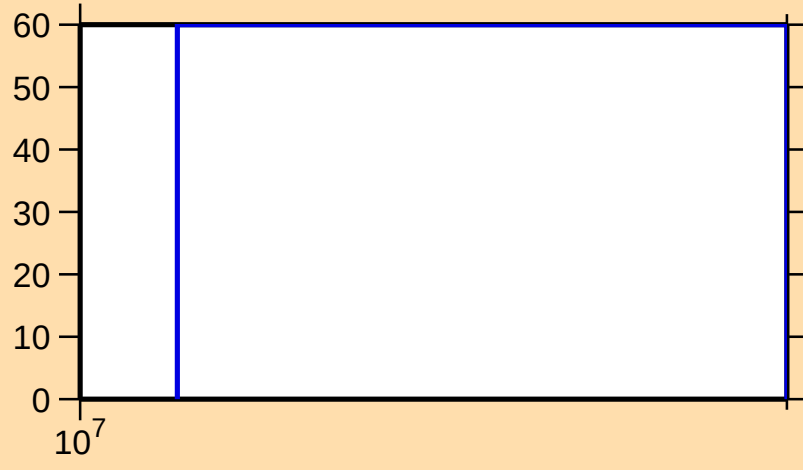
\Delta\sigma/\sigma vs. E for ^{166}\text{W}(n,2n)
