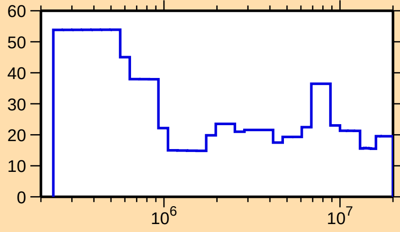
\Delta\sigma/\sigma vs. E for ^{166}\text{W}(\text{n,el.})
