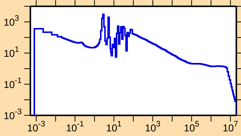
\sigma vs. E for ^{166}\text{W}(n,\gamma)
