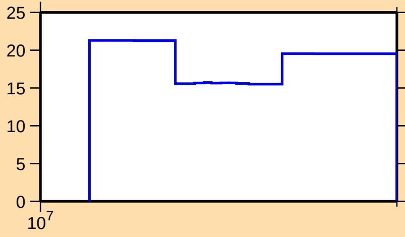
\Delta\sigma/\sigma vs. E for ^{166}\text{W}(n,\text{el.})
