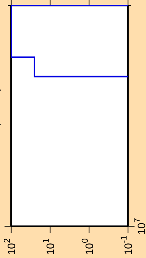
\Delta\sigma/\sigma vs. E for ^{166}\text{W}(\text{mt } 34)
