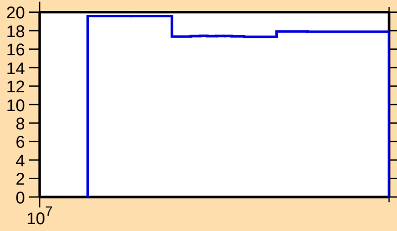
\Delta\sigma/\sigma vs. E for ^{166}\text{W}(n,\text{nonel.})
