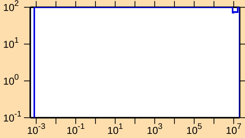
\Delta\sigma/\sigma vs. E for ^{166}\text{W}(n,p)
