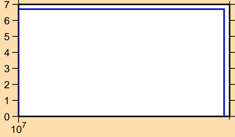
\Delta\sigma/\sigma vs. E for ^{166}\text{W}(n,\text{tot.})
