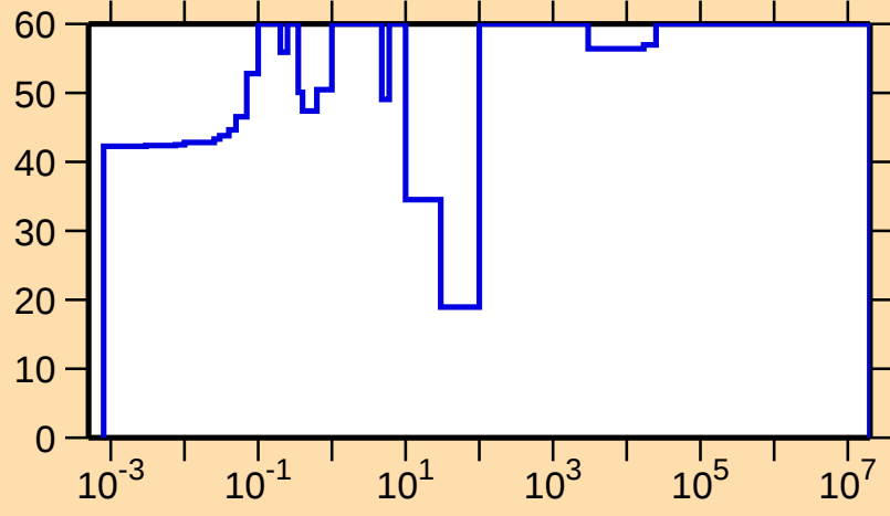
\Delta\sigma/\sigma vs. E for ^{166}\text{W}(n,\gamma)
