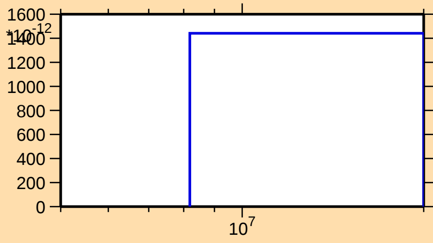
\sigma vs. E for ^{166}\text{W}(n,\text{nd})
