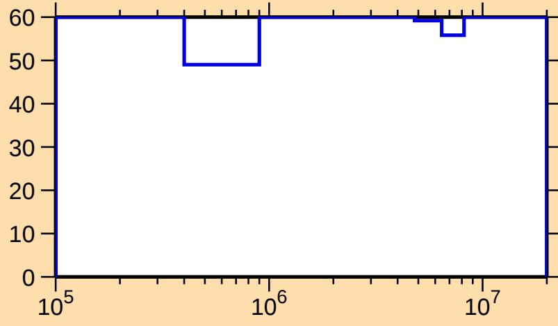
\Delta\sigma/\sigma vs. E for ^{166}\text{W}(n,\text{inel.})
