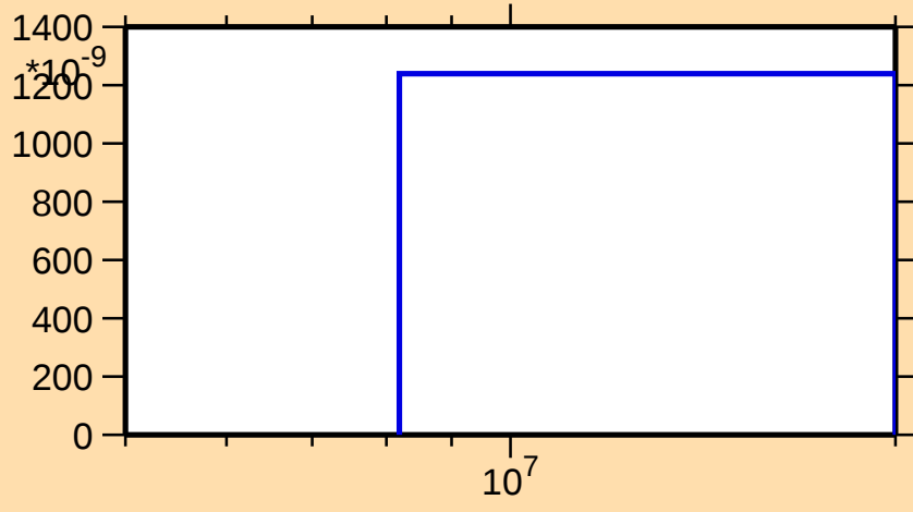
\sigma vs. E for ^{166}\text{W}(n,\text{pd})
