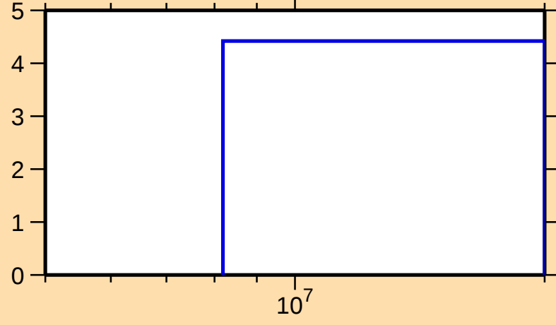
\Delta\sigma/\sigma vs. E for ^{166}\text{W}(n,\text{tot.})
