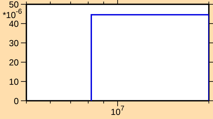
\sigma vs. E for ^{166}\text{W}(n,t)
