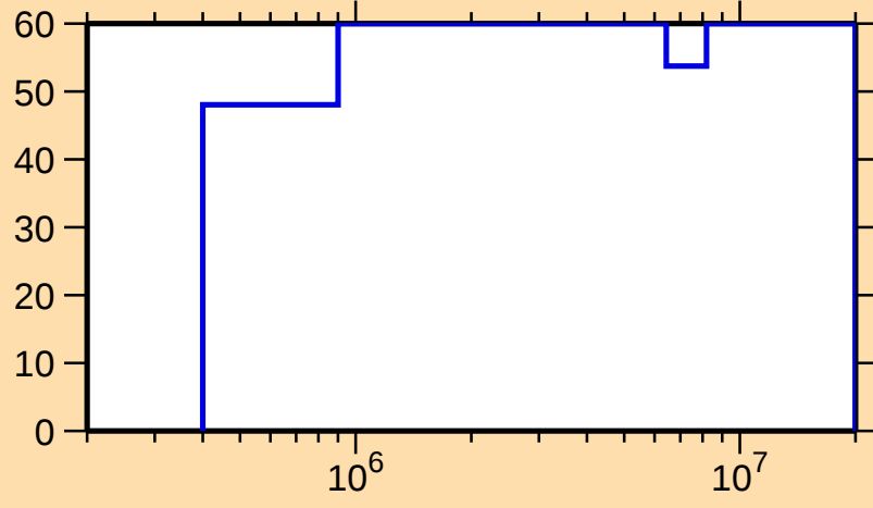
\Delta\sigma/\sigma vs. E for ^{166}\text{W}(n,n_1)
