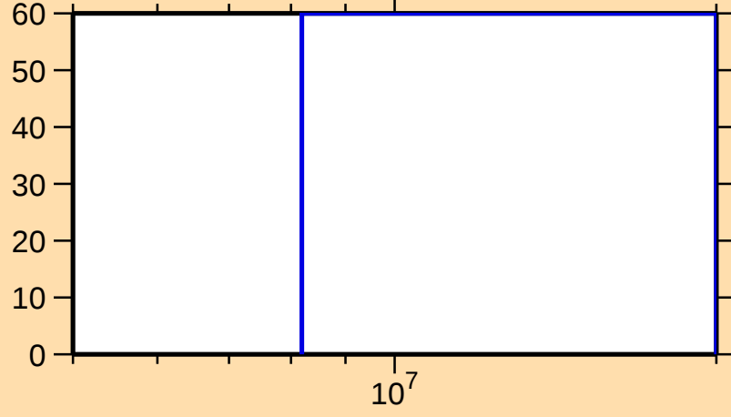
\Delta\sigma/\sigma vs. E for ^{166}\text{W}(n,\text{inel.})
