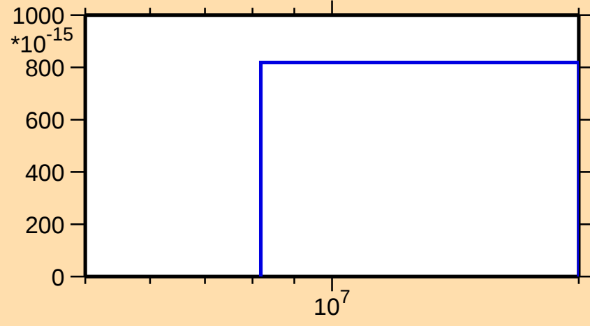
\sigma vs. E for ^{166}\text{W}(\text{mt } 34)
