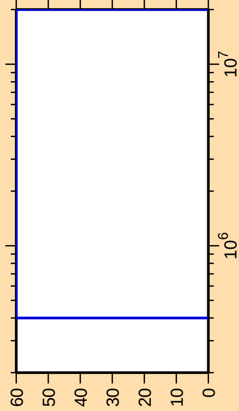
\Delta\sigma/\sigma vs. E for ^{166}\text{W}(n,\text{ncont.})
