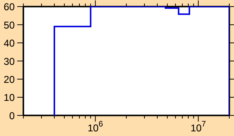
\Delta\sigma/\sigma vs. E for ^{166}\text{W}(\text{n},\text{inel.})
