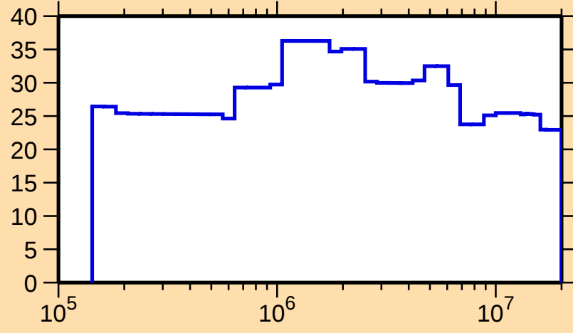
\Delta\sigma/\sigma vs. E for ^{167}\text{W}(\text{n,nonel.})
