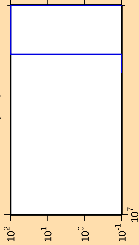
\Delta\sigma/\sigma vs. E for ^{167}\text{W}(n,nt)
