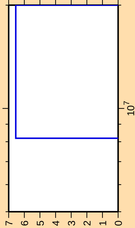
\Delta\sigma/\sigma vs. E for ^{167}\text{W}(n,nt)
