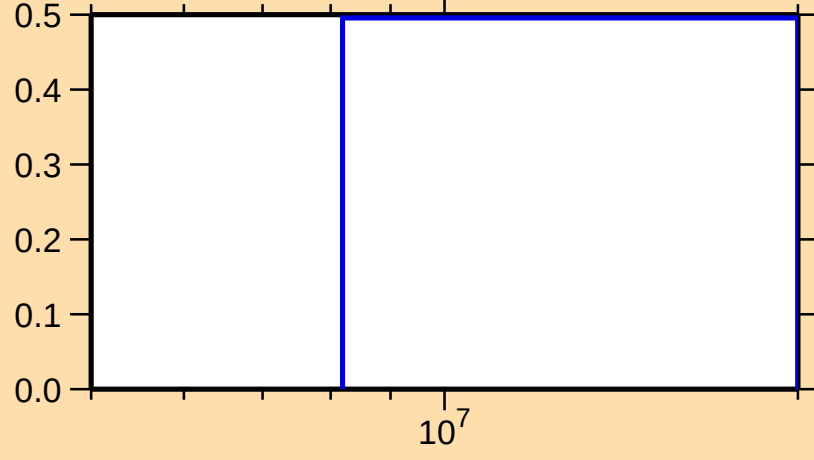
\sigma vs. E for ^{167}\text{W}(n,2n)
