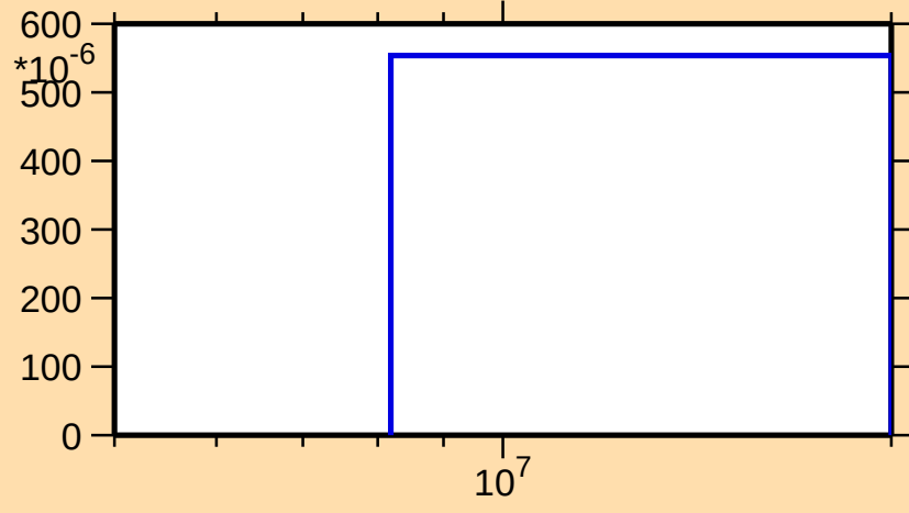
\sigma vs. E for ^{167}\text{W}(n,2n\alpha)
