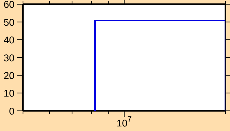
\Delta\sigma/\sigma vs. E for ^{167}\text{W}(n,\text{inel.})
