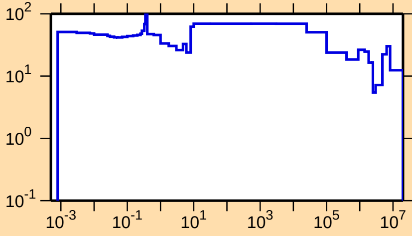
\Delta\sigma/\sigma vs. E for ^{167}\text{W}(n,\text{tot.})
