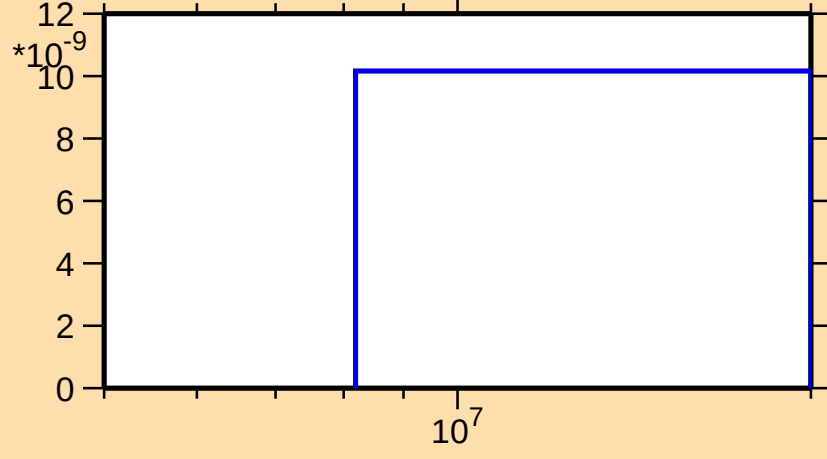
\sigma vs. E for ^{167}\text{W}(n,3n)
