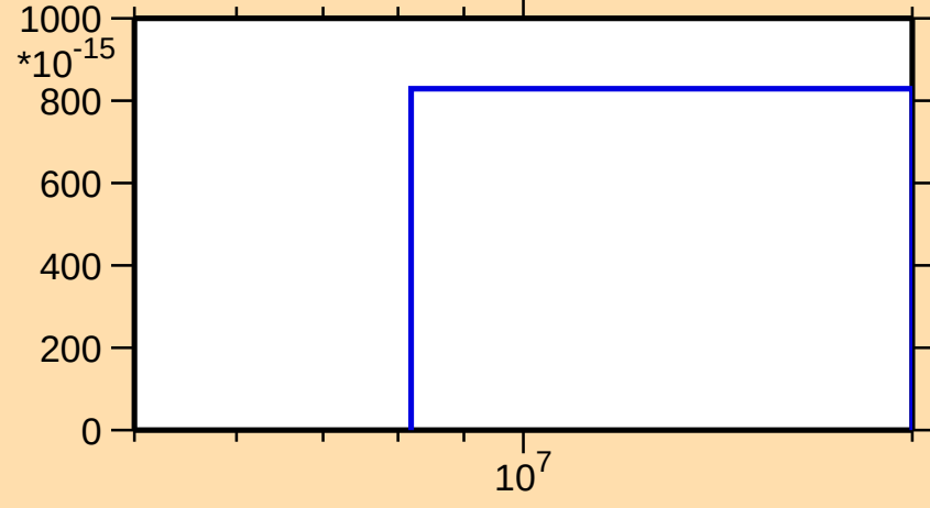
\sigma vs. E for ^{167}\text{W}(n,nt)
