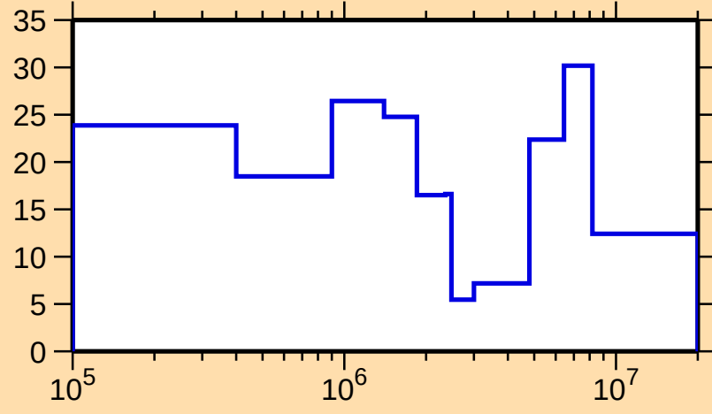
\Delta\sigma/\sigma vs. E for ^{167}\text{W}(\text{n,tot.})
