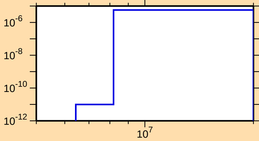
\sigma vs. E for ^{167}\text{W}(n,\text{He3})
