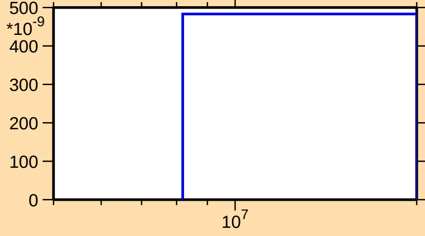
\sigma vs. E for ^{167}\text{W}(n,\text{pd})
