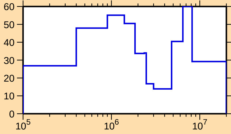
\Delta\sigma/\sigma vs. E for ^{167}\text{W}(n,\text{el.})
