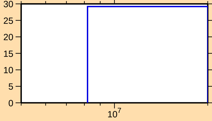
\Delta\sigma/\sigma vs. E for ^{167}\text{W}(n,\text{el.})
