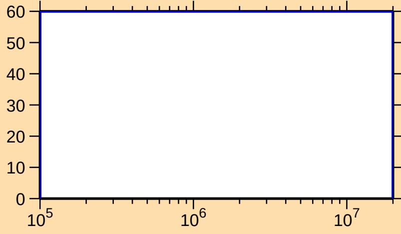
\Delta\sigma/\sigma vs. E for ^{167}\text{W}(n,ncont.)
