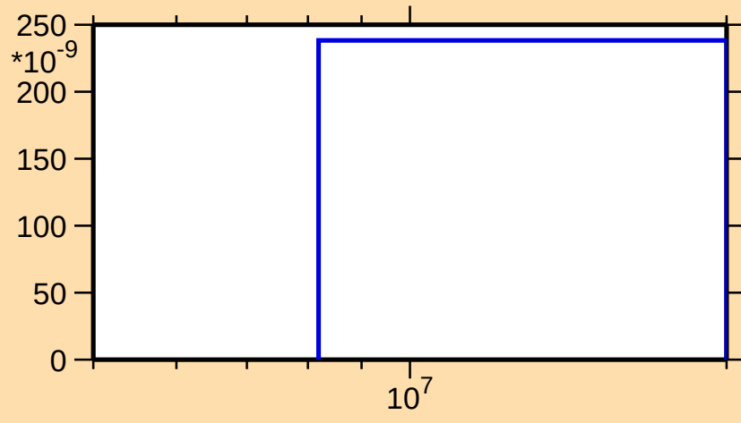
\sigma vs. E for ^{167}\text{W}(\text{n},\text{nd})
