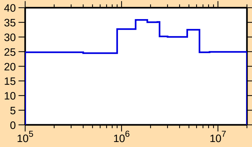
\Delta\sigma/\sigma vs. E for ^{167}\text{W}(\text{n},\text{nonel.})
