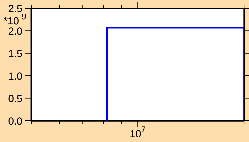
\sigma vs. E for ^{167}\text{W}(\text{mt117})
