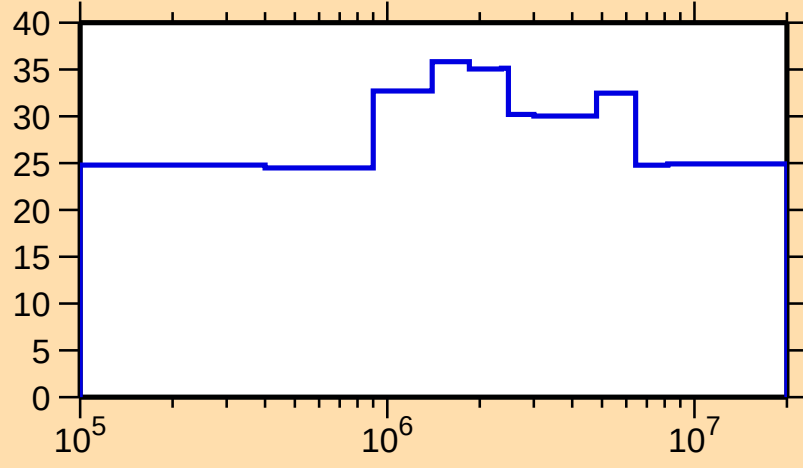
\Delta\sigma/\sigma vs. E for ^{167}\text{W}(\text{n,nonel.})
