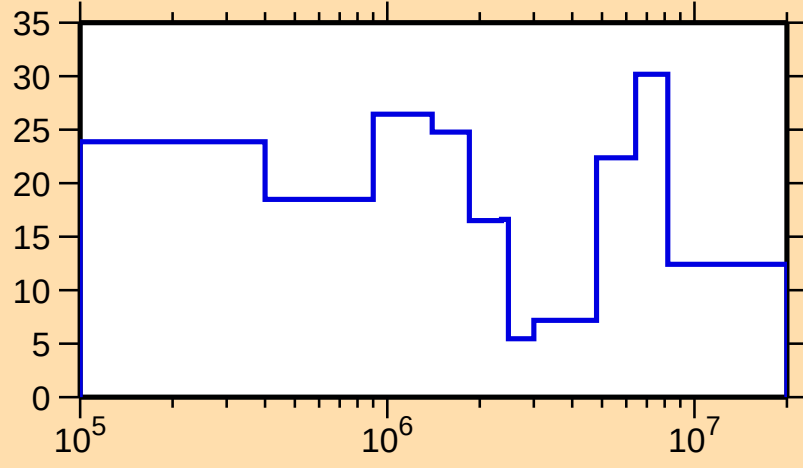
\Delta\sigma/\sigma vs. E for ^{167}\text{W}(n,\text{tot.})
