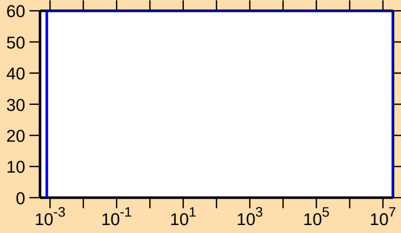
\Delta\sigma/\sigma vs. E for ^{167}\text{W}(n,p)
