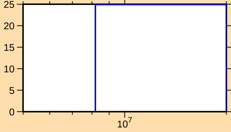
\Delta\sigma/\sigma vs. E for ^{167}\text{W}(n,\text{nonel.})
