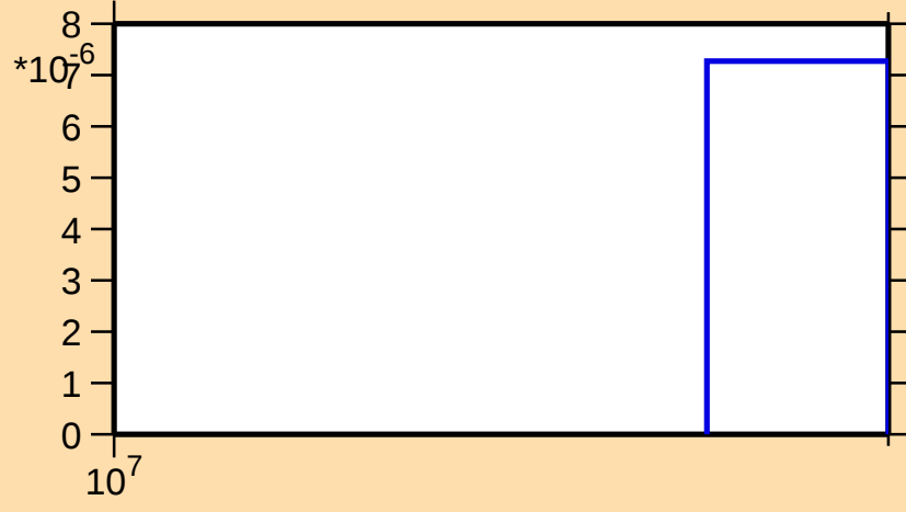
\sigma vs. E for ^{168}\text{W}(n,3n)
