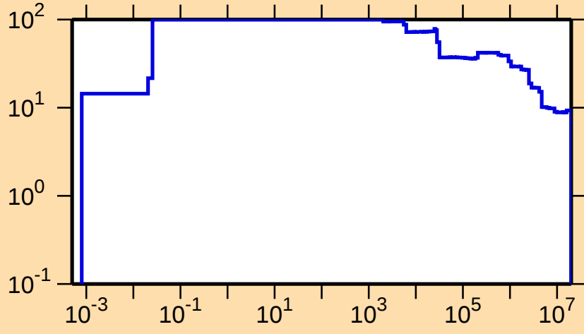
\Delta\sigma/\sigma vs. E for ^{168}\text{W}(n,\text{nonel.})
