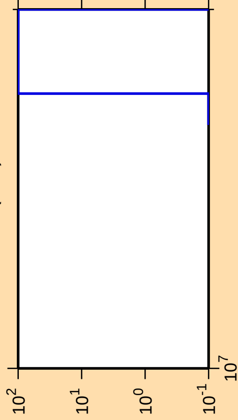
\Delta\sigma/\sigma vs. E for ^{168}\text{W}(n,nt)
