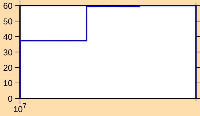
\Delta\sigma/\sigma vs. E for ^{168}\text{W}(n,\text{inel.})
