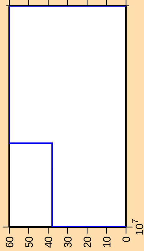
\Delta\sigma/\sigma vs. E for ^{168}\text{W}(n,n\text{cont.})
