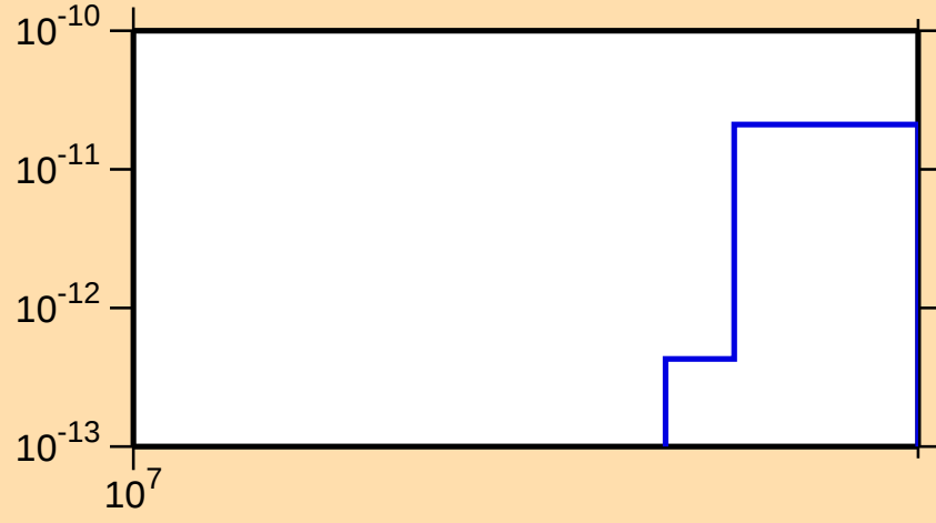
\sigma vs. E for ^{168}\text{W}(\text{mt 34})
