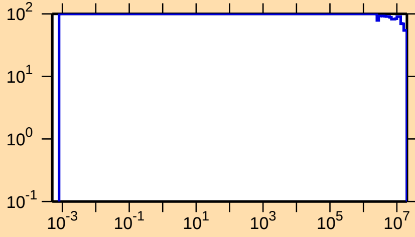
\Delta\sigma/\sigma vs. E for ^{168}\text{W}(n,p)
