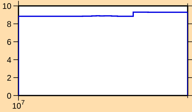
\Delta\sigma/\sigma vs. E for ^{168}\text{W}(n,\text{nonel.})
