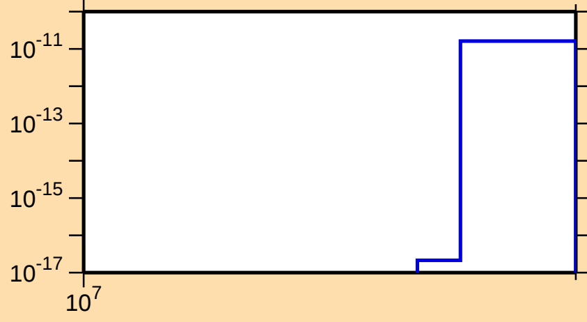
\sigma vs. E for ^{168}\text{W}(n,nt)
