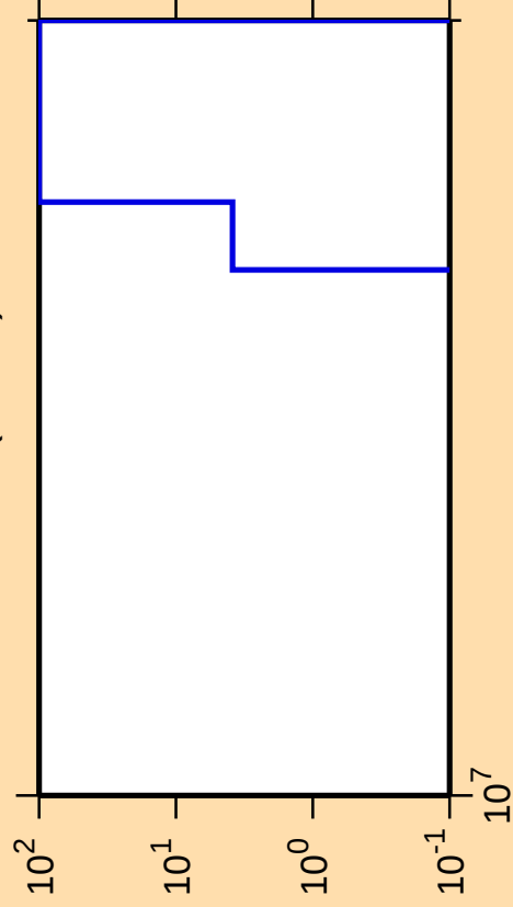
\Delta\sigma/\sigma vs. E for ^{168}\text{W}(\text{mt 34})
