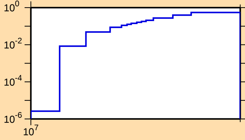
\sigma vs. E for ^{168}\text{W}(n,2n)
