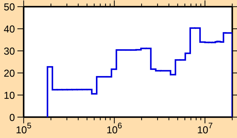
\Delta\sigma/\sigma vs. E for ^{168}\text{W}(n,\text{el.})
