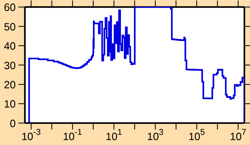
\Delta\sigma/\sigma vs. E for ^{168}\text{W}(n,\text{tot.})
