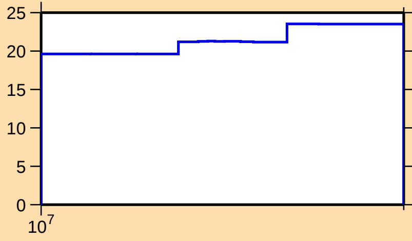
\Delta\sigma/\sigma vs. E for ^{168}\text{W}(n,\text{tot.})
