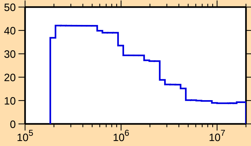
\Delta\sigma/\sigma vs. E for ^{168}\text{W}(\text{n,nonel.})
