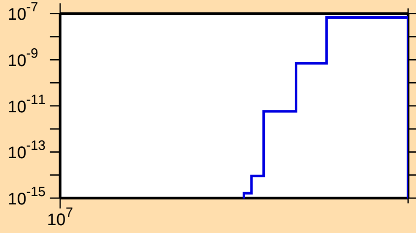
\sigma vs. E for ^{168}\text{W}(n,\text{nd})
