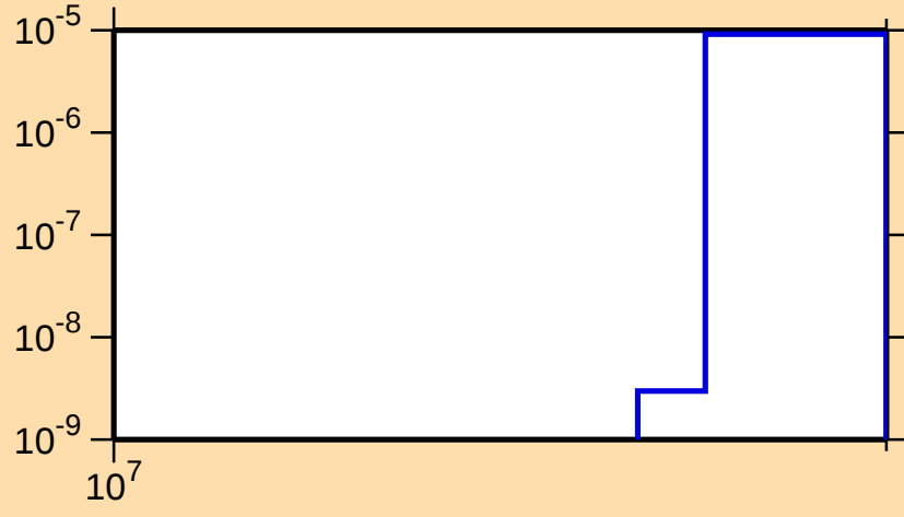
\sigma vs. E for ^{168}\text{W}(n,2np)
