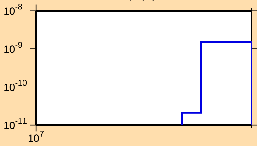
\sigma vs. E for ^{168}\text{W}(n,\text{pt})
