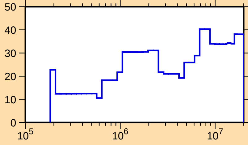
\Delta\sigma/\sigma vs. E for ^{168}\text{W}(\text{n,el.})
