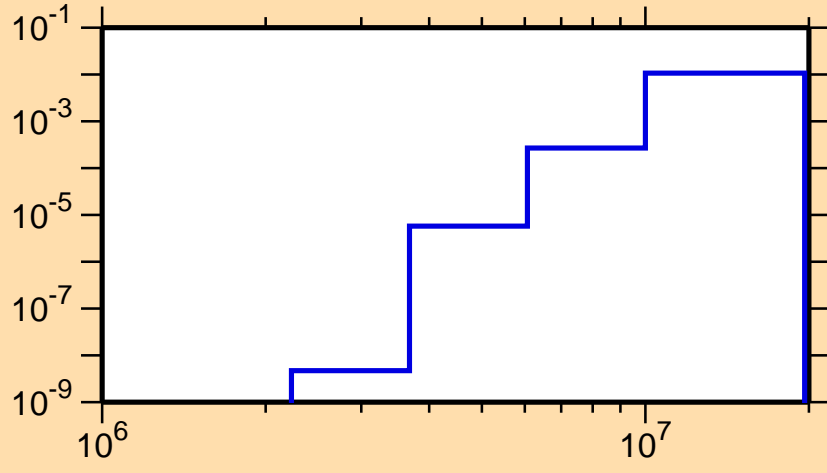
\sigma vs. E for ^{168}\text{W}(n,n\alpha)
