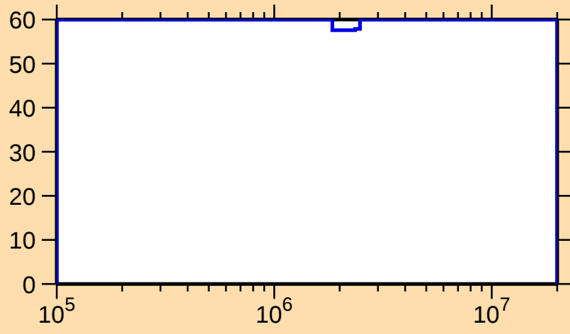
\Delta\sigma/\sigma vs. E for ^{168}\text{W}(n,n_1)
