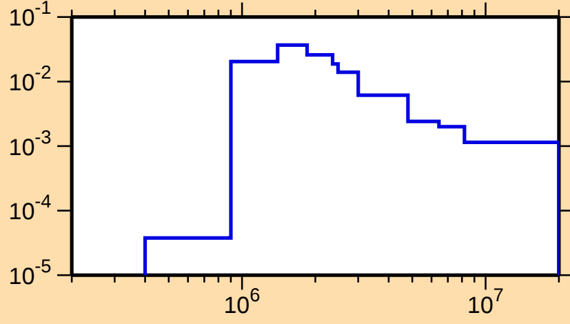
\sigma vs. E for ^{168}\text{W}(n,n_3)
