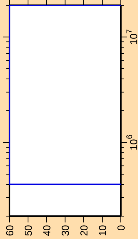
\Delta\sigma/\sigma vs. E for ^{168}\text{W}(n,n_3)
