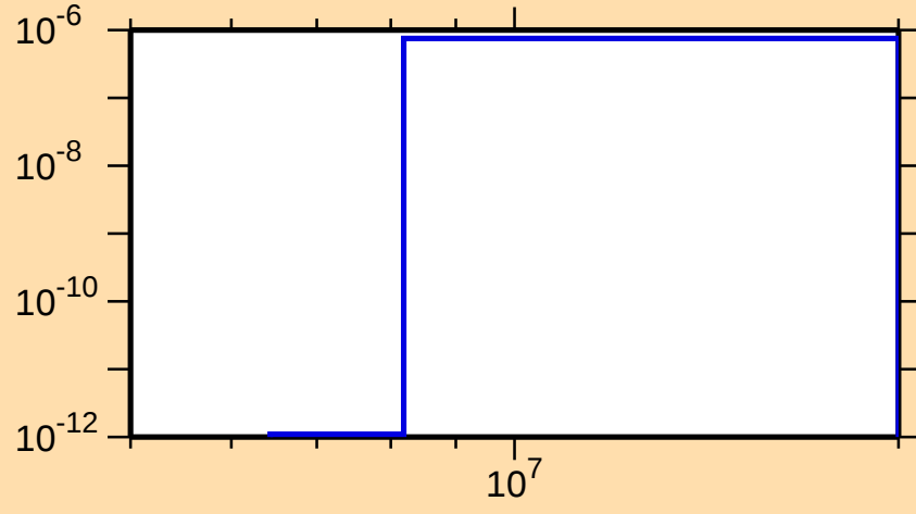
\sigma vs. E for ^{168}\text{W}(n,\text{He3})
