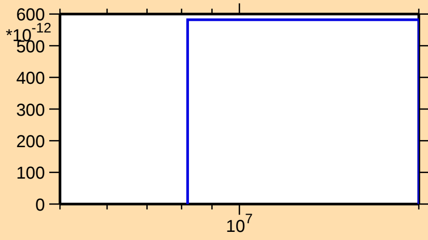
\sigma vs. E for ^{168}\text{W}(n,\text{nd})
