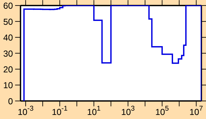
\Delta\sigma/\sigma vs. E for ^{168}\text{W}(n,\gamma)
