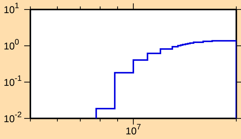
\sigma vs. E for ^{169}\text{W}(n,2n)
