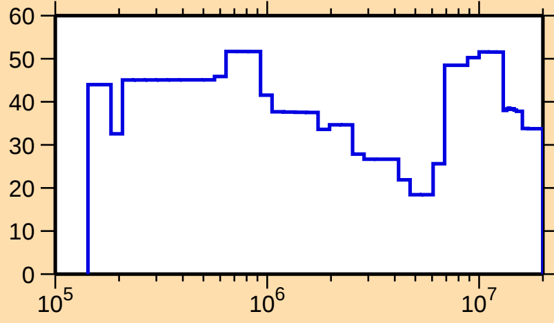
\Delta\sigma/\sigma vs. E for ^{169}\text{W}(\text{n,el.})
