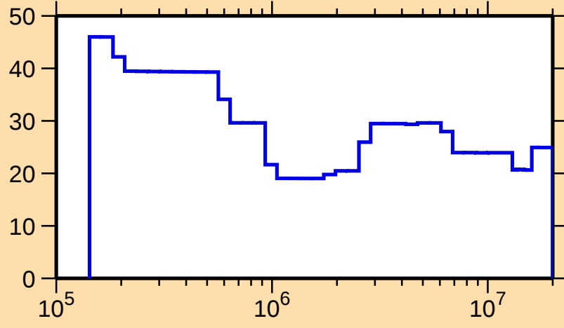
\Delta\sigma/\sigma vs. E for ^{169}\text{W}(n,\text{nonel.})
