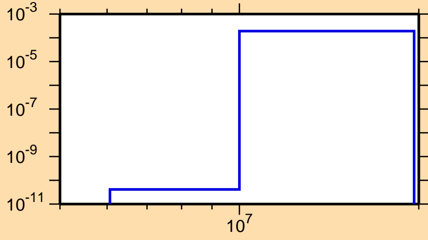
\sigma vs. E for ^{169}\text{W}(n,t)
