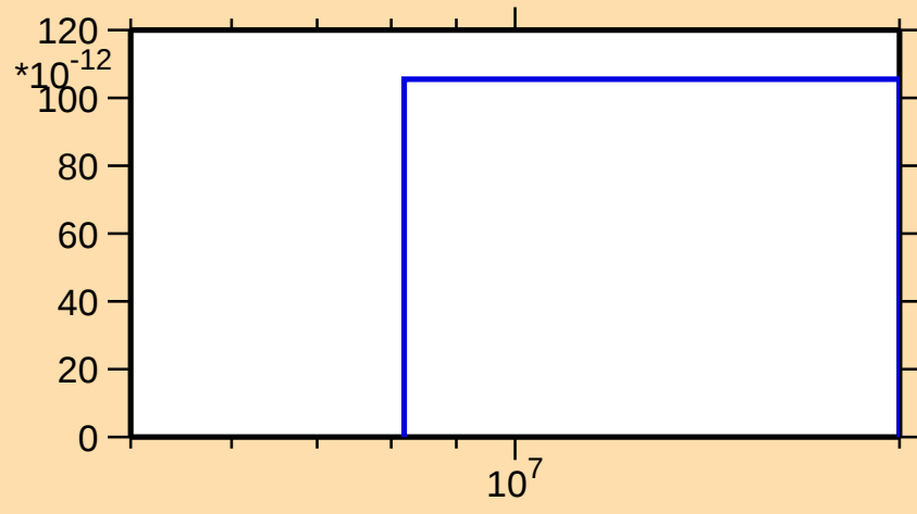
\sigma vs. E for ^{169}\text{W}(\text{mt117})
