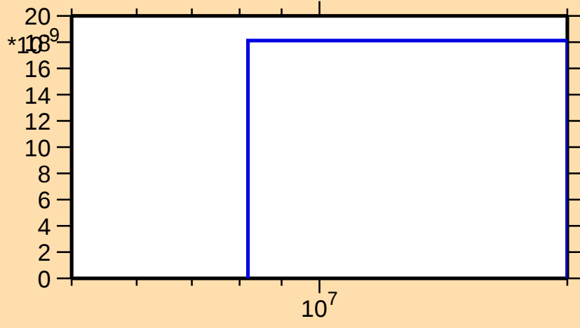
\sigma vs. E for ^{169}\text{W}(n,\text{pd})
