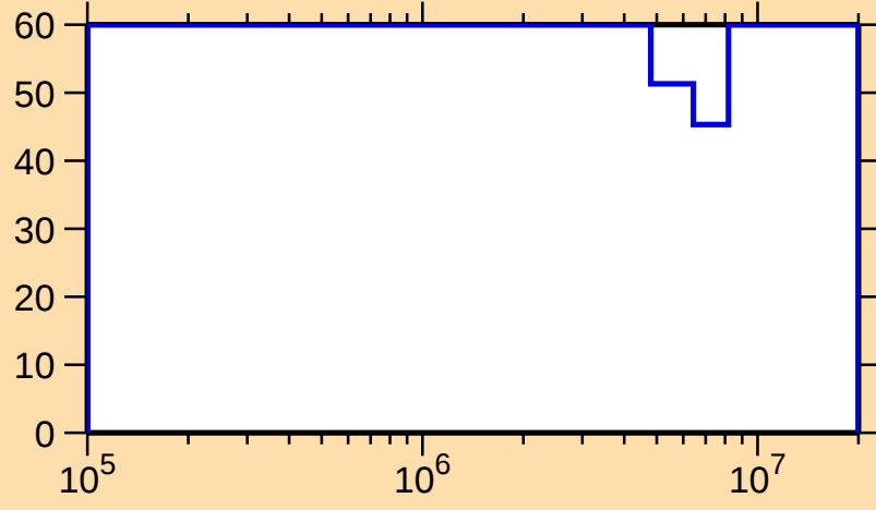
\Delta\sigma/\sigma vs. E for ^{169}\text{W}(\text{n},\text{inel.})
