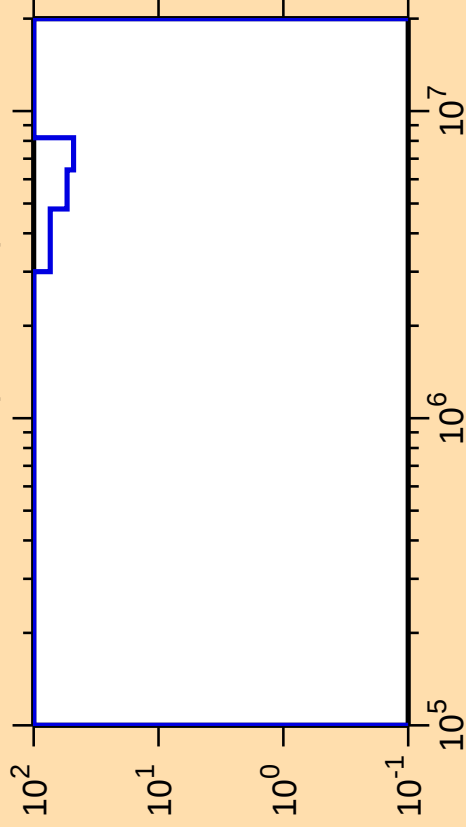
\Delta\sigma/\sigma vs. E for ^{169}\text{W}(\text{n},\text{ncont.})
