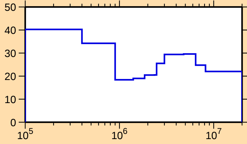
\Delta\sigma/\sigma vs. E for ^{169}\text{W}(\text{n},\text{nonel.})
