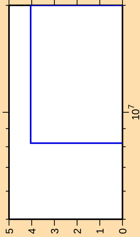
\Delta\sigma/\sigma vs. E for ^{169}\text{W}(n,nt)
