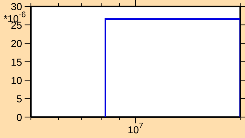
\sigma vs. E for ^{169}\text{W}(n,2n\alpha)
