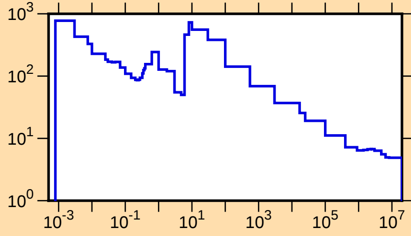
\sigma vs. E for ^{169}\text{W}(n,\text{tot.})
