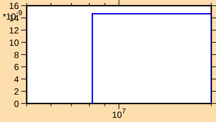
\sigma vs. E for ^{169}\text{W}(\text{mt 45})
