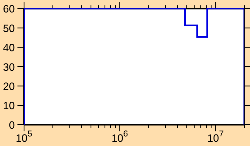
\Delta\sigma/\sigma vs. E for ^{169}\text{W}(n,\text{inel.})
