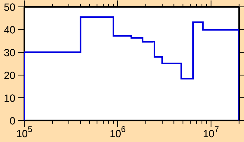
\Delta\sigma/\sigma vs. E for ^{169}\text{W}(n,\text{el.})
