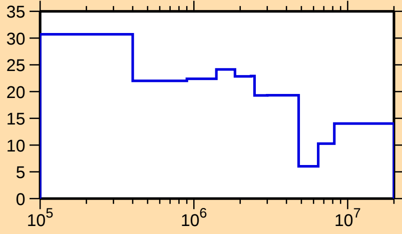
\Delta\sigma/\sigma vs. E for ^{169}\text{W}(n,\text{tot.})
