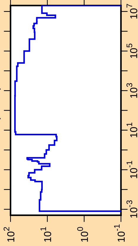
\Delta\sigma/\sigma vs. E for ^{169}\text{W}(n,\text{tot.})
