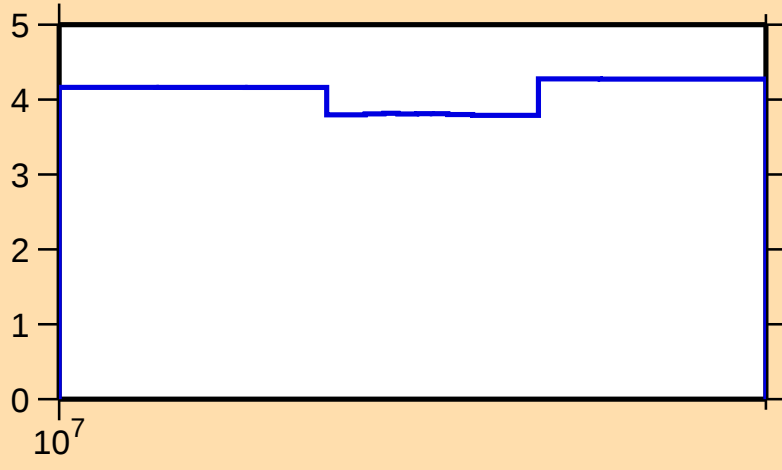
\Delta\sigma/\sigma vs. E for ^{170}\text{W}(n,\text{tot.})
