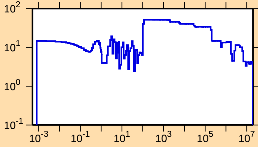
\Delta\sigma/\sigma vs. E for ^{170}\text{W}(\text{n,tot.})
