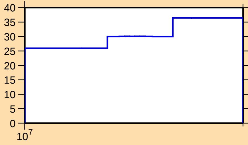
\Delta\sigma/\sigma vs. E for ^{170}\text{W}(n,\text{inel.})
