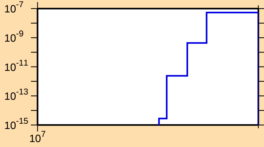
\sigma vs. E for ^{170}\text{W}(n,\text{nd})
