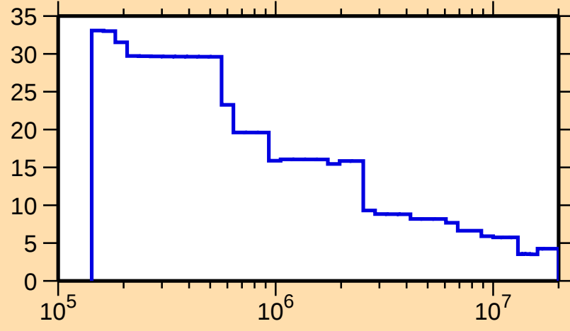
\Delta\sigma/\sigma vs. E for ^{170}\text{W}(\text{n,nonel.})
