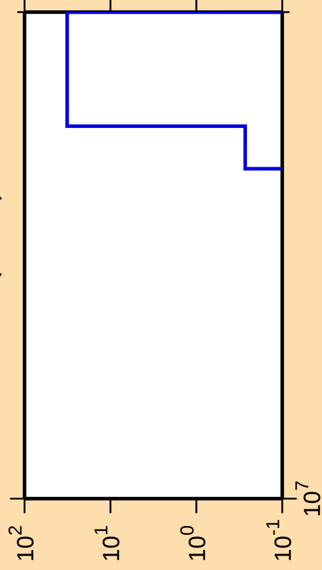
\Delta\sigma/\sigma vs. E for ^{170}\text{W} (mt 34)
