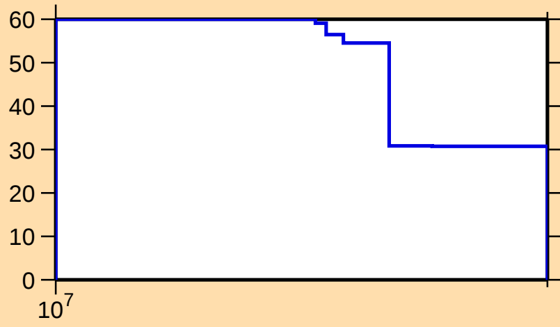
\Delta\sigma/\sigma vs. E for ^{170}\text{W}(n,2n)
