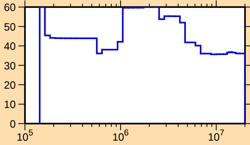
\Delta\sigma/\sigma vs. E for ^{170}\text{W}(n,n_1)
