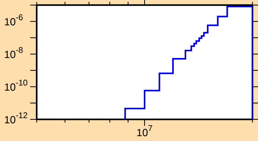
\sigma vs. E for ^{170}\text{W}(n,\text{He3})
