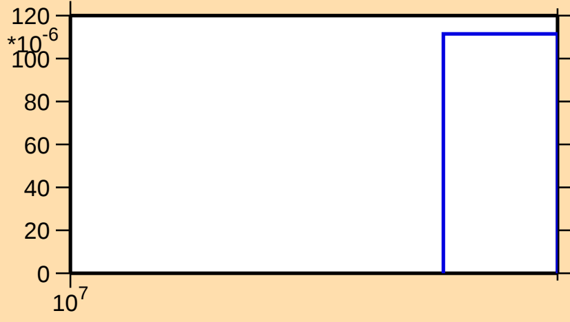
\sigma vs. E for ^{170}\text{W}(n,3n)
