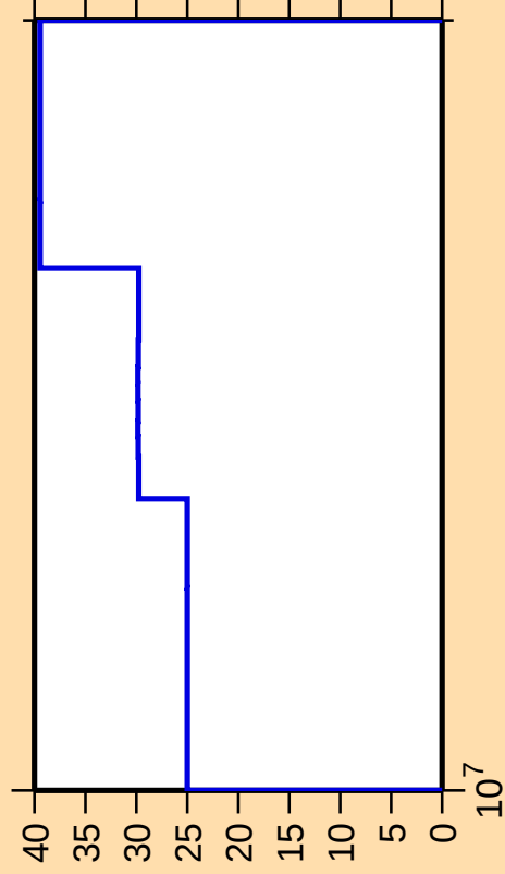
\Delta\sigma/\sigma vs. E for ^{170}\text{W}(n,n\text{cont.})
