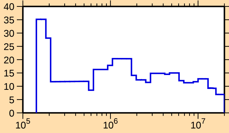
\Delta\sigma/\sigma vs. E for ^{170}\text{W}(n,\text{el.})
