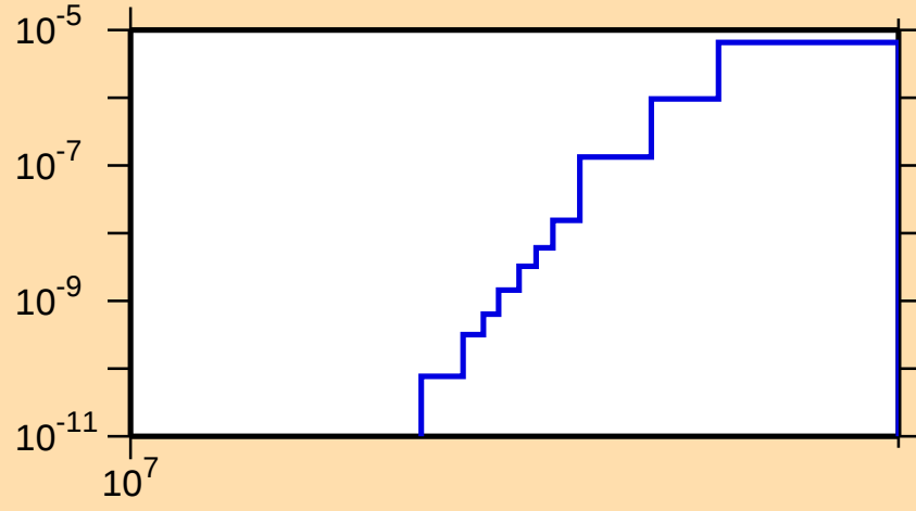
\sigma vs. E for ^{170}\text{W}(n,2n\alpha)
