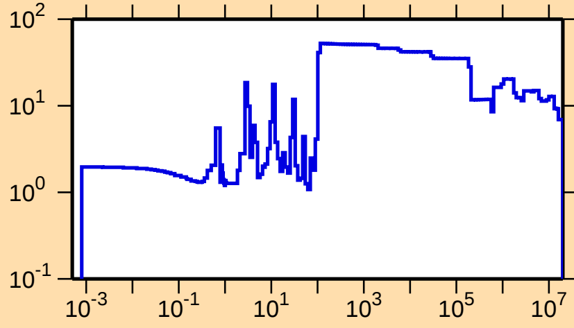
\Delta\sigma/\sigma vs. E for ^{170}\text{W}(\text{n,el.})
