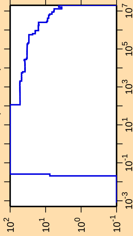
\Delta\sigma/\sigma vs. E for ^{170}\text{W}(n,\text{nonel.})
