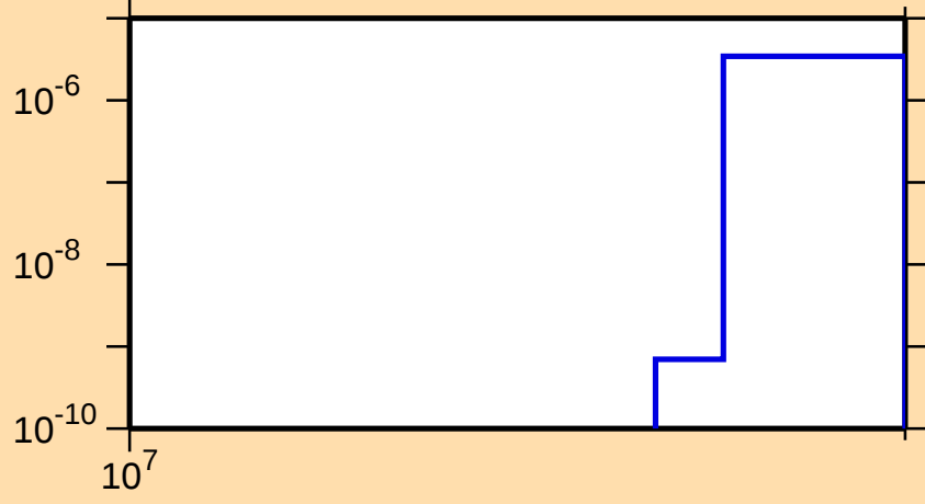
\sigma vs. E for ^{170}\text{W}(n,2np)
