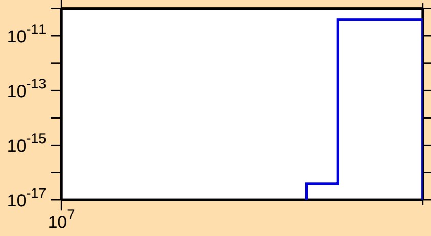
\sigma vs. E for ^{170}\text{W}(n,nt)
