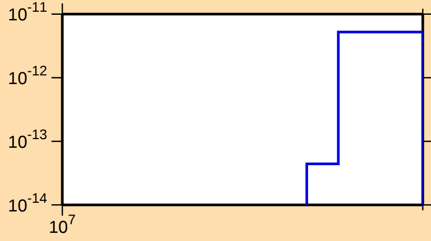
\sigma vs. E for ^{170}\text{W} (mt 34)
