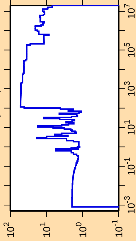
\Delta\sigma/\sigma vs. E for ^{170}\text{W}(\text{n,el.})
