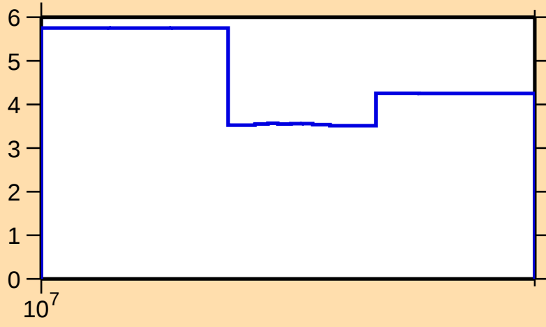
\Delta\sigma/\sigma vs. E for ^{170}\text{W}(n,\text{nonel.})
