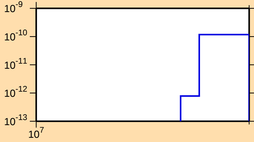
\sigma vs. E for ^{170}\text{W}(n,\text{pt})
