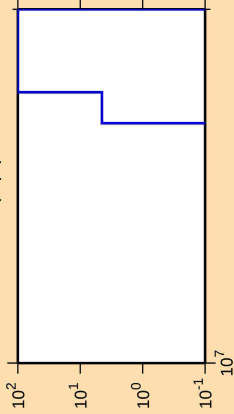
\Delta\sigma/\sigma vs. E for ^{170}\text{W}(n,\text{pt})
