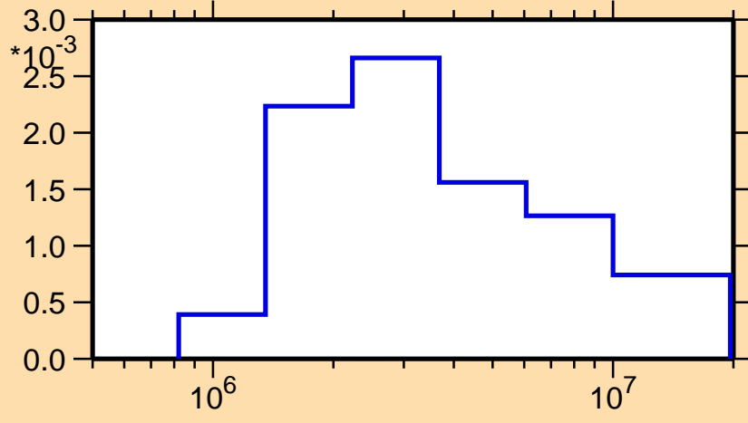
\sigma vs. E for ^{170}\text{W}(n,n_3)
