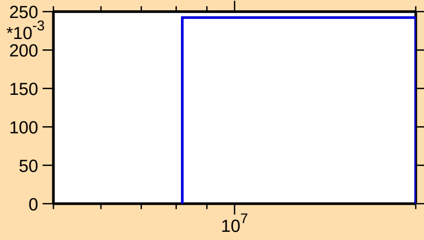
\sigma vs. E for ^{170}\text{W}(n,2n)
