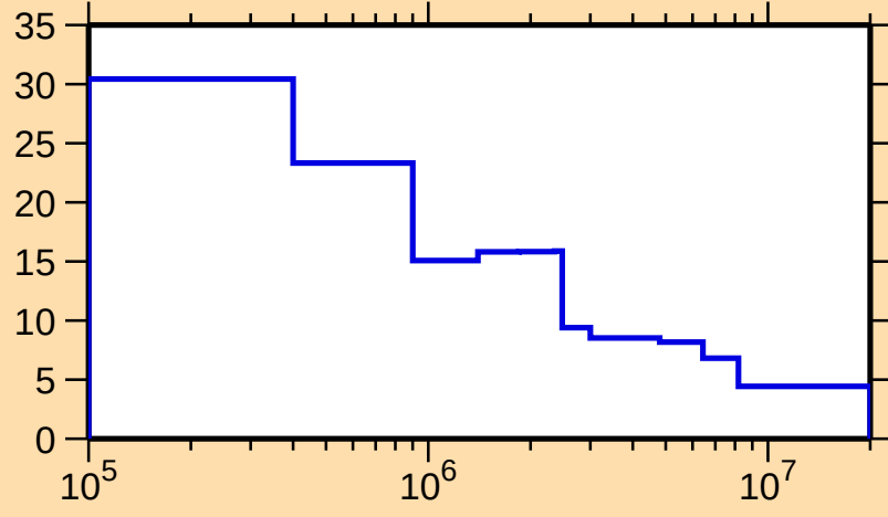
\Delta\sigma/\sigma vs. E for ^{170}\text{W}(n,\text{nonel.})
