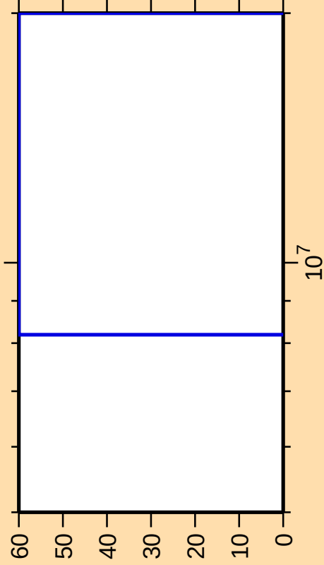
\Delta\sigma/\sigma vs. E for ^{170}\text{W}(\text{n},\text{nd})
