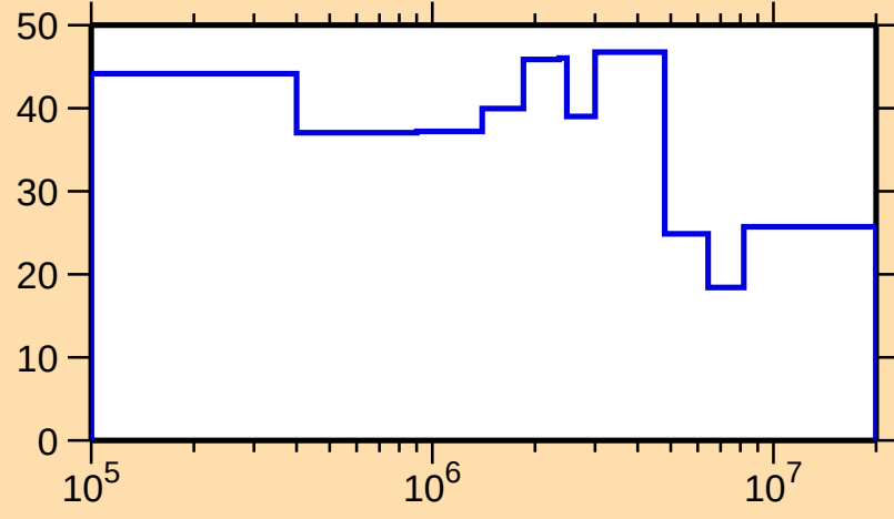
\Delta\sigma/\sigma vs. E for ^{170}\text{W}(\text{n,inel.})
