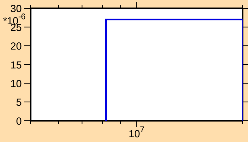
\sigma vs. E for ^{170}\text{W}(n,t)
