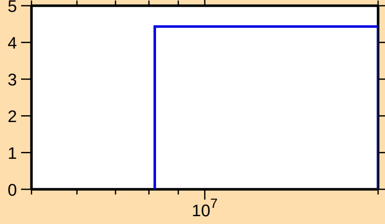
\Delta\sigma/\sigma vs. E for ^{170}\text{W}(n,\text{nonel.})
