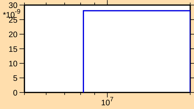
\sigma vs. E for ^{170}\text{W}(n,2np)
