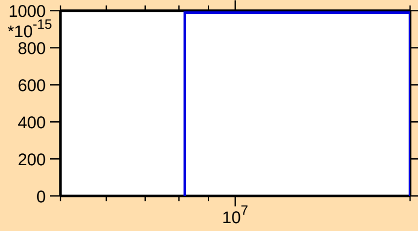
\sigma vs. E for ^{170}\text{W}(\text{n},\text{pt})
