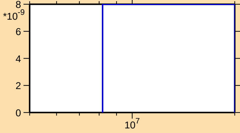
\sigma vs. E for ^{170}\text{W}(n,\text{pd})
