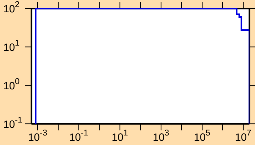
\Delta\sigma/\sigma vs. E for ^{170}\text{W}(n,p)
