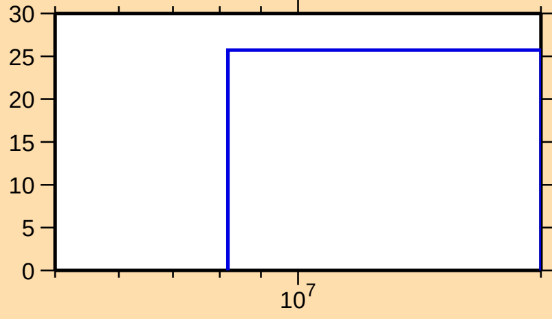
\Delta\sigma/\sigma vs. E for ^{170}\text{W}(n,\text{inel.})
