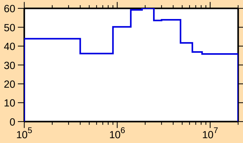
\Delta\sigma/\sigma vs. E for ^{170}\text{W}(n,n_1)
