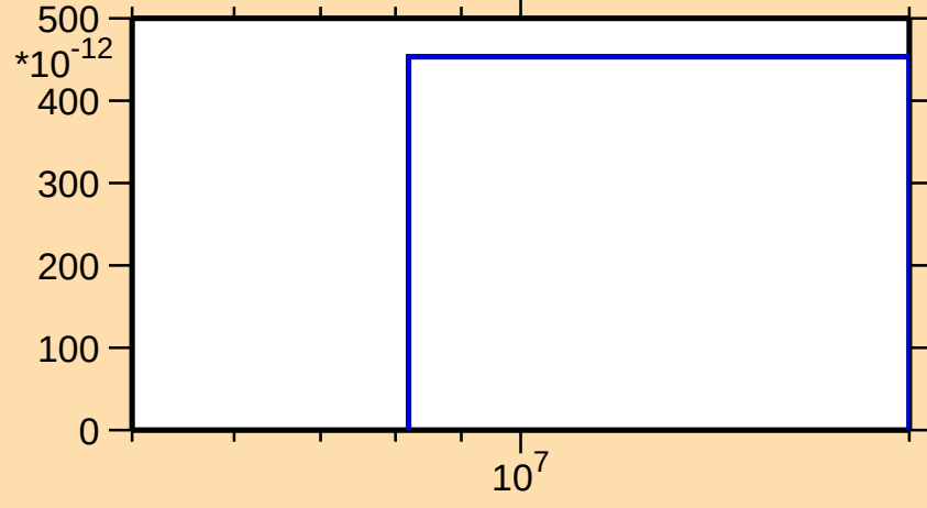
\sigma vs. E for ^{170}\text{W}(\text{n},\text{nd})
