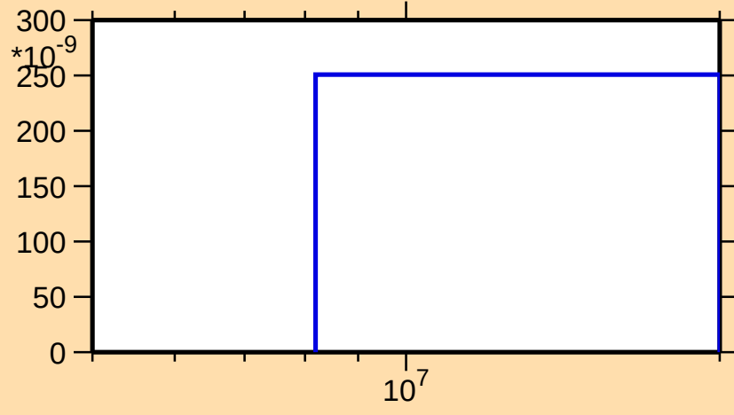
\sigma vs. E for ^{170}\text{W}(n,\text{He3})
