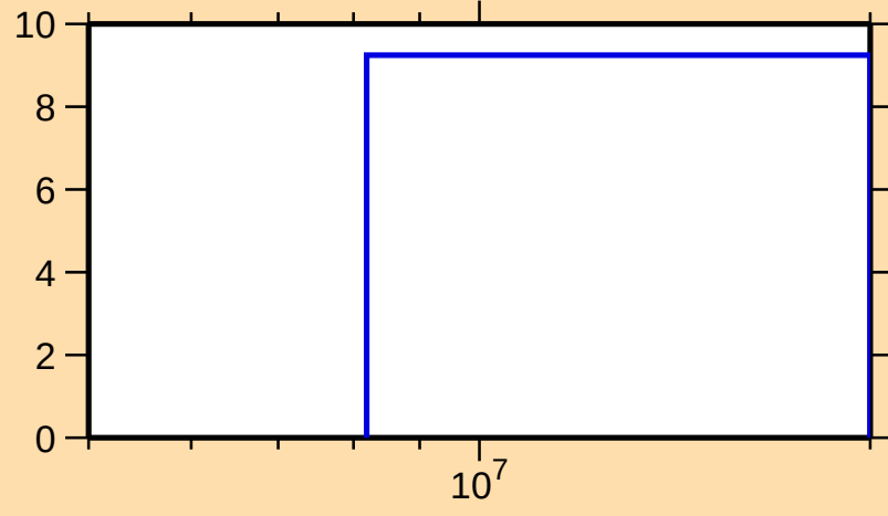
\Delta\sigma/\sigma vs. E for ^{170}\text{W}(n,\text{el.})
