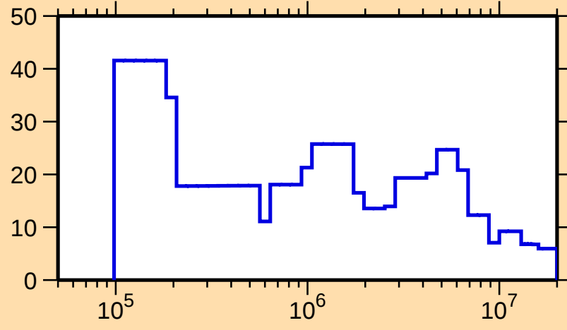
\Delta\sigma/\sigma vs. E for ^{171}\text{W}(\text{n,el.})
