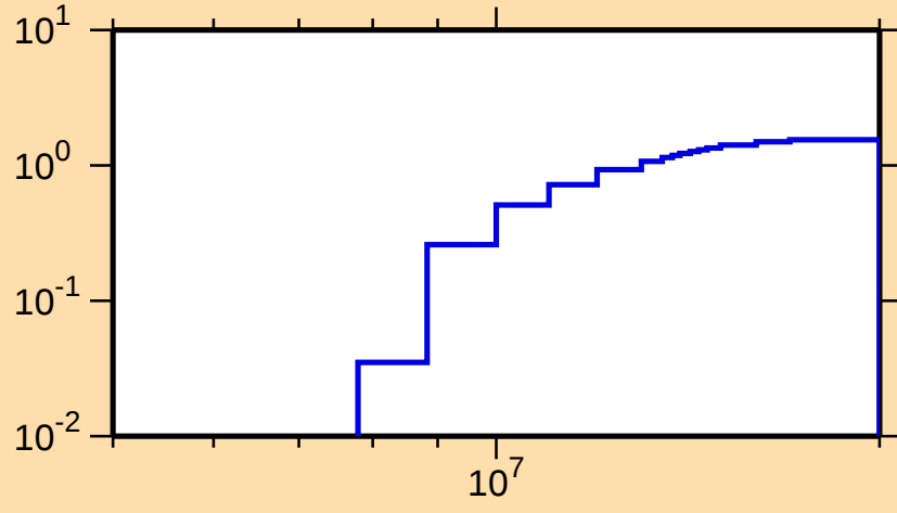
\sigma vs. E for ^{171}\text{W}(n,2n)
