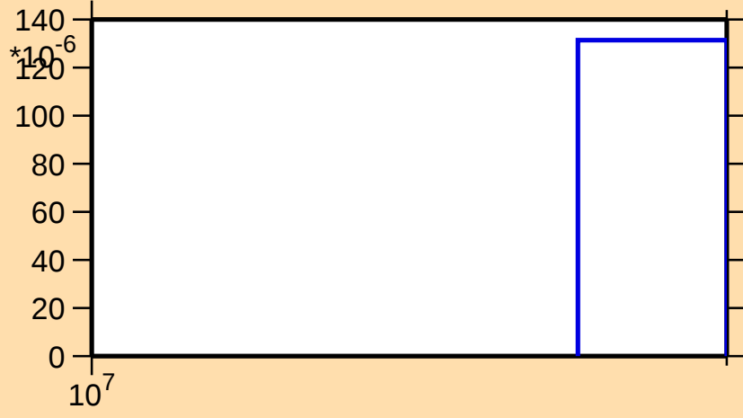
\sigma vs. E for ^{171}\text{W}(n,3n)
