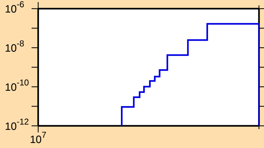
\sigma vs. E for ^{171}\text{W}(\text{n},\text{pd})
