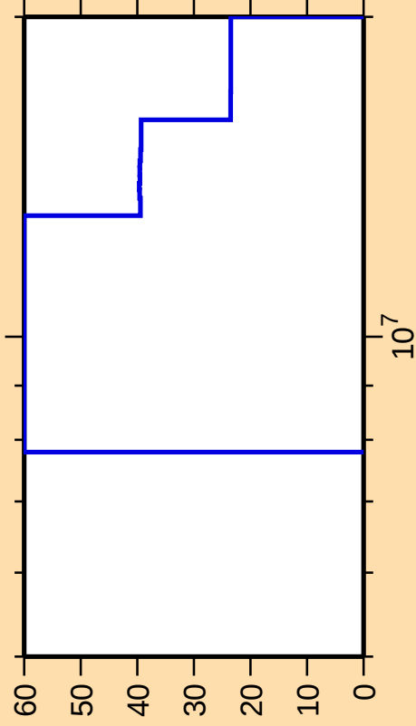
\Delta\sigma/\sigma vs. E for ^{171}\text{W}(n,2n)
