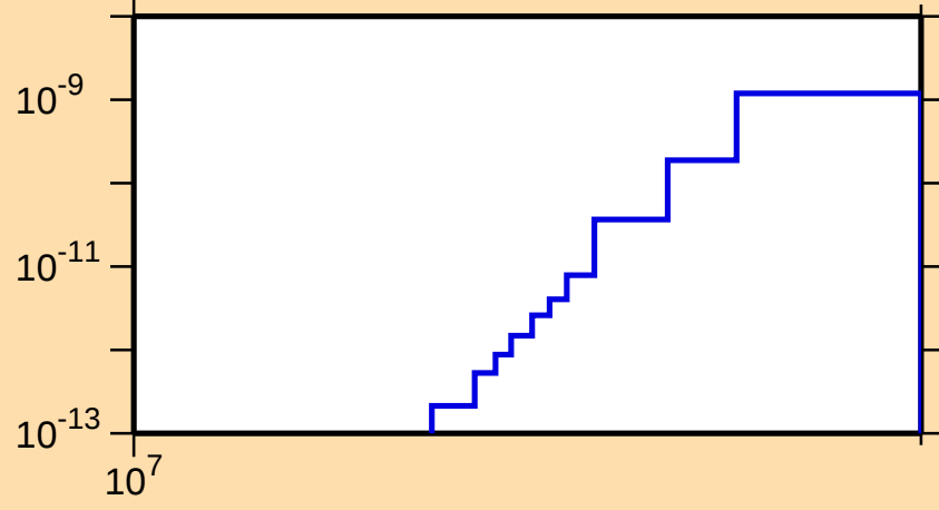
\sigma vs. E for ^{171}\text{W}(\text{mt117})
