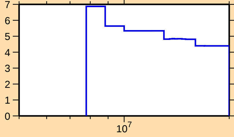
\Delta\sigma/\sigma vs. E for ^{171}\text{W}(n,\text{nonel.})
