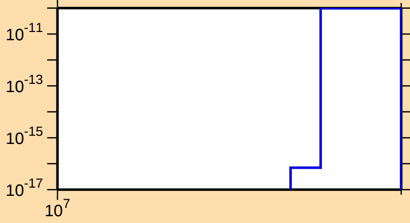
\sigma vs. E for ^{171}\text{W}(n,nt)
