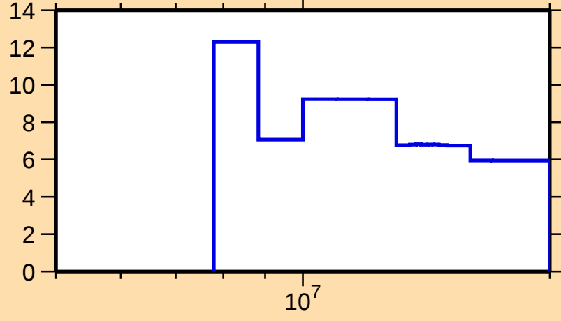
\Delta\sigma/\sigma vs. E for ^{171}\text{W}(n,\text{el.})
