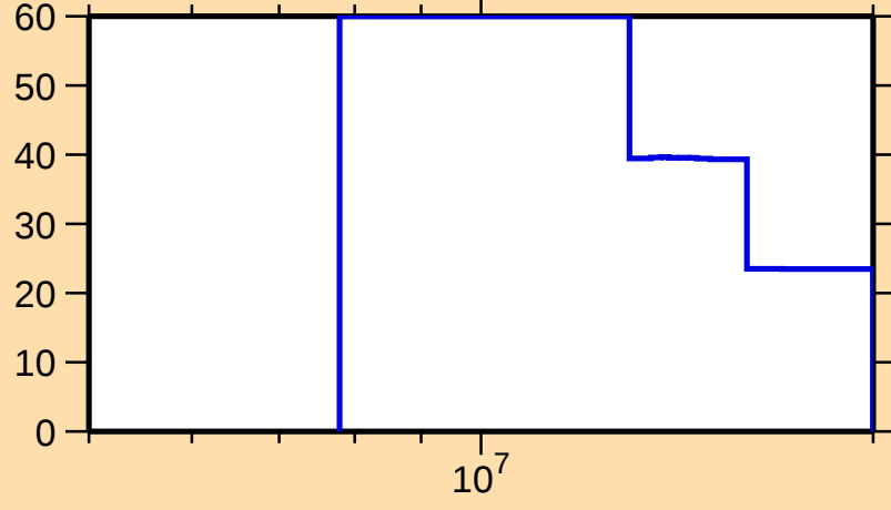
\Delta\sigma/\sigma vs. E for ^{171}\text{W}(n,2n)
