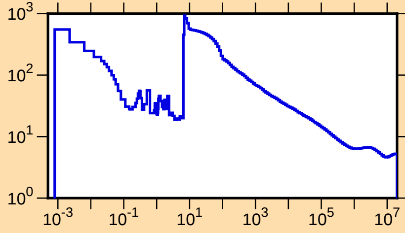
\sigma vs. E for ^{171}\text{W}(n,\text{tot.})
