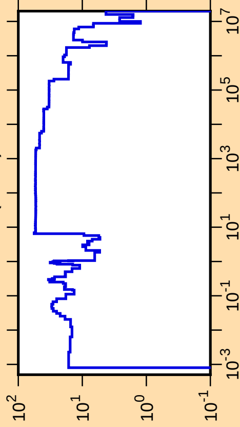
\Delta\sigma/\sigma vs. E for ^{171}\text{W}(n,\text{tot.})
