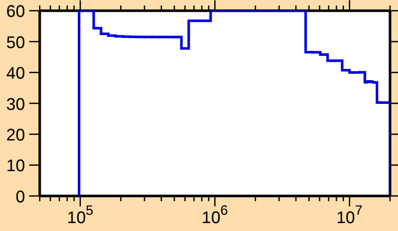
\Delta\sigma/\sigma vs. E for ^{171}\text{W}(n,n_1)
