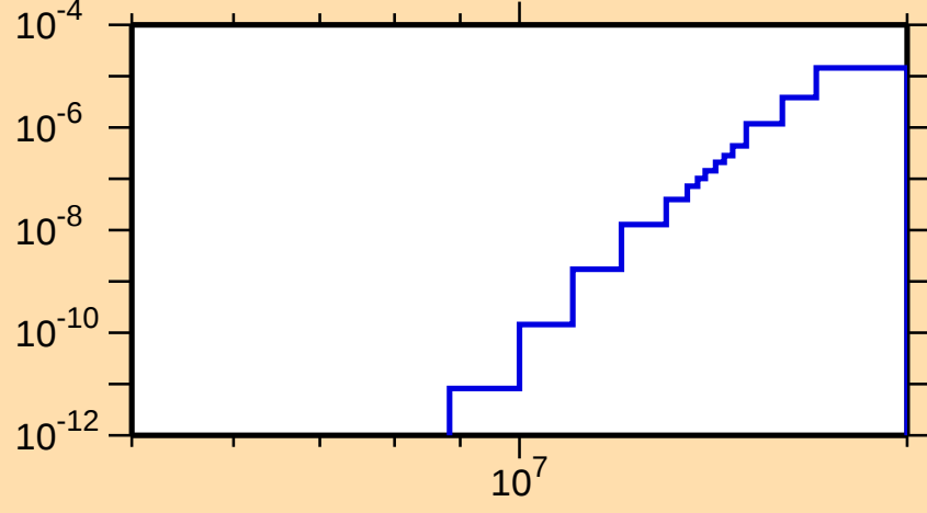
\sigma vs. E for ^{171}\text{W}(n,\text{He3})
