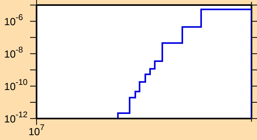
\sigma vs. E for ^{171}\text{W}(n,\text{nd})
