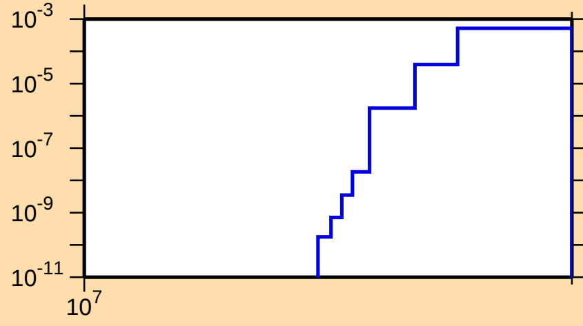
\sigma vs. E for ^{171}\text{W}(n,2np)
