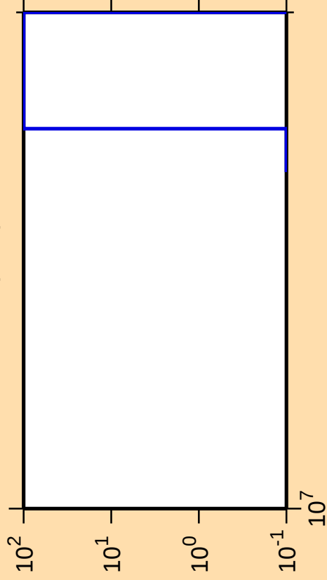
\Delta\sigma/\sigma vs. E for ^{171}\text{W}(n,nt)
