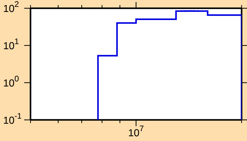
\Delta\sigma/\sigma vs. E for ^{171}\text{W}(n,\text{inel.})
