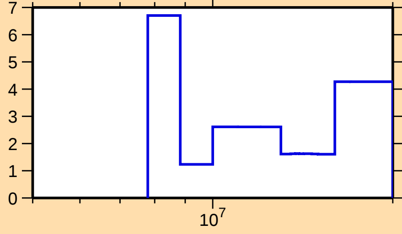
\Delta\sigma/\sigma vs. E for ^{171}\text{W}(n,\text{tot.})
