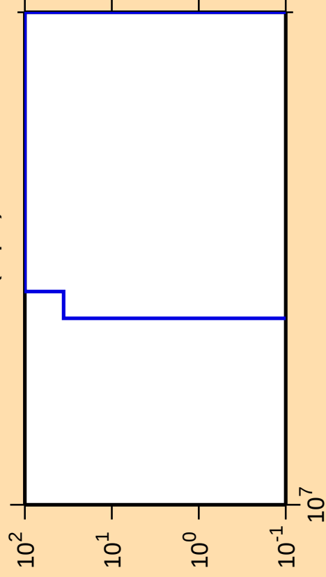
\Delta\sigma/\sigma vs. E for ^{171}\text{W}(\text{n},\text{pd})
