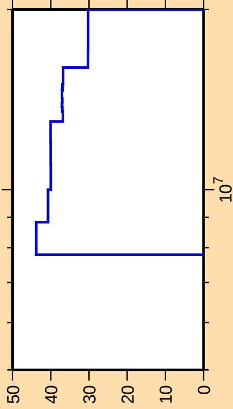
\Delta\sigma/\sigma vs. E for ^{171}\text{W}(n,n_1)
