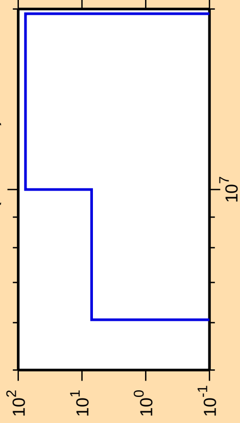
\Delta\sigma/\sigma vs. E for ^{171}\text{W}(n,n\text{cont.})
