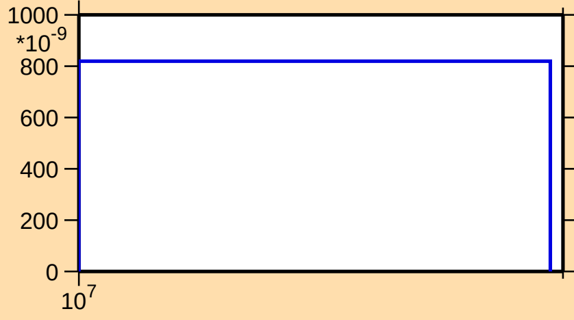
\sigma vs. E for ^{171}\text{W}(n,3n)
