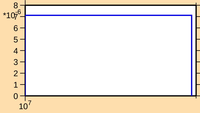
\sigma vs. E for ^{171}\text{W}(n,2np)
