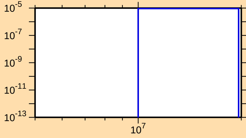
\sigma vs. E for ^{171}\text{W}(n,2n\alpha)
