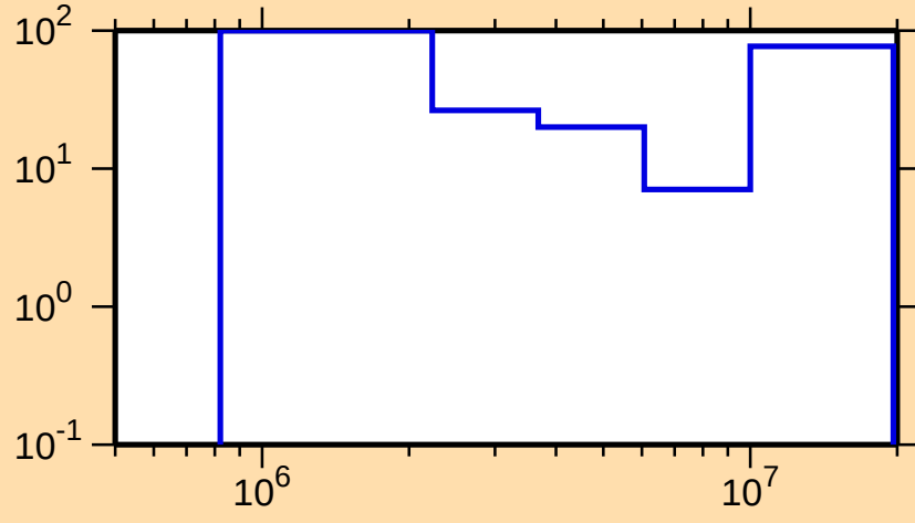
\Delta\sigma/\sigma vs. E for ^{171}\text{W}(n,ncont.)
