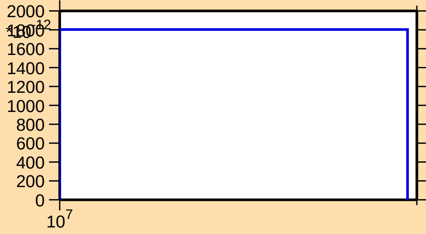
\sigma vs. E for ^{171}\text{W}(\text{mt 45})
