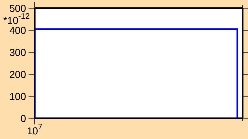
\sigma vs. E for ^{171}\text{W}(\text{n},\text{pt})
