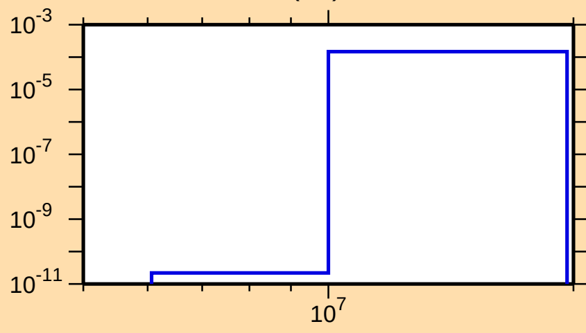
\sigma vs. E for ^{171}\text{W}(n,t)
