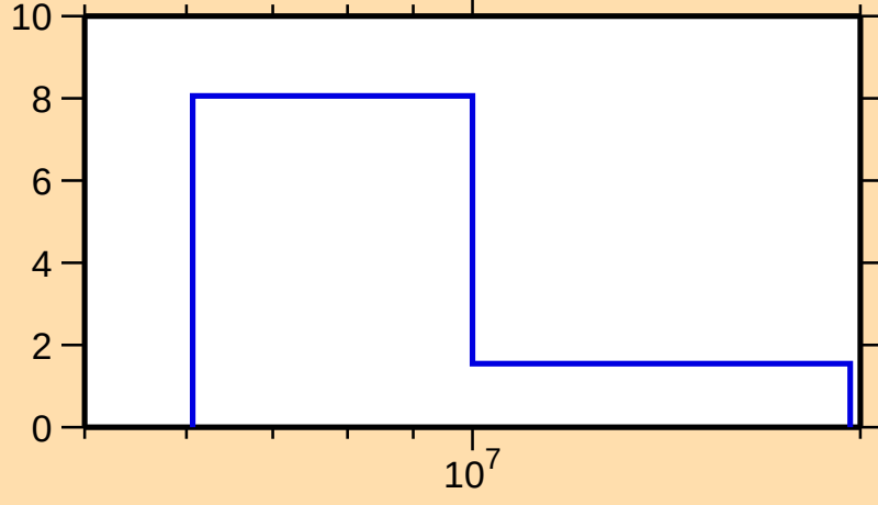
\Delta\sigma/\sigma vs. E for ^{171}\text{W}(n,\text{tot.})
