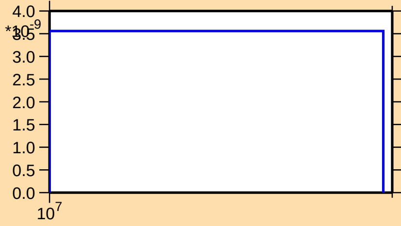
\sigma vs. E for ^{171}\text{W}(\text{n},\text{pd})
