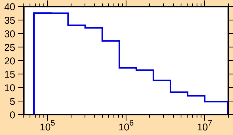
\Delta\sigma/\sigma vs. E for ^{171}\text{W}(\text{n,nonel.})
