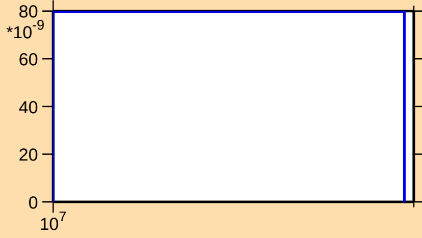
\sigma vs. E for ^{171}\text{W}(n,\text{nd})
