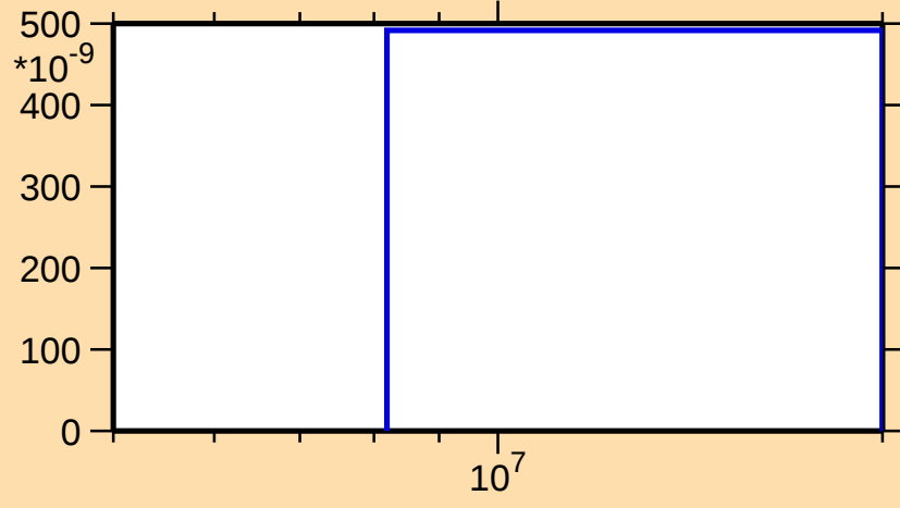
\sigma vs. E for ^{171}\text{W}(n,\text{He3})
