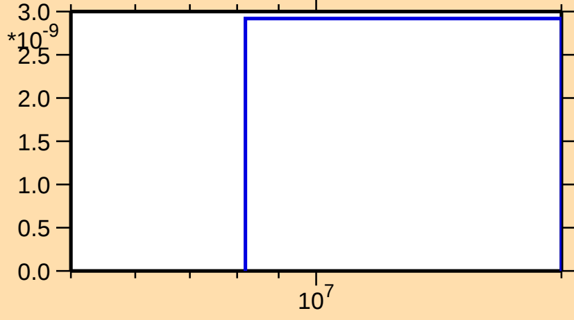
\sigma vs. E for ^{171}\text{W}(n,\text{pd})
