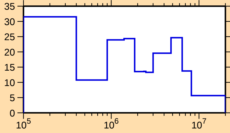
\Delta\sigma/\sigma vs. E for ^{171}\text{W}(\text{n,el.})
