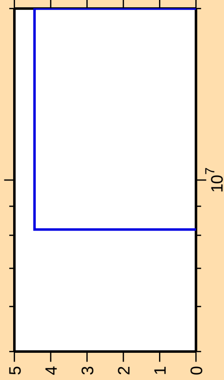
\Delta\sigma/\sigma vs. E for ^{171}\text{W}(n,nt)
