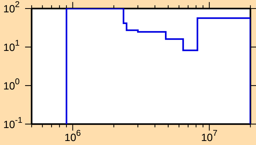
\Delta\sigma/\sigma vs. E for ^{171}\text{W}(n,n\text{cont.})
