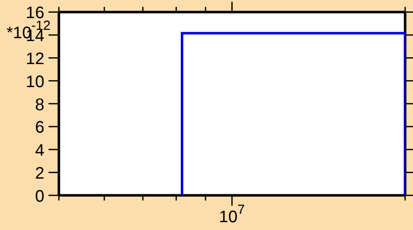
\sigma vs. E for ^{171}\text{W}(\text{mt } 34)
