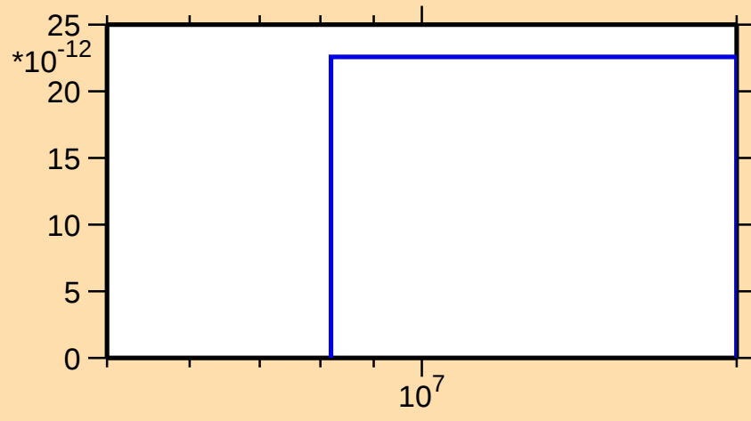
\sigma vs. E for ^{171}\text{W}(\text{mt117})
