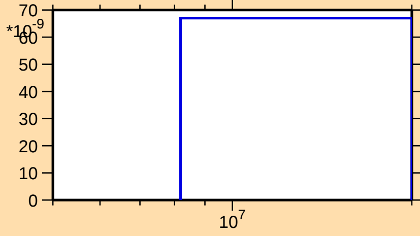
\sigma vs. E for ^{171}\text{W}(\text{n},\text{nd})
