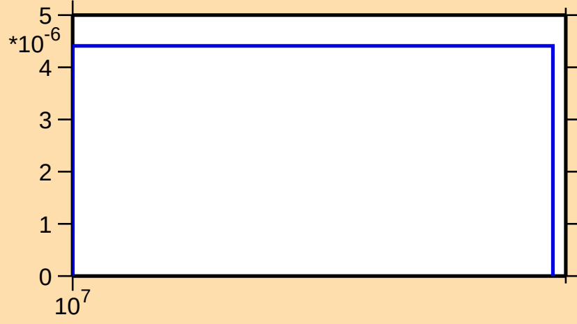
\sigma vs. E for ^{172}\text{W}(n,3n)
