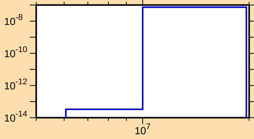
\sigma vs. E for ^{172}\text{W}(n,\text{He3})
