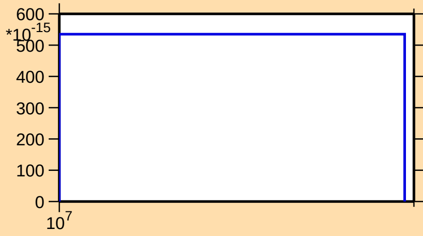
\sigma vs. E for ^{172}\text{W}(n,nt)
