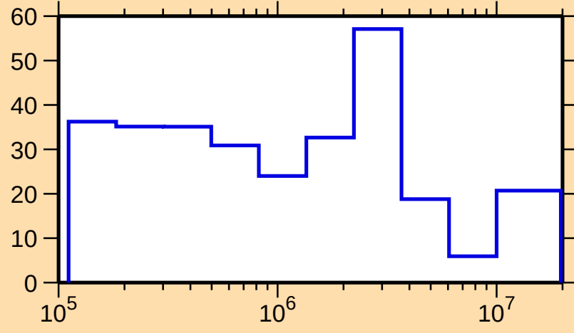
\Delta\sigma/\sigma vs. E for ^{172}\text{W}(\text{n,inel.})
