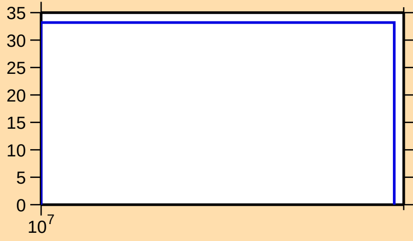
\Delta\sigma/\sigma vs. E for ^{172}\text{W}(n,2n)
