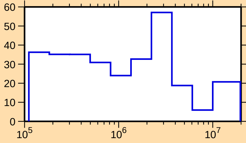
\Delta\sigma/\sigma vs. E for ^{172}\text{W}(n,\text{inel.})
