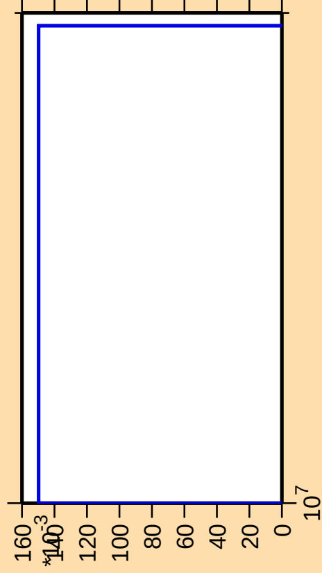
\Delta\sigma/\sigma vs. E for ^{172}\text{W}(\text{mt } 34)
