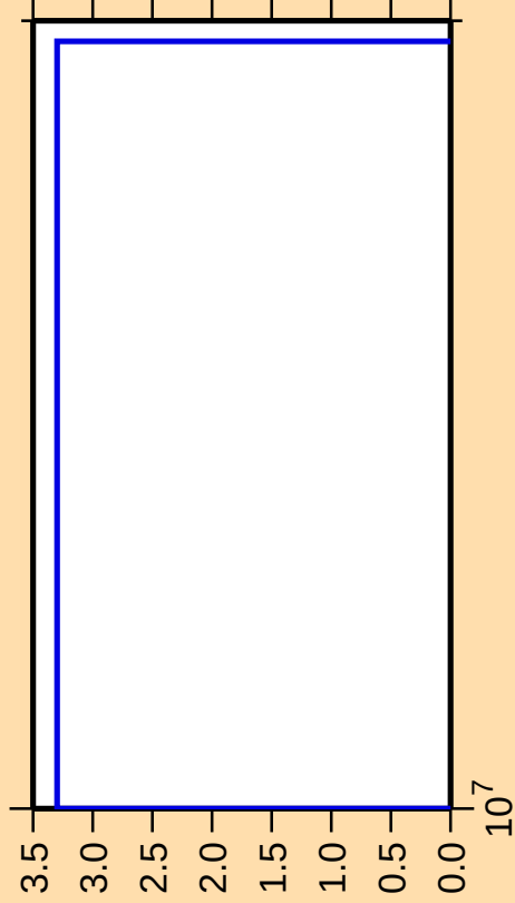
\Delta\sigma/\sigma vs. E for ^{172}\text{W}(n,nt)
