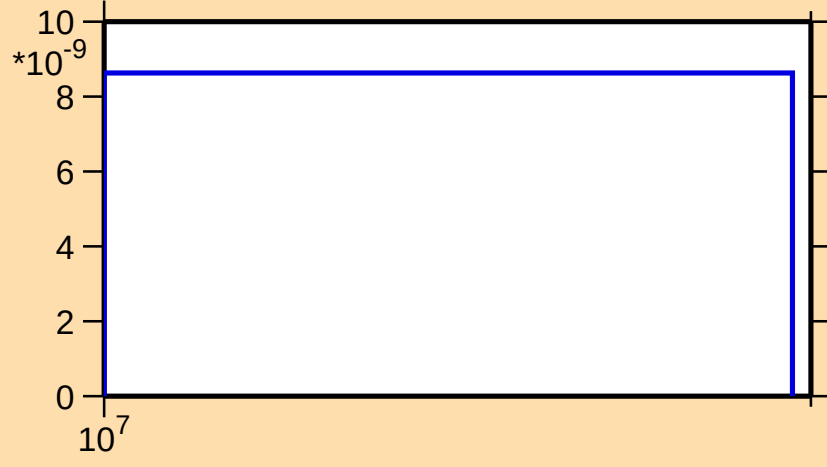
\sigma vs. E for ^{172}\text{W}(n,2np)
