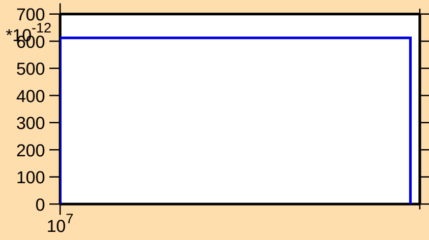
\sigma vs. E for ^{172}\text{W}(\text{n},\text{pd})
