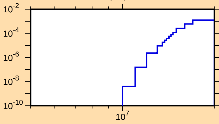
\sigma vs. E for ^{173}\text{W}(n,t)
