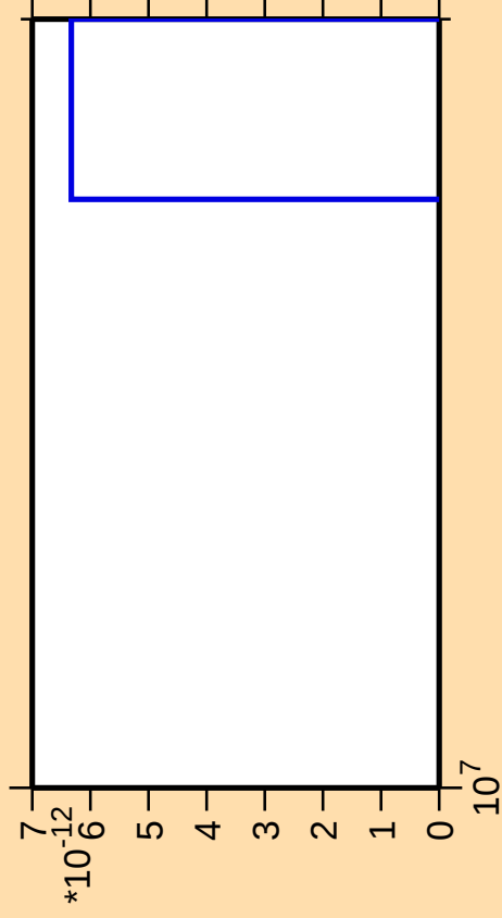
\Delta\sigma/\sigma vs. E for ^{173}\text{W} (mt 11)
