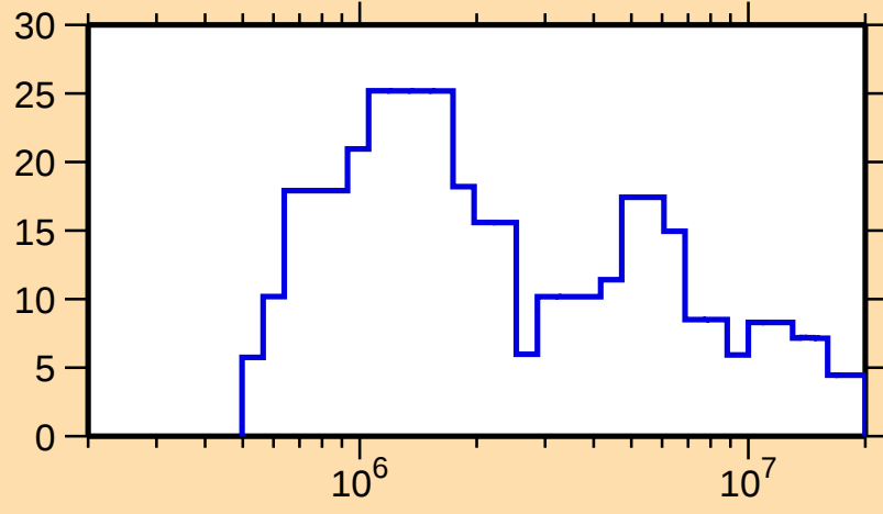
\Delta\sigma/\sigma vs. E for ^{173}\text{W}(\text{n},\text{el.})
