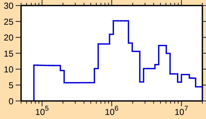
\Delta\sigma/\sigma vs. E for ^{173}\text{W}(\text{n,el.})
