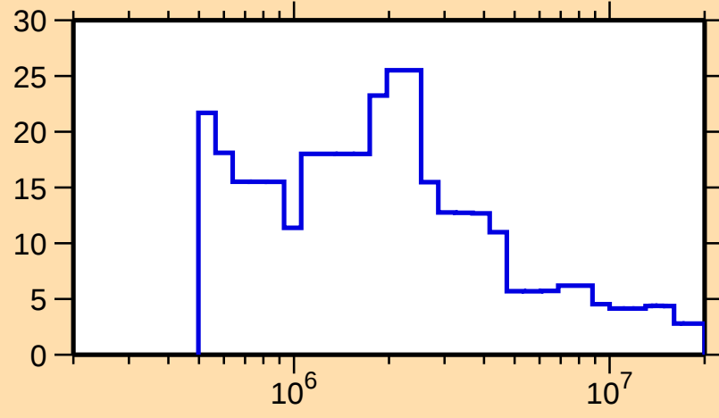
\Delta\sigma/\sigma vs. E for ^{173}\text{W}(\text{n},\text{nonel.})
