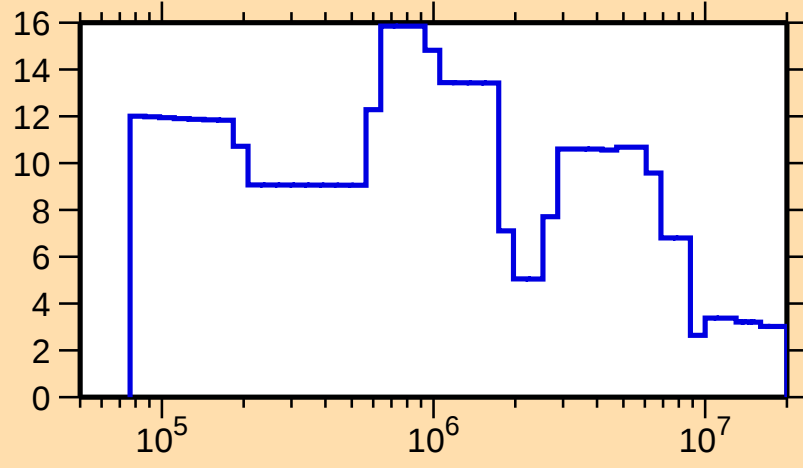
\Delta\sigma/\sigma vs. E for ^{173}\text{W}(\text{n,tot.})
