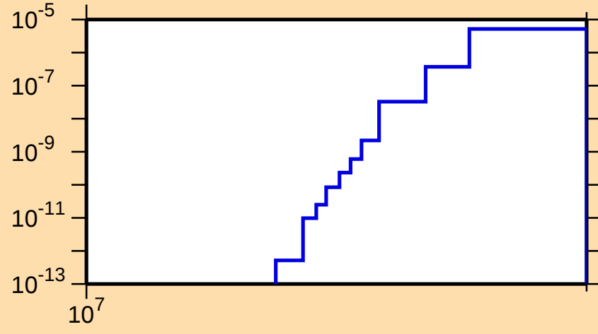
\sigma vs. E for ^{173}\text{W}(n,\text{nd})
