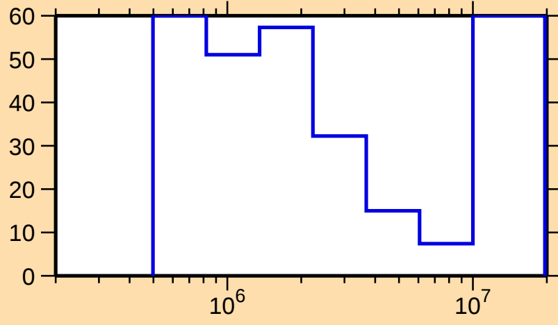
\Delta\sigma/\sigma vs. E for ^{173}\text{W}(\text{n},\text{inel.})
