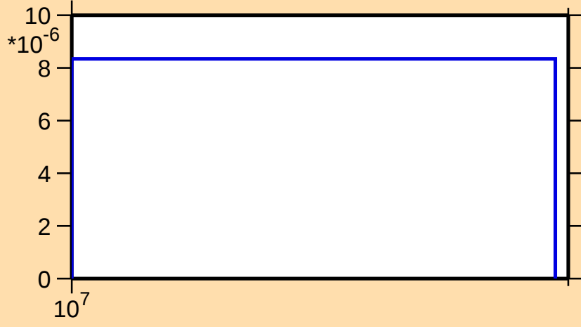
\sigma vs. E for ^{173}\text{W}(n,3n)
