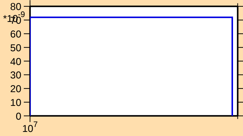
\sigma vs. E for ^{173}\text{W}(\text{n},\text{nd})
