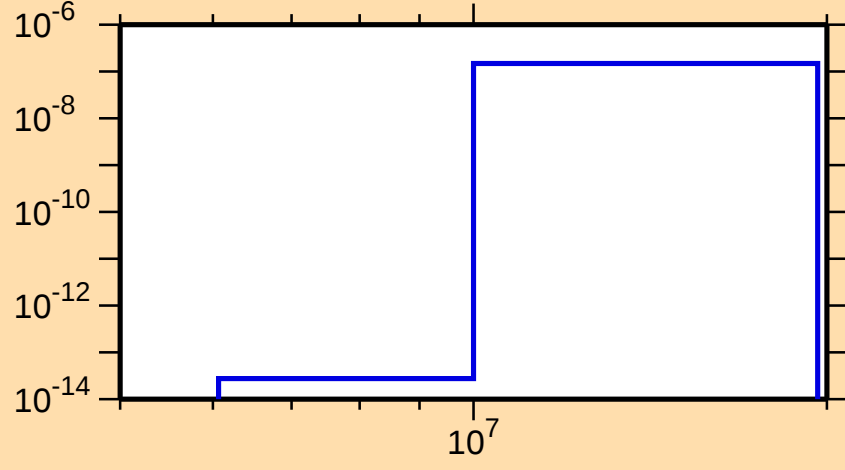
\sigma vs. E for ^{173}\text{W}(n,\text{He3})
