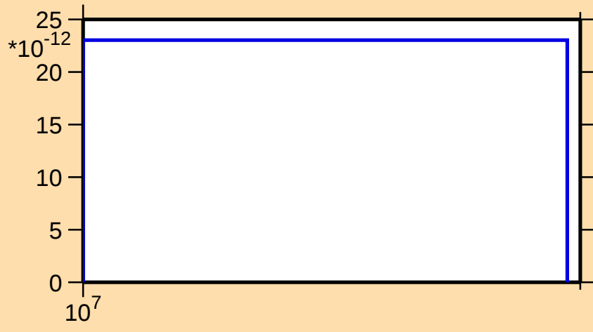
\sigma vs. E for ^{173}\text{W}(\text{n},\text{pt})
