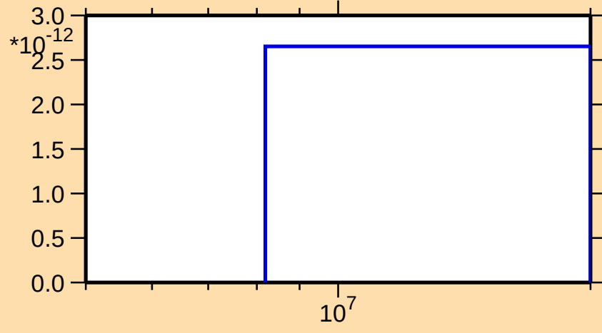
\sigma vs. E for ^{173}\text{W}(\text{mt } 34)
