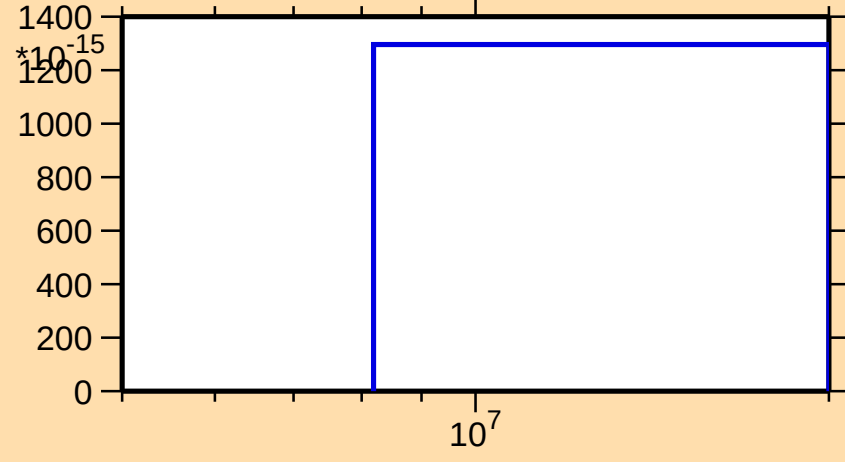
\sigma vs. E for ^{173}\text{W}(n,nt)
