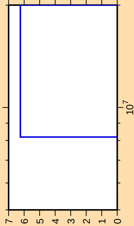
\Delta\sigma/\sigma vs. E for ^{173}\text{W}(n,nt)
