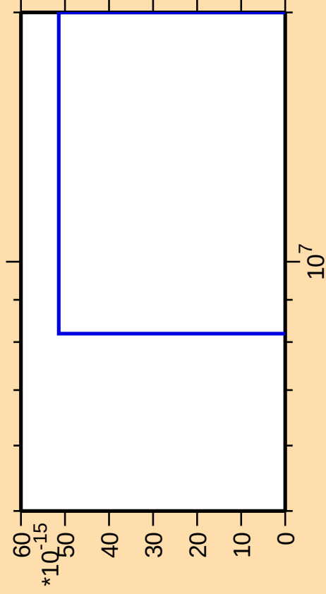
\Delta\sigma/\sigma vs. E for ^{173}\text{W}(\text{mt 11})
