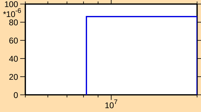
\sigma vs. E for ^{173}\text{W}(n,t)
