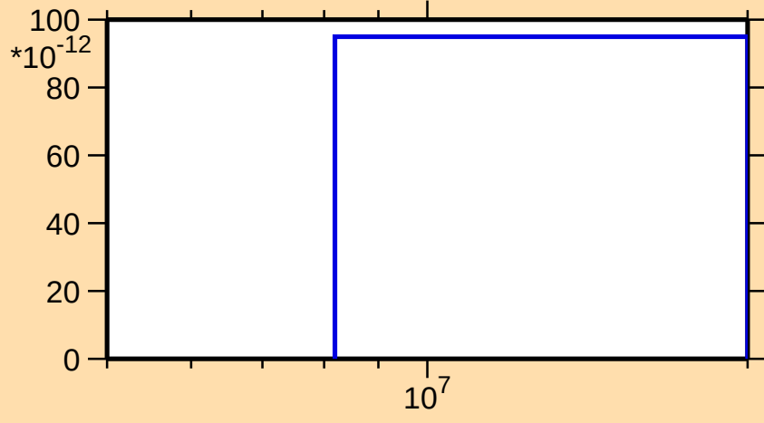
\sigma vs. E for ^{173}\text{W}(\text{mt 45})
