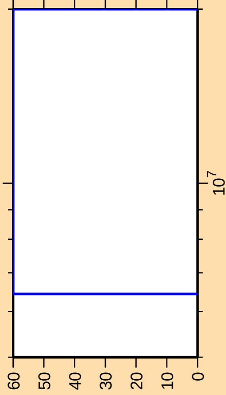
\Delta\sigma/\sigma vs. E for ^{173}\text{W}(n,np)
