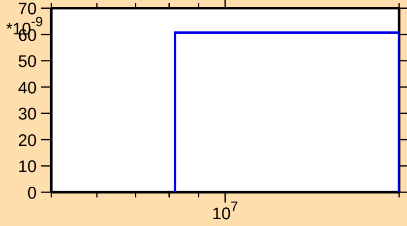
\sigma vs. E for ^{173}\text{W}(\text{n},\text{nd})
