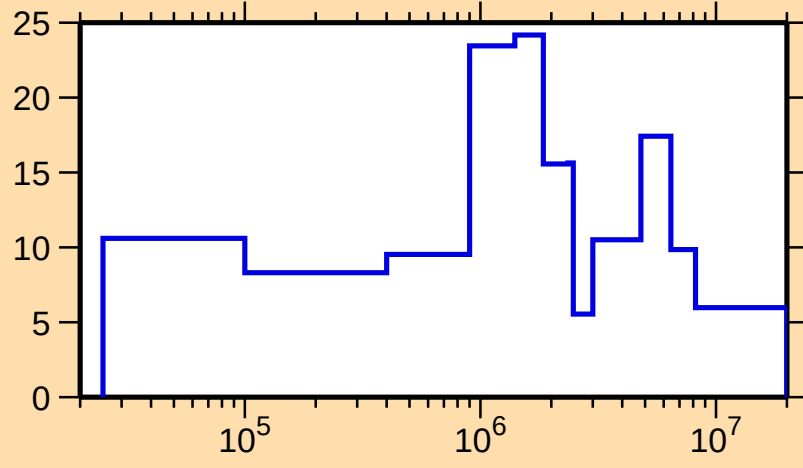
\Delta\sigma/\sigma vs. E for ^{173}\text{W}(\text{n,el.})
