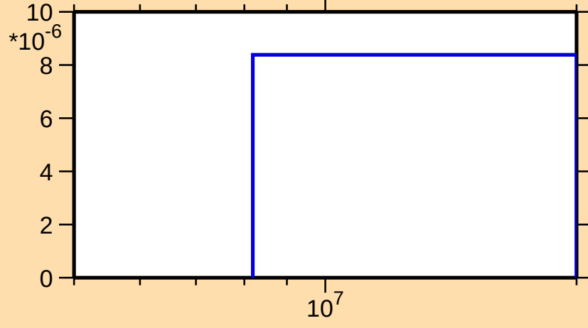
\sigma vs. E for ^{173}\text{W}(n,3n)
