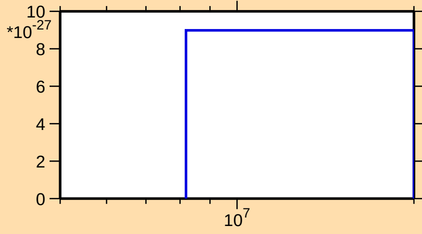
\sigma vs. E for ^{173}\text{W}(\text{mt 11})
