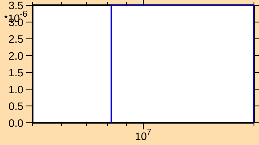
\sigma vs. E for ^{173}\text{W}(n,2n\alpha)
