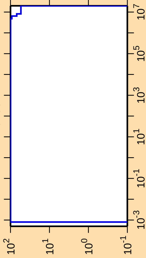
\Delta\sigma/\sigma vs. E for ^{173}\text{W}(n,p)
