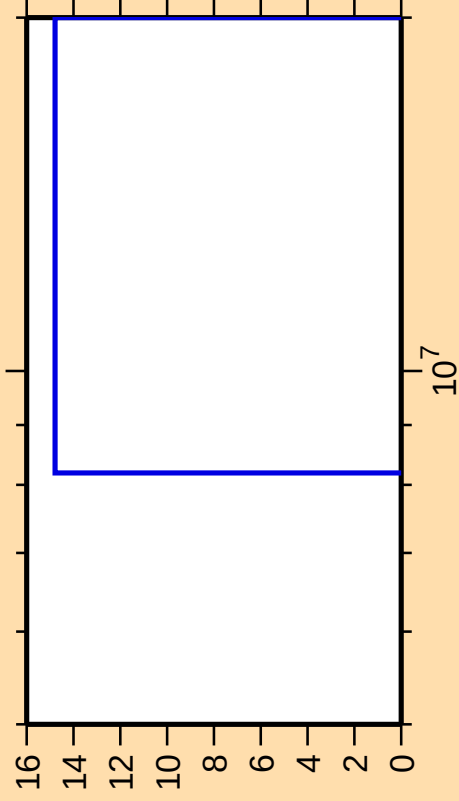
\Delta\sigma/\sigma vs. E for ^{173}\text{W}(\text{mt } 34)
