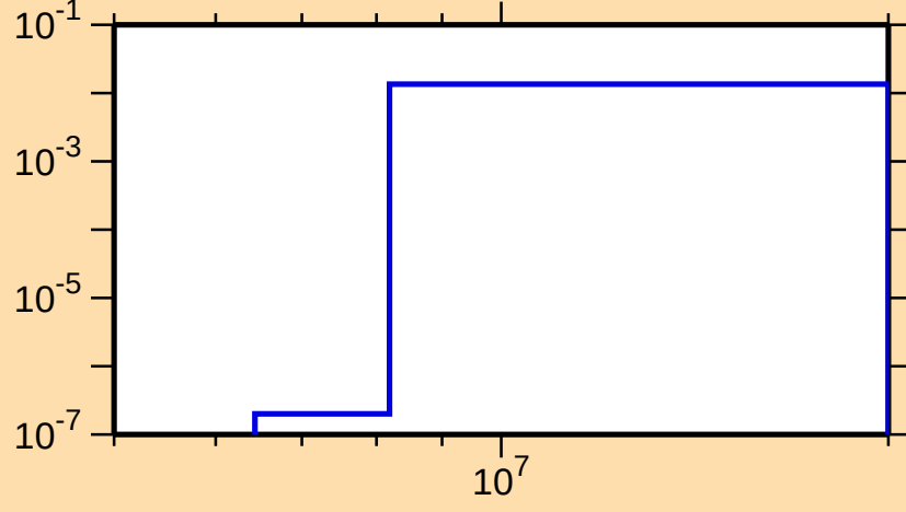
\sigma vs. E for ^{173}\text{W}(n,np)
