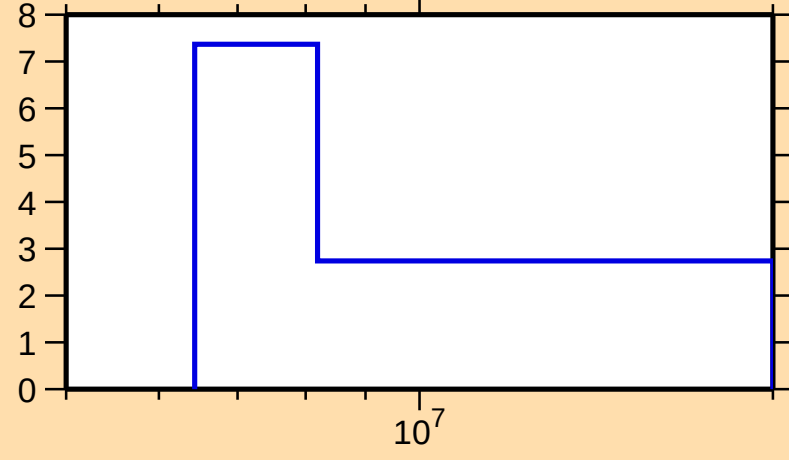
\Delta\sigma/\sigma vs. E for ^{173}\text{W}(n,\text{tot.})
