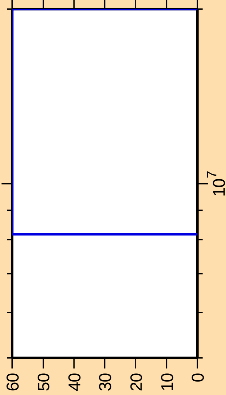
\Delta\sigma/\sigma vs. E for ^{173}\text{W}(\text{n},\text{pd})
