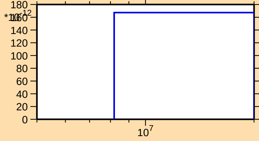
\sigma vs. E for ^{173}\text{W}(\text{n},\text{pd})
