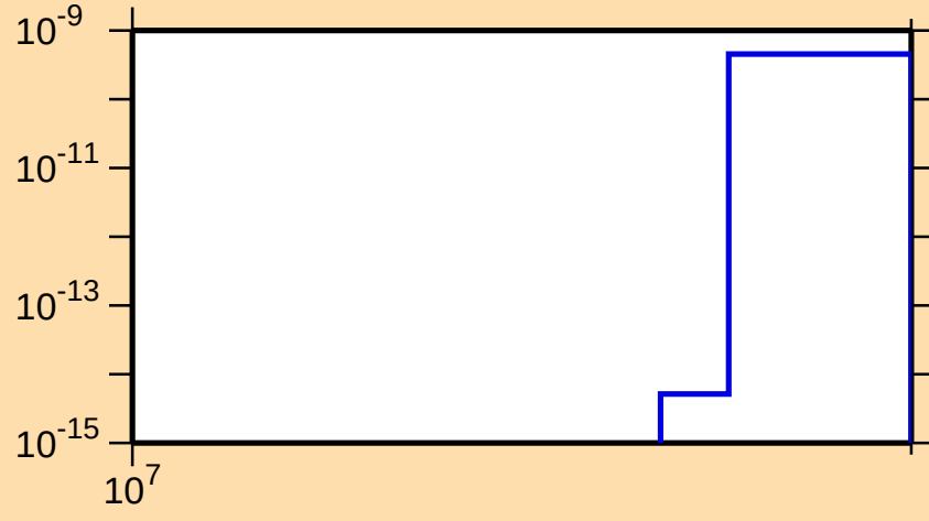
\sigma vs. E for ^{174}\text{W}(n,nt)
