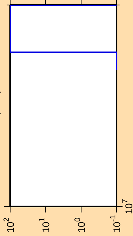
\Delta\sigma/\sigma vs. E for ^{174}\text{W}(n,nt)
