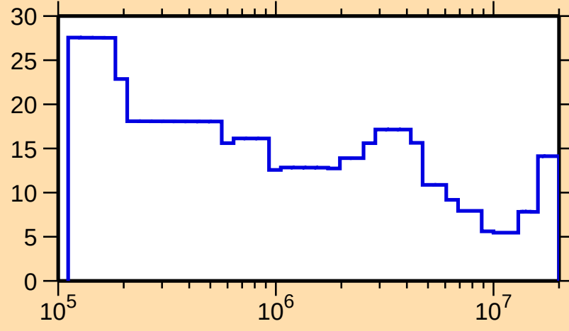
\Delta\sigma/\sigma vs. E for ^{174}\text{W}(n,\text{tot.})
