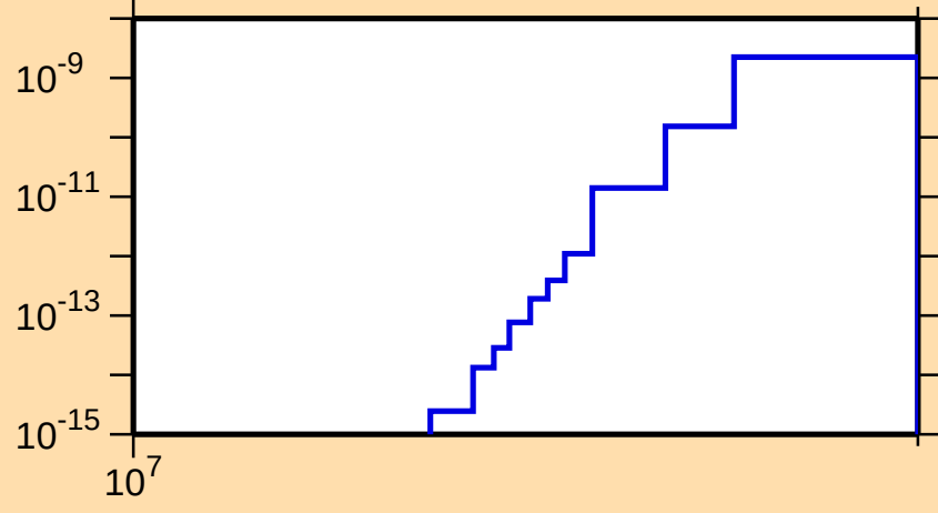
\sigma vs. E for ^{174}\text{W}(n,\text{pd})
