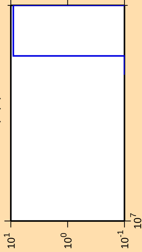
\Delta\sigma/\sigma vs. E for ^{174}\text{W}(\text{n},\text{pt})
