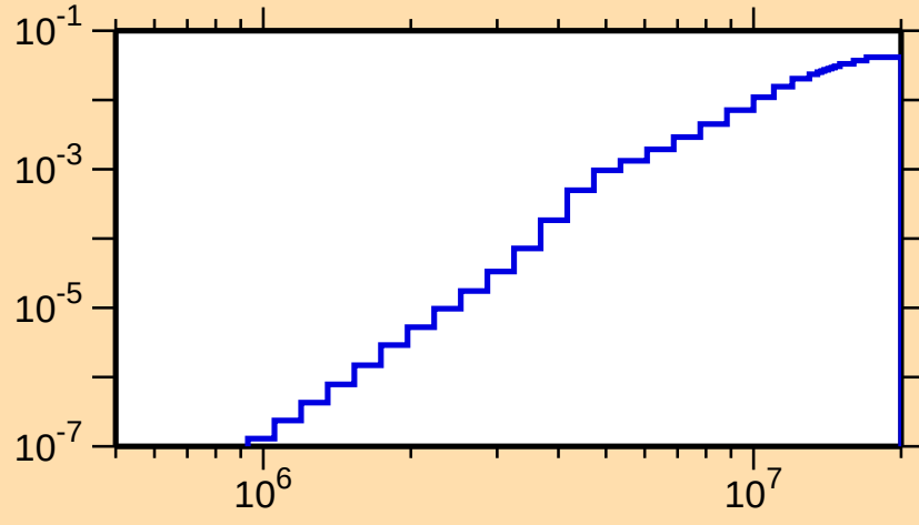
\sigma vs. E for ^{174}\text{W}(n,p)
