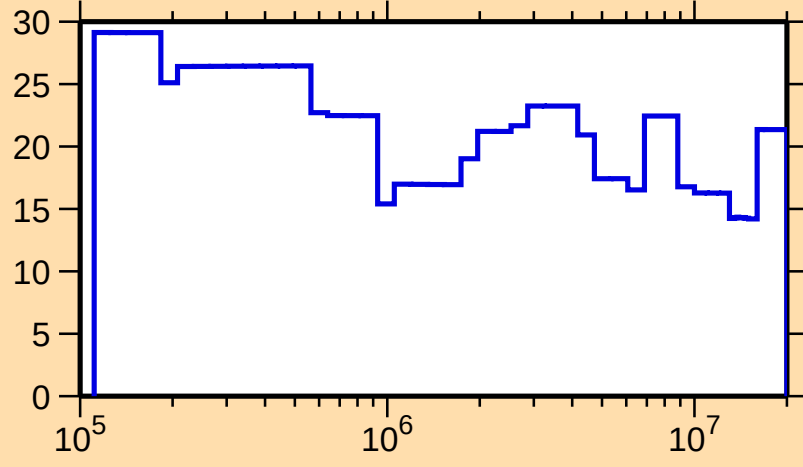
\Delta\sigma/\sigma vs. E for ^{174}\text{W}(\text{n,el.})
