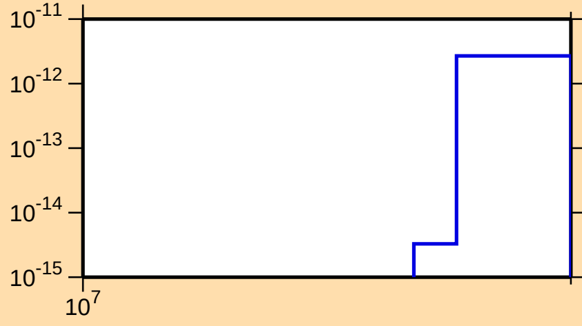
\sigma vs. E for ^{174}\text{W}(\text{n},\text{pt})
