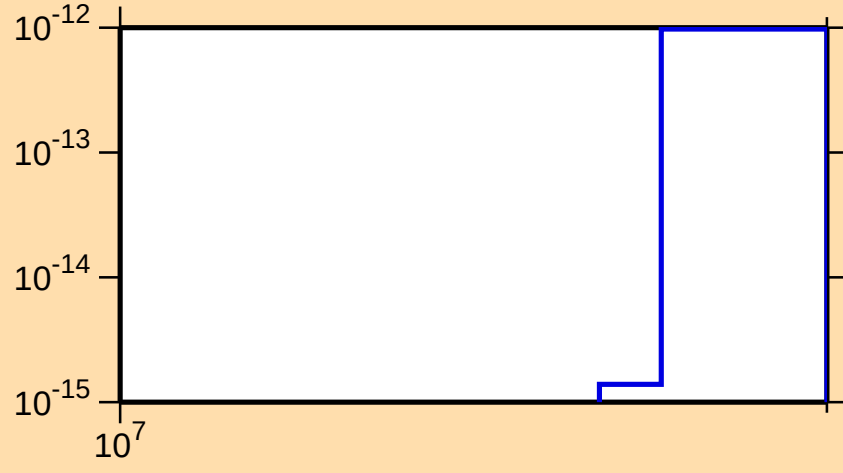
\sigma vs. E for ^{174}\text{W}(\text{mt 34})
