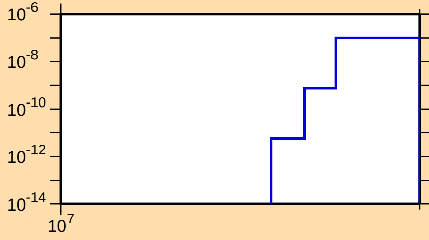
\sigma vs. E for ^{174}\text{W}(n,\text{nd})
