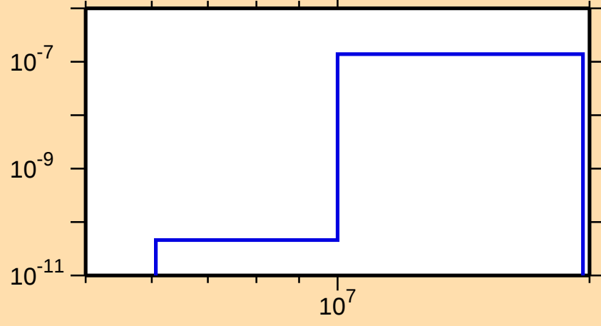
\sigma vs. E for ^{174}\text{W}(n,p\alpha)
