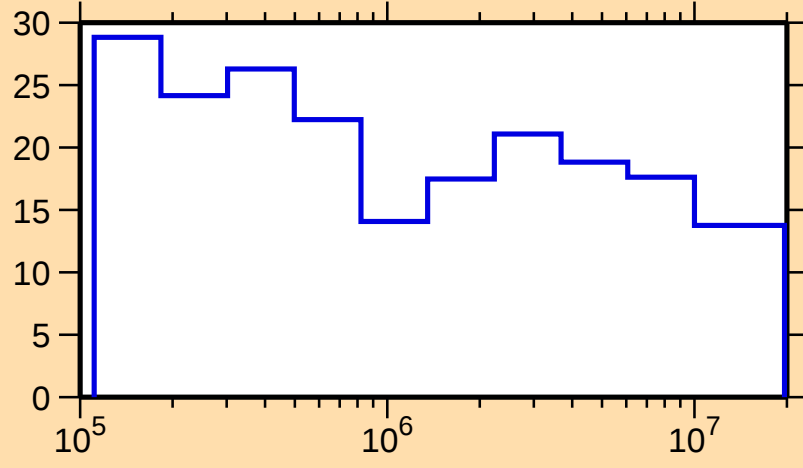
\Delta\sigma/\sigma vs. E for ^{174}\text{W}(\text{n,el.})
