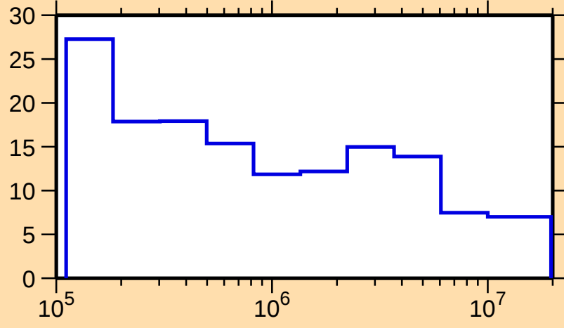
\Delta\sigma/\sigma vs. E for ^{174}\text{W}(n,\text{tot.})
