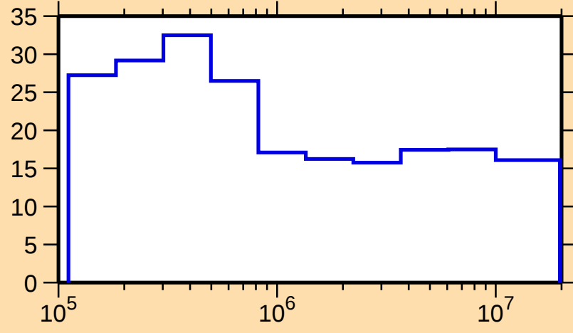
\Delta\sigma/\sigma vs. E for ^{174}\text{W}(\text{n,nonel.})
