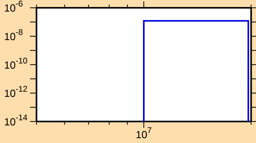
\sigma vs. E for ^{174}\text{W}(n,2n\alpha)
