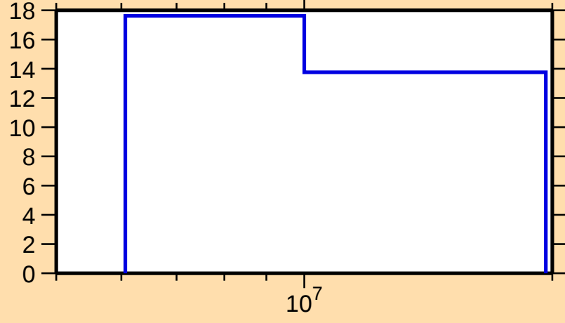
\Delta\sigma/\sigma vs. E for ^{174}\text{W}(n,\text{el.})
