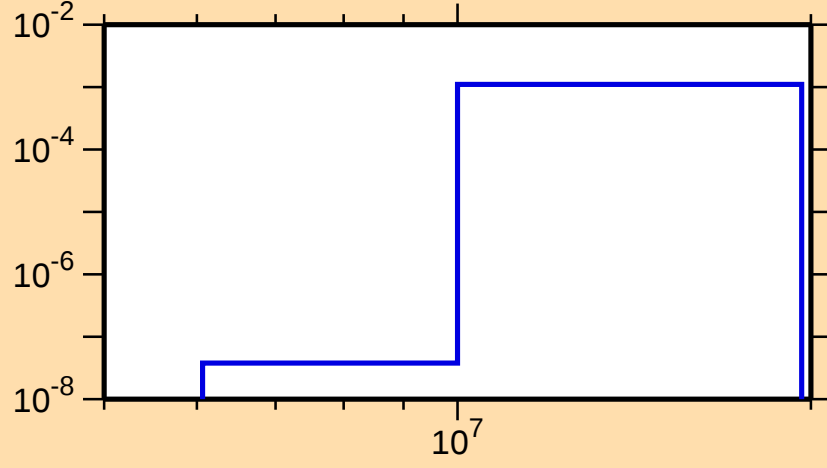
\sigma vs. E for ^{174}\text{W}(n,d)
