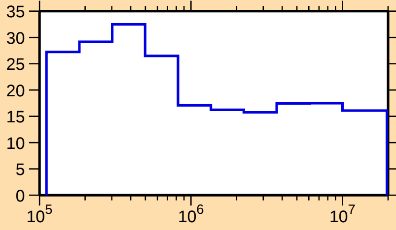
\Delta\sigma/\sigma vs. E for ^{174}\text{W}(n,\text{nonel.})
