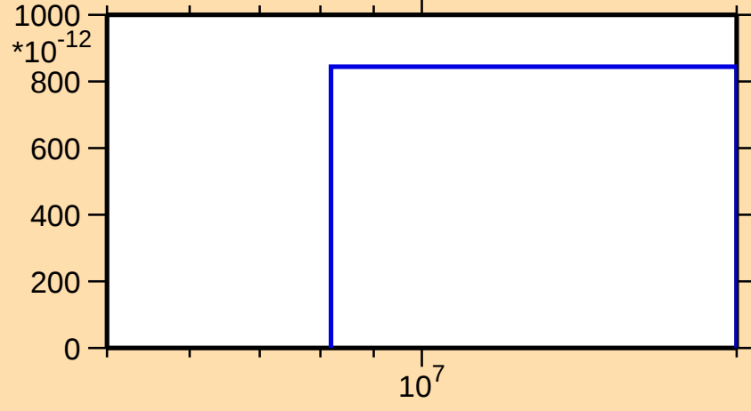
\sigma vs. E for ^{174}\text{W}(\text{n},\text{nd})
