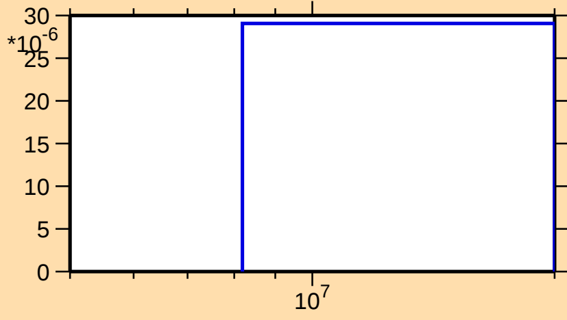
\sigma vs. E for ^{174}\text{W}(n,3n)
