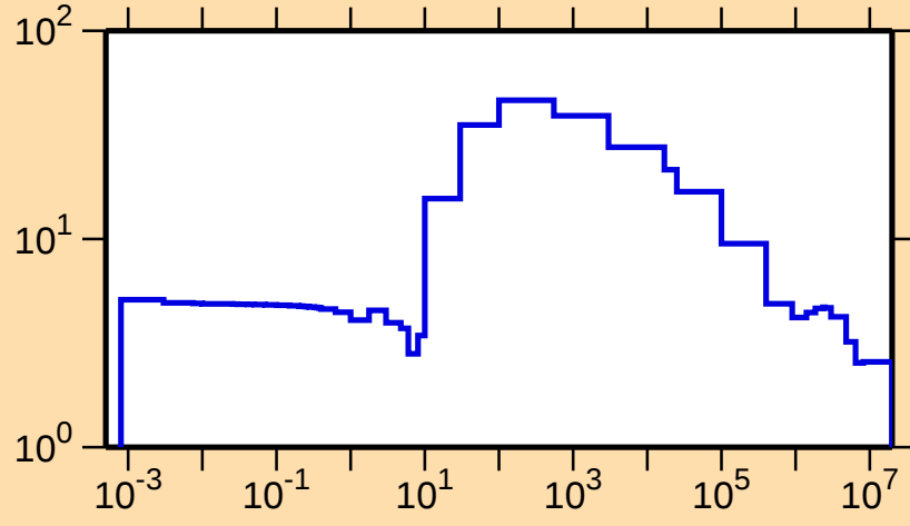
\sigma vs. E for ^{174}\text{W}(\text{n,el.})
