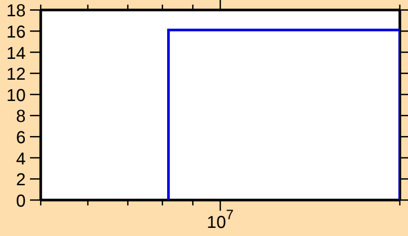
\Delta\sigma/\sigma vs. E for ^{174}\text{W}(n,\text{nonel.})
