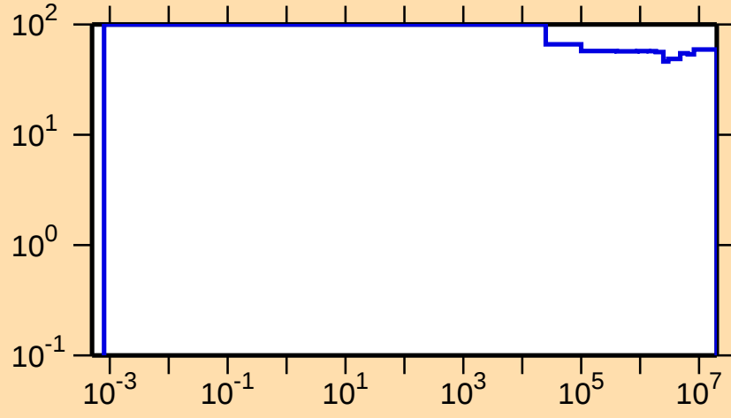
\Delta\sigma/\sigma vs. E for ^{174}\text{W}(n,p)
