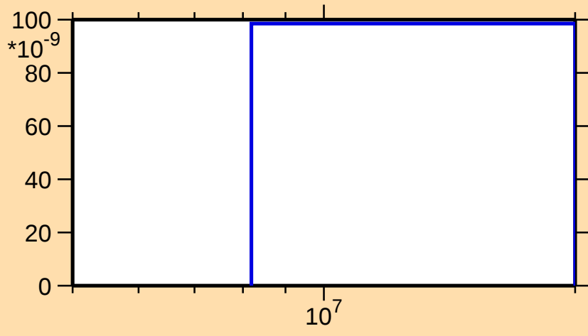
\sigma vs. E for ^{174}\text{W}(n,2n\alpha)
