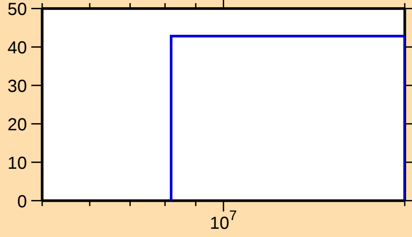
\Delta\sigma/\sigma vs. E for ^{174}\text{W}(n,\text{inel.})
