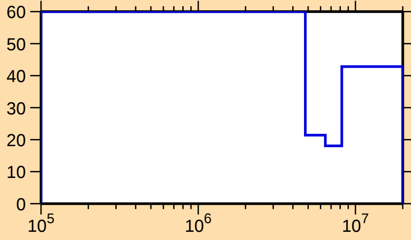
\Delta\sigma/\sigma vs. E for ^{174}\text{W}(n,\text{inel.})
