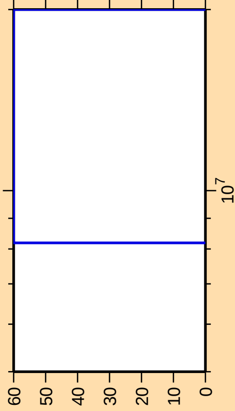
\Delta\sigma/\sigma vs. E for ^{174}\text{W}(\text{n},\text{nd})
