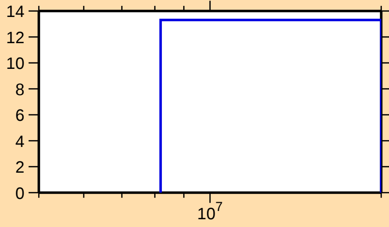
\Delta\sigma/\sigma vs. E for ^{174}\text{W}(n,\text{el.})
