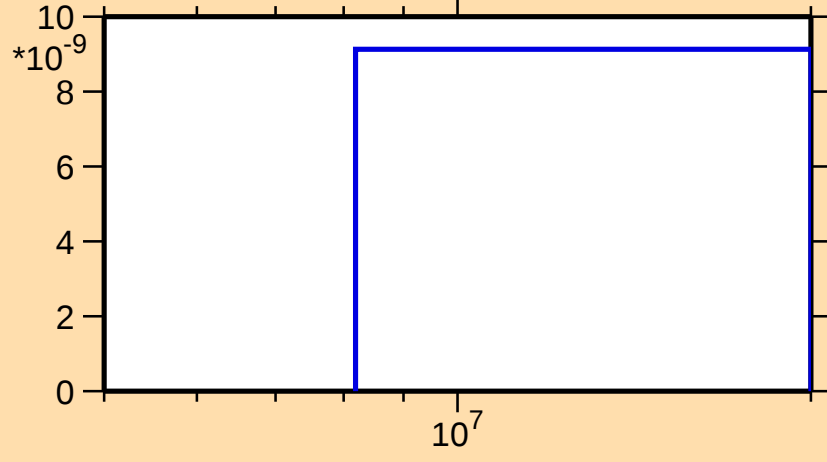
\sigma vs. E for ^{174}\text{W}(n,2np)
