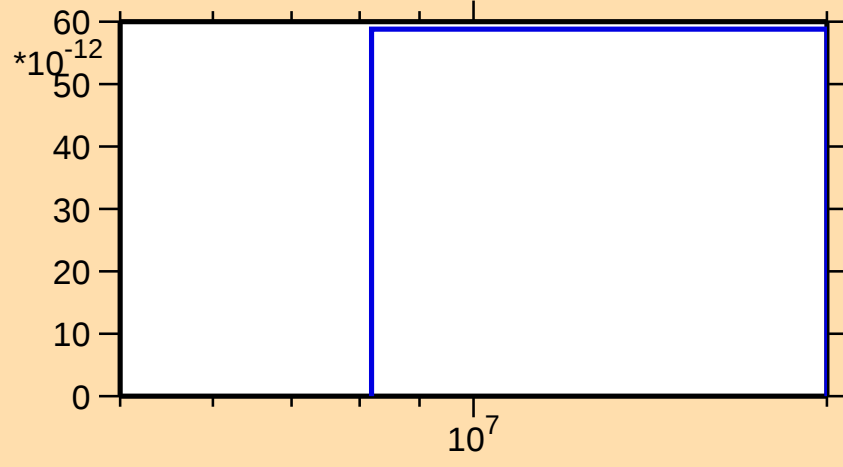
\sigma vs. E for ^{174}\text{W}(\text{mt } 45)
