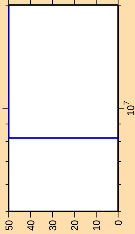
\Delta\sigma/\sigma vs. E for ^{174}\text{W}(n,n\text{cont.})
