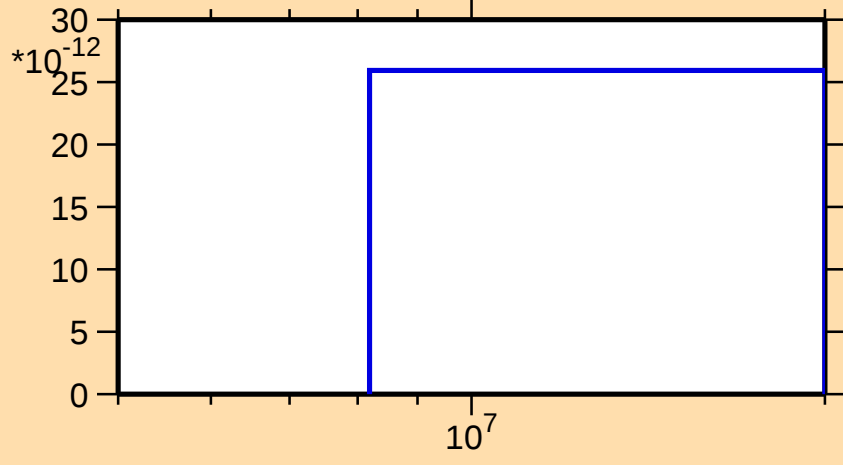
\sigma vs. E for ^{174}\text{W}(\text{n},\text{pd})
