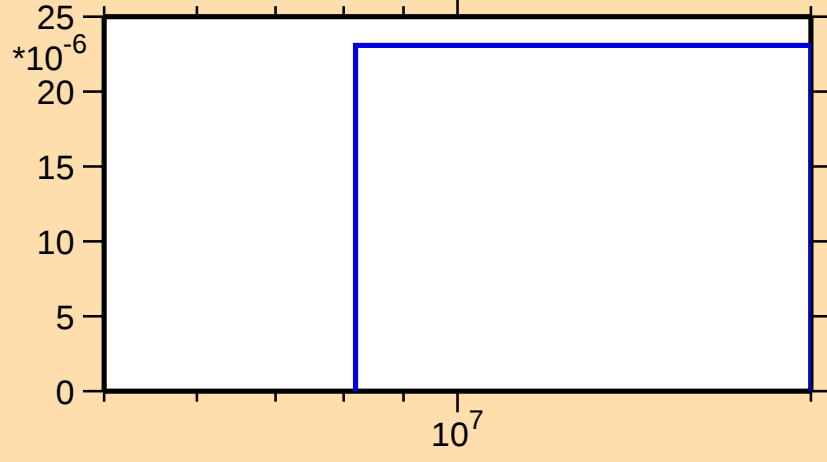
\sigma vs. E for ^{174}\text{W}(n,t)
