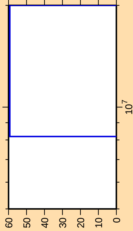
\Delta\sigma/\sigma vs. E for ^{174}\text{W}(n,p)
