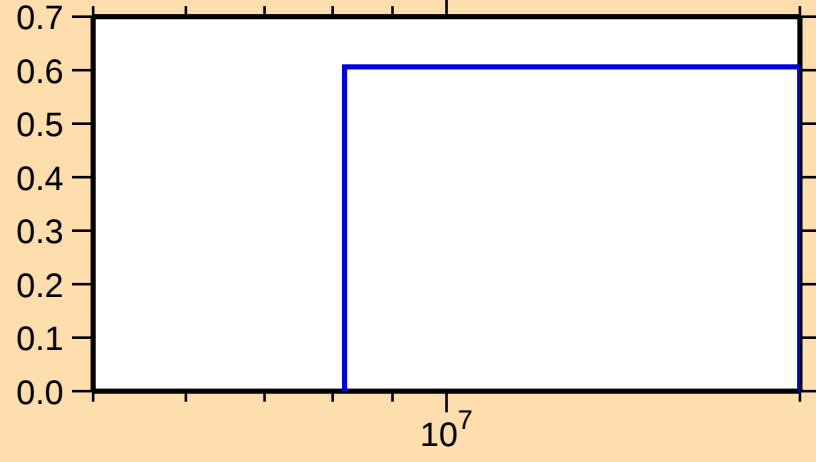
\sigma vs. E for ^{174}\text{W}(n,2n)
