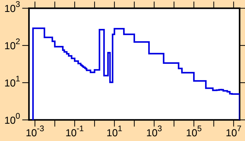
\sigma vs. E for ^{174}\text{W}(n,\text{tot.})
