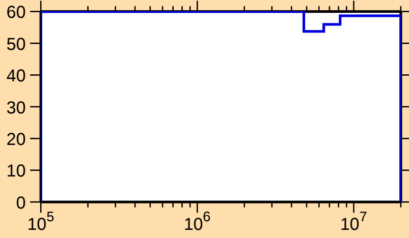
\Delta\sigma/\sigma vs. E for ^{174}\text{W}(n,n_1)
