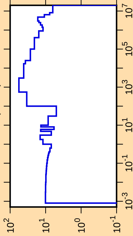
\Delta\sigma/\sigma vs. E for ^{174}\text{W}(n,\text{tot.})
