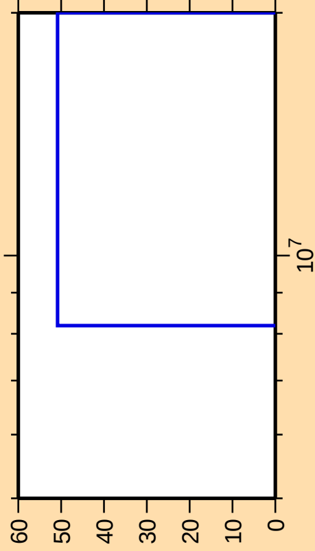
\Delta\sigma/\sigma vs. E for ^{174}\text{W}(n,2n)
