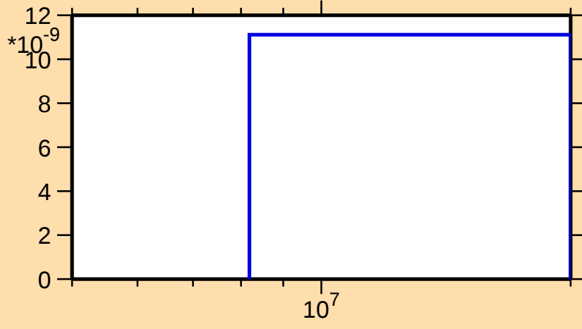
\sigma vs. E for ^{174}\text{W}(n,\text{He3})
