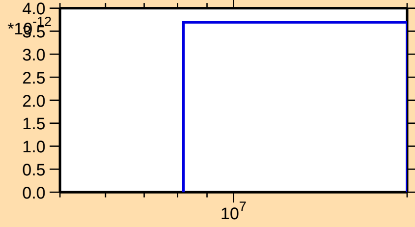
\sigma vs. E for ^{174}\text{W}(\text{n},\text{nt})
