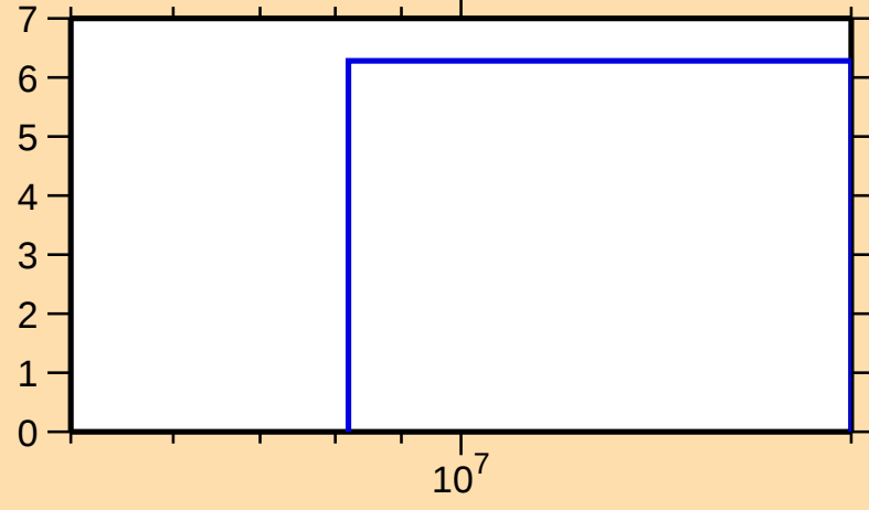
\Delta\sigma/\sigma vs. E for ^{174}\text{W}(n,\text{tot.})
