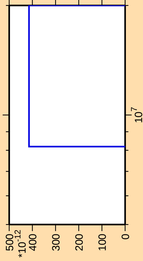
\Delta\sigma/\sigma vs. E for ^{174}\text{W}(\text{mt 11})
