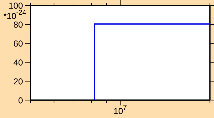
\sigma vs. E for ^{174}\text{W}(\text{mt 11})
