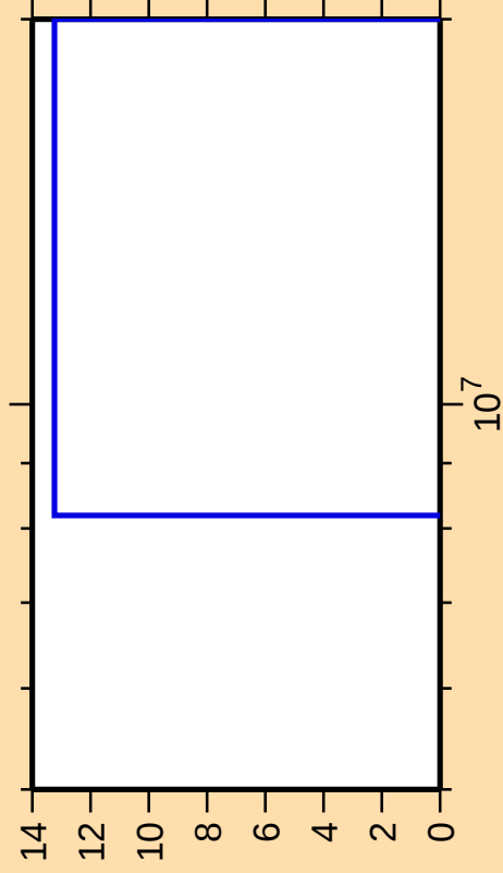
\Delta\sigma/\sigma vs. E for ^{174}\text{W}(\text{n},\text{nt})
