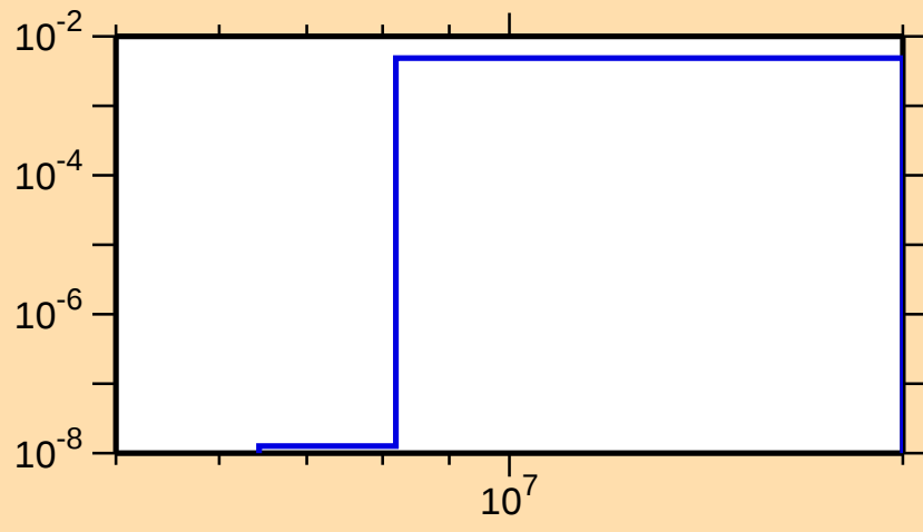
\sigma vs. E for ^{174}\text{W}(n,np)
