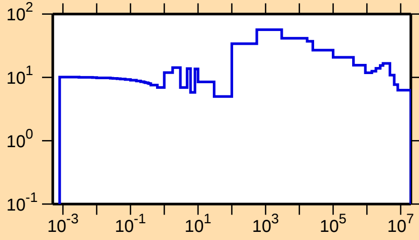
\Delta\sigma/\sigma vs. E for ^{174}\text{W}(\text{n,tot.})
