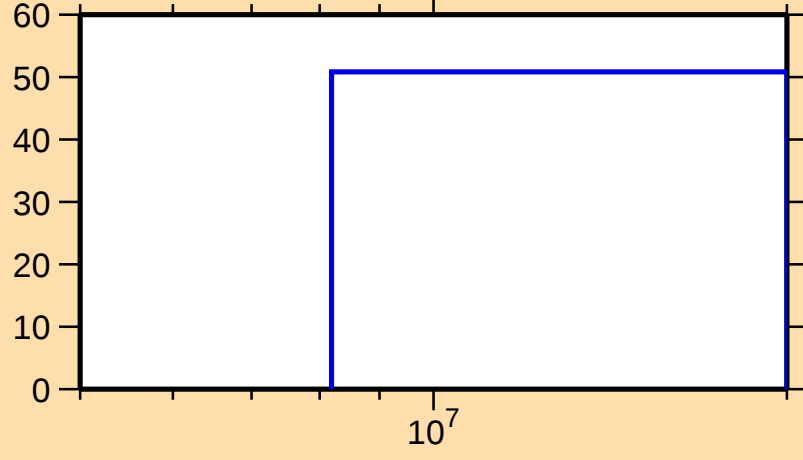
\Delta\sigma/\sigma vs. E for ^{174}\text{W}(n,2n)
