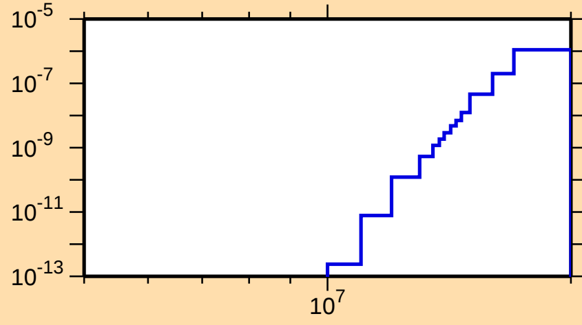
\sigma vs. E for ^{175}\text{W}(n,\text{He3})
