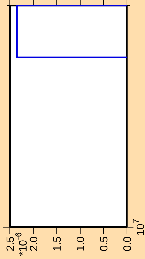
\Delta\sigma/\sigma vs. E for ^{175}\text{W}(\text{mt 11})
