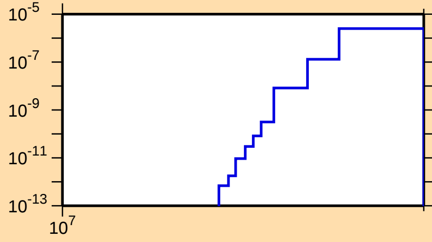
\sigma vs. E for ^{175}\text{W}(n,\text{nd})
