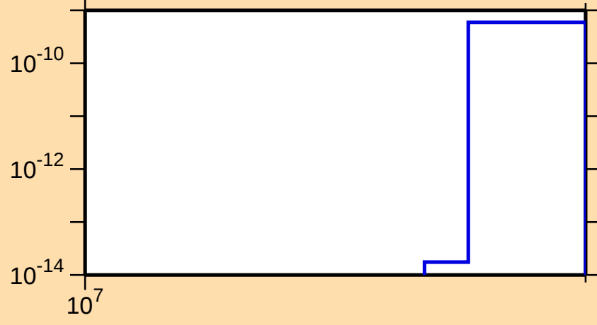
\sigma vs. E for ^{175}\text{W}(n,nt)
