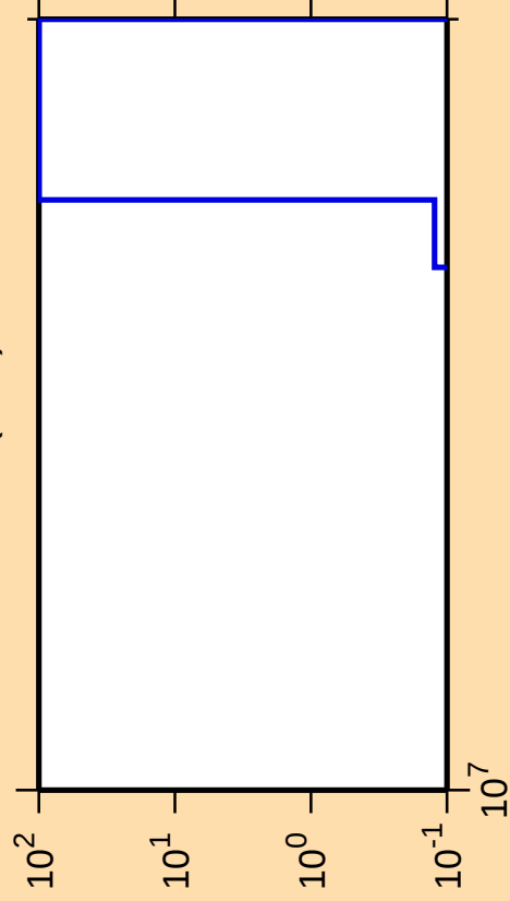
\Delta\sigma/\sigma vs. E for ^{175}\text{W}(n,nt)
