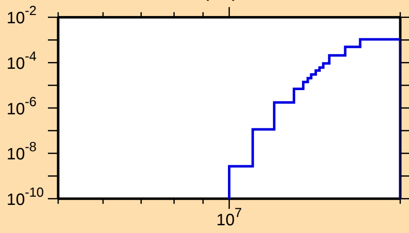
\sigma vs. E for ^{175}\text{W}(n,t)
