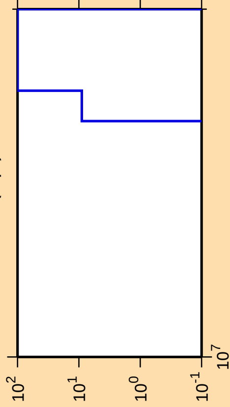
\Delta\sigma/\sigma vs. E for ^{175}\text{W}(\text{n},\text{pt})
