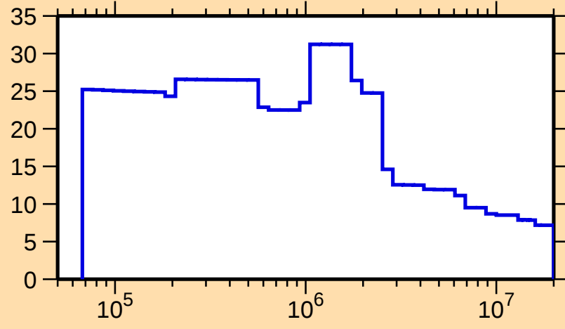
\Delta\sigma/\sigma vs. E for ^{175}\text{W}(\text{n,nonel.})
