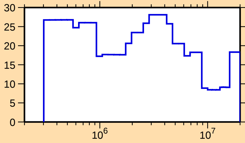
\Delta\sigma/\sigma vs. E for ^{175}\text{W}(n,\text{el.})
