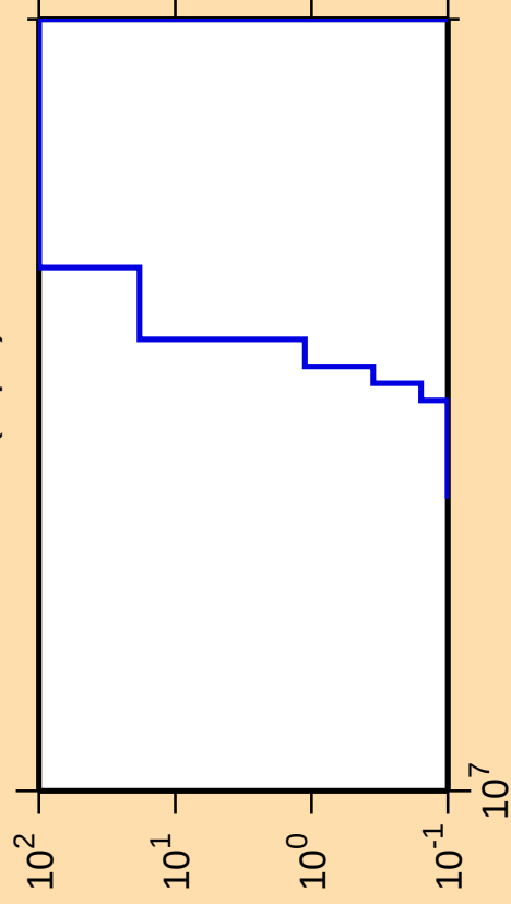
\Delta\sigma/\sigma vs. E for ^{175}\text{W}(n,\text{pd})
