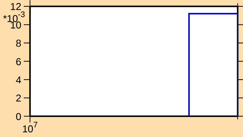
\sigma vs. E for ^{175}\text{W}(n,3n)
