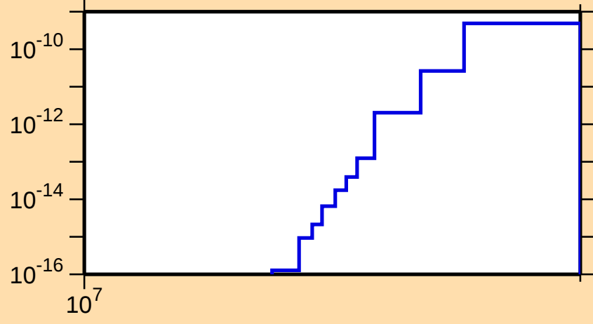
\sigma vs. E for ^{175}\text{W}(n,\text{pd})
