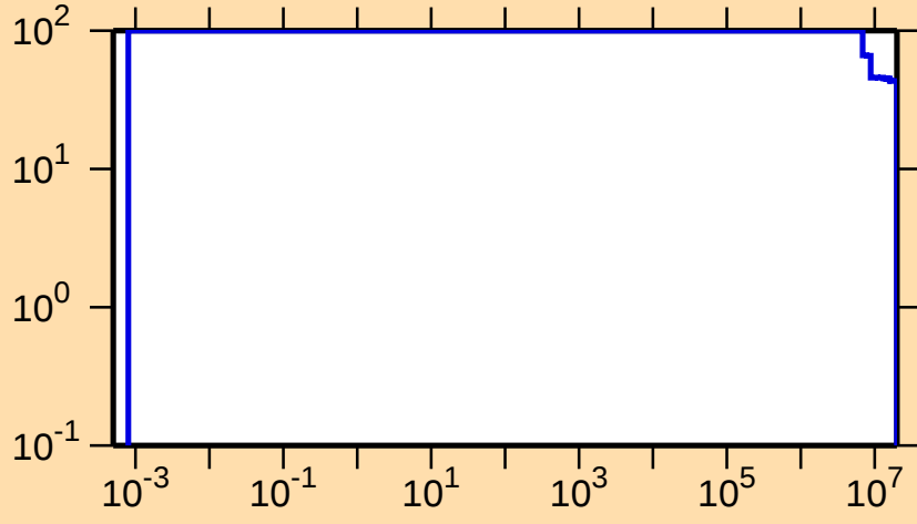
\Delta\sigma/\sigma vs. E for ^{175}\text{W}(n,p)
