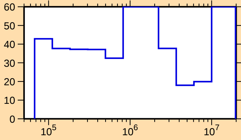
\Delta\sigma/\sigma vs. E for ^{175}\text{W}(n,\text{inel.})
