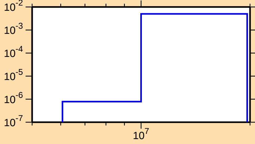
\sigma vs. E for ^{175}\text{W}(n,np)
