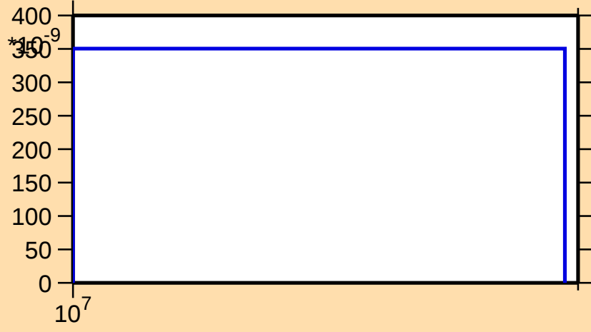
\sigma vs. E for ^{175}\text{W}(n,2np)
