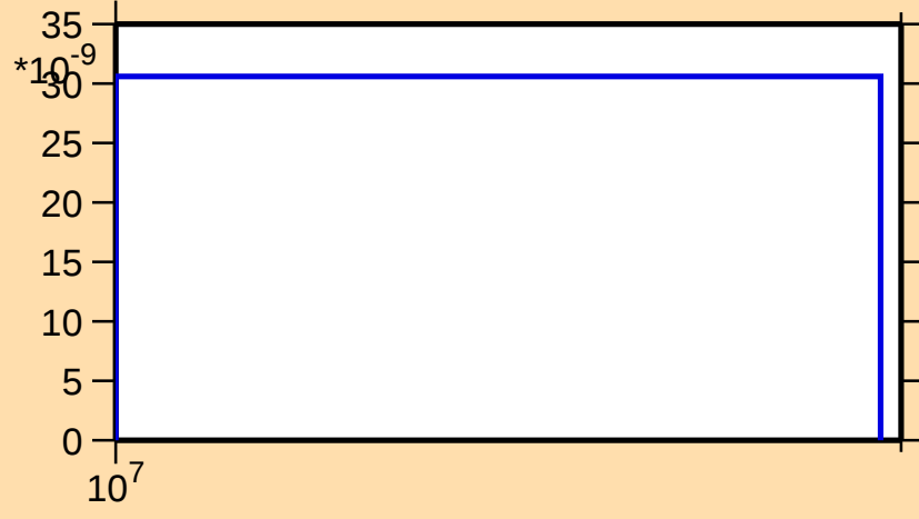
\sigma vs. E for ^{175}\text{W}(\text{n},\text{nd})
