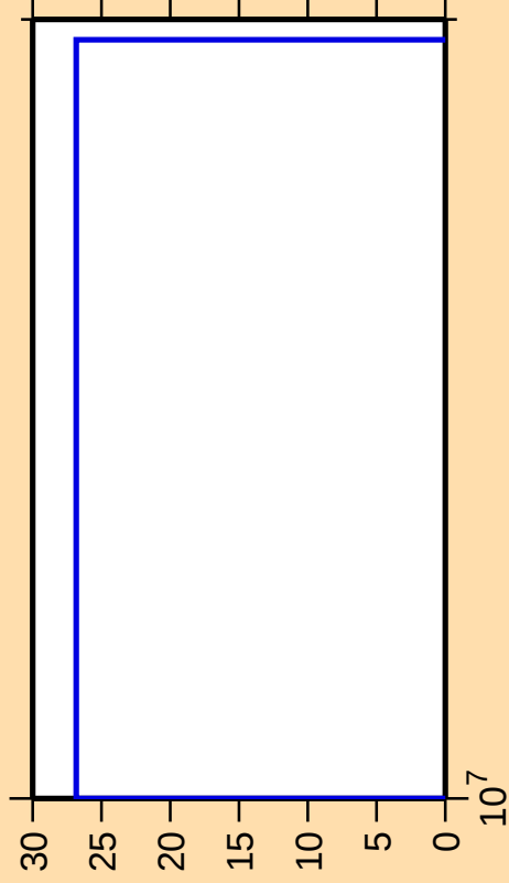
\Delta\sigma/\sigma vs. E for ^{175}\text{W}(\text{n},\text{pd})
