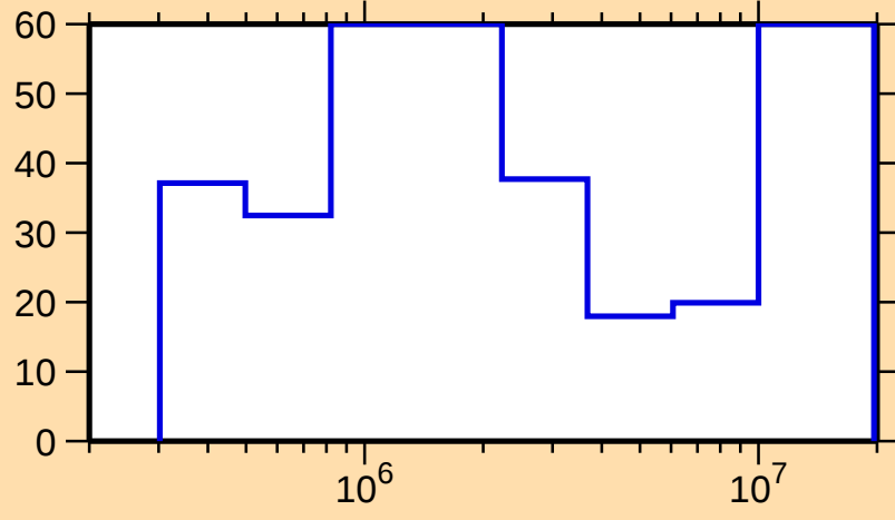
\Delta\sigma/\sigma vs. E for ^{175}\text{W}(\text{n},\text{inel.})
