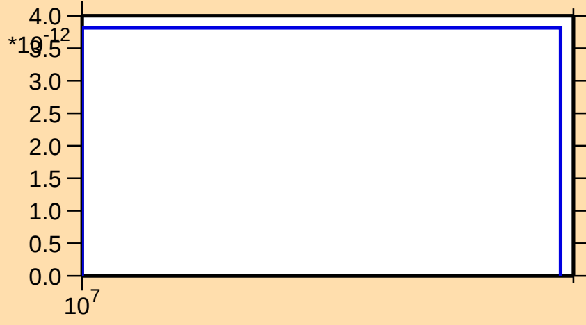
\sigma vs. E for ^{175}\text{W}(n,\text{nt})
