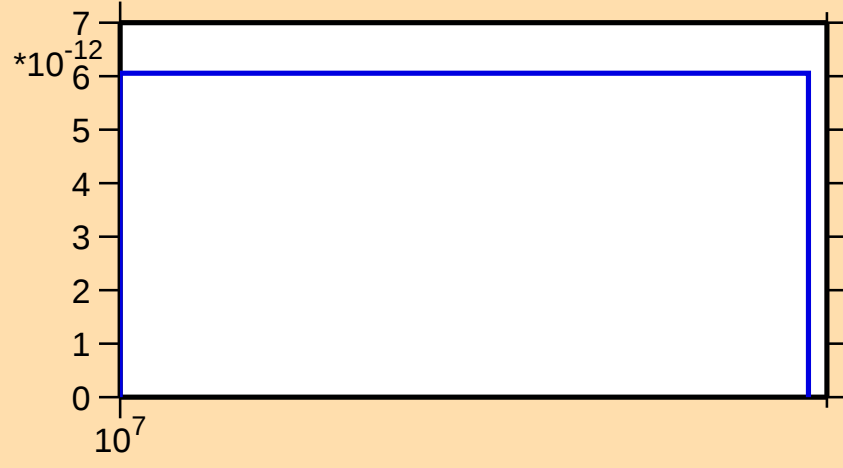
\sigma vs. E for ^{175}\text{W}(\text{n},\text{pd})
