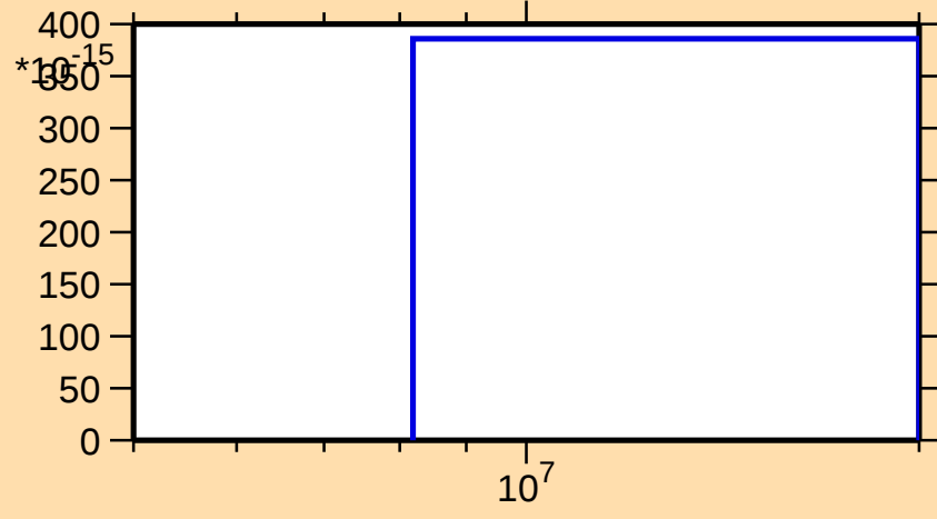
\sigma vs. E for ^{175}\text{W}(\text{mt } 34)
