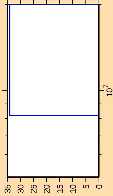
\Delta\sigma/\sigma vs. E for ^{175}\text{W}(n,\text{nt})
