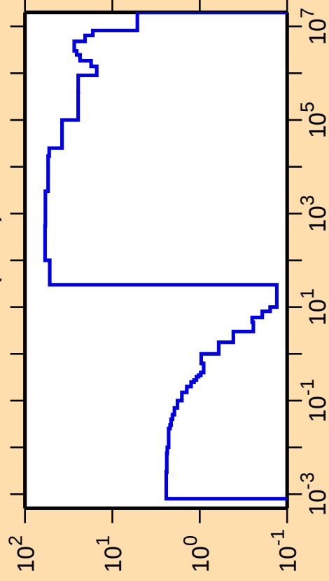
\Delta\sigma/\sigma vs. E for ^{175}\text{W}(\text{n,el.})
