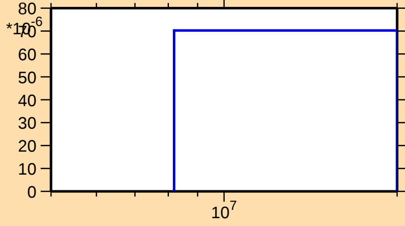
\sigma vs. E for ^{175}\text{W}(n,t)
