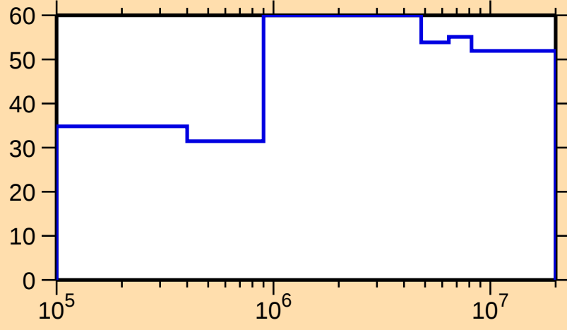
\Delta\sigma/\sigma vs. E for ^{175}\text{W}(n,n_1)
