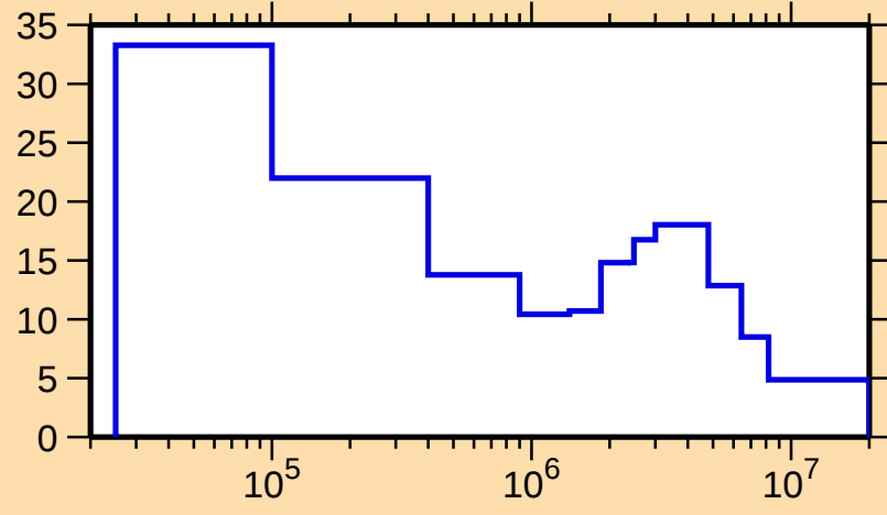
\Delta\sigma/\sigma vs. E for ^{175}\text{W}(n,\text{tot.})
