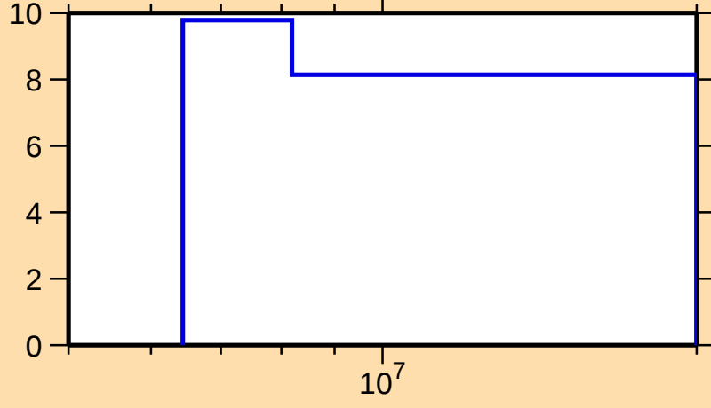
\Delta\sigma/\sigma vs. E for ^{175}\text{W}(n,\text{nonel.})
