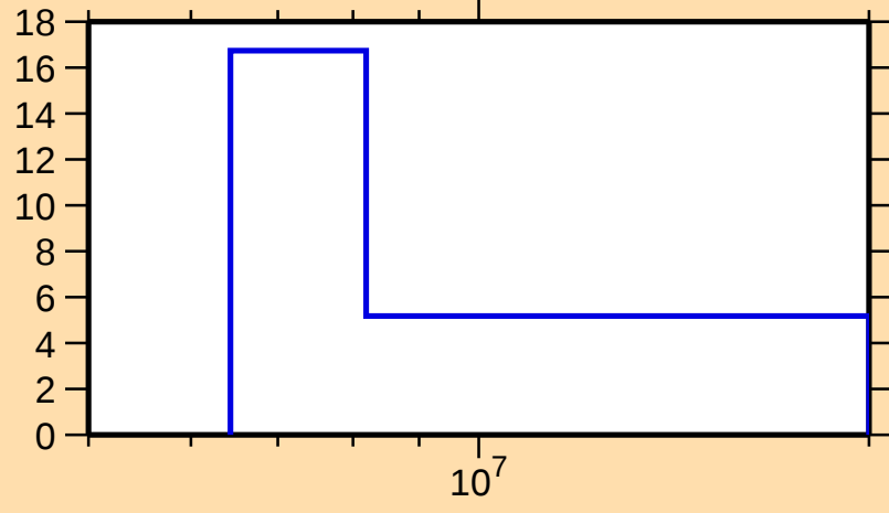
\Delta\sigma/\sigma vs. E for ^{175}\text{W}(n,\text{el.})
