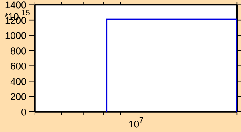
\sigma vs. E for ^{175}\text{W}(\text{n},\text{pt})
