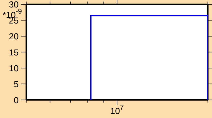
\sigma vs. E for ^{175}\text{W}(n,\text{nd})
