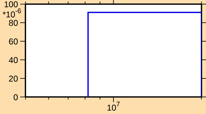
\sigma vs. E for ^{175}\text{W}(n,3n)
