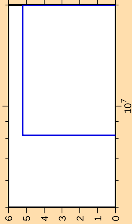
\Delta\sigma/\sigma vs. E for ^{175}\text{W}(\text{mt117})
