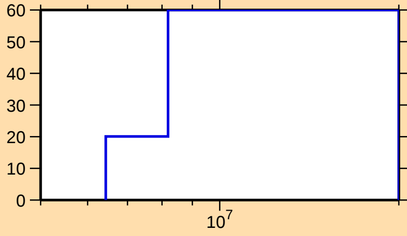
\Delta\sigma/\sigma vs. E for ^{175}\text{W}(n,\text{inel.})
