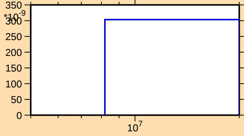
\sigma vs. E for ^{175}\text{W}(n,2np)
