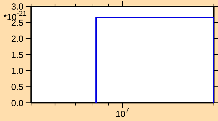
\sigma vs. E for ^{175}\text{W}(\text{mt 11})
