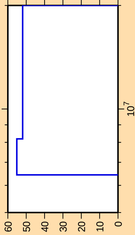
\Delta\sigma/\sigma vs. E for ^{175}\text{W}(n,n_1)
