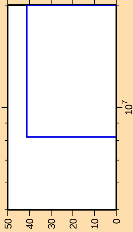
\Delta\sigma/\sigma vs. E for ^{175}\text{W}(\text{mt } 45)
