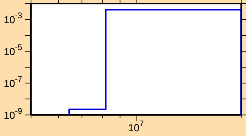
\sigma vs. E for ^{175}\text{W}(n,np)
