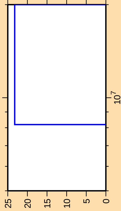
\Delta\sigma/\sigma vs. E for ^{175}\text{W}(\text{n,pd})
