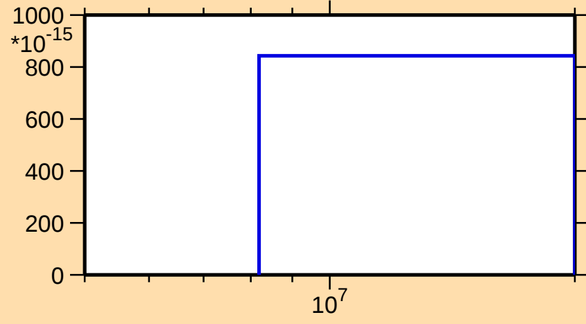
\sigma vs. E for ^{175}\text{W}(\text{mt117})
