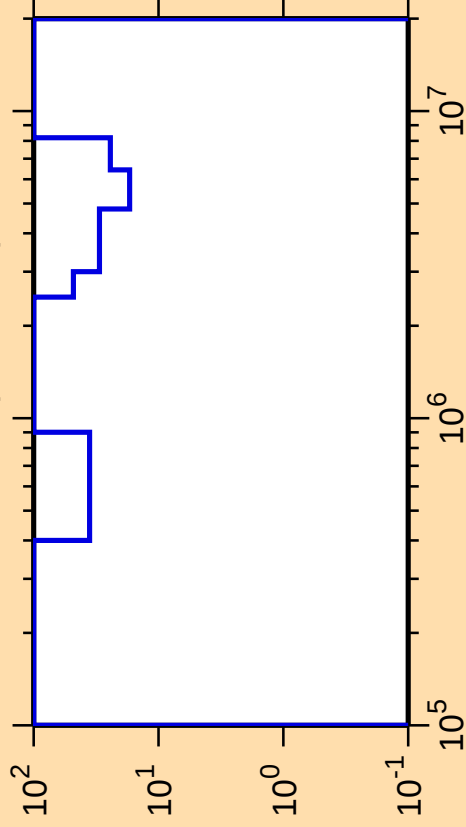
\Delta\sigma/\sigma vs. E for ^{175}\text{W}(\text{n},\text{ncont.})
