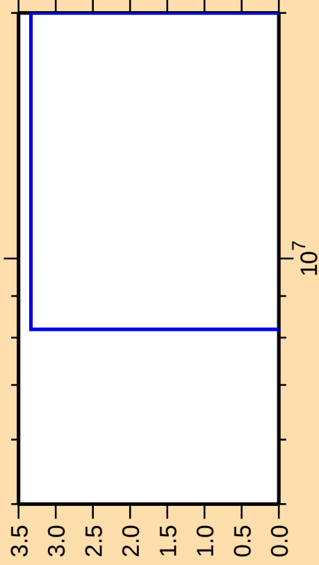
\Delta\sigma/\sigma vs. E for ^{175}\text{W}(\text{mt } 34)
