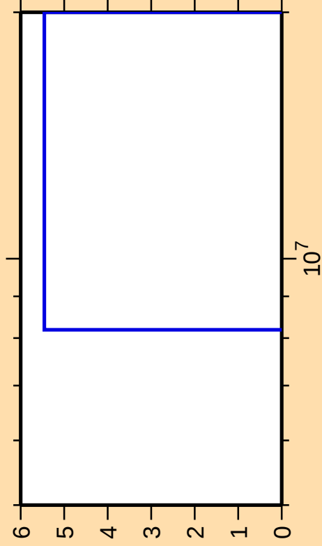
\Delta\sigma/\sigma vs. E for ^{175}\text{W}(\text{n},\text{pt})
