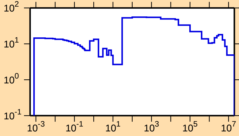
\Delta\sigma/\sigma vs. E for ^{175}\text{W}(\text{n,tot.})
