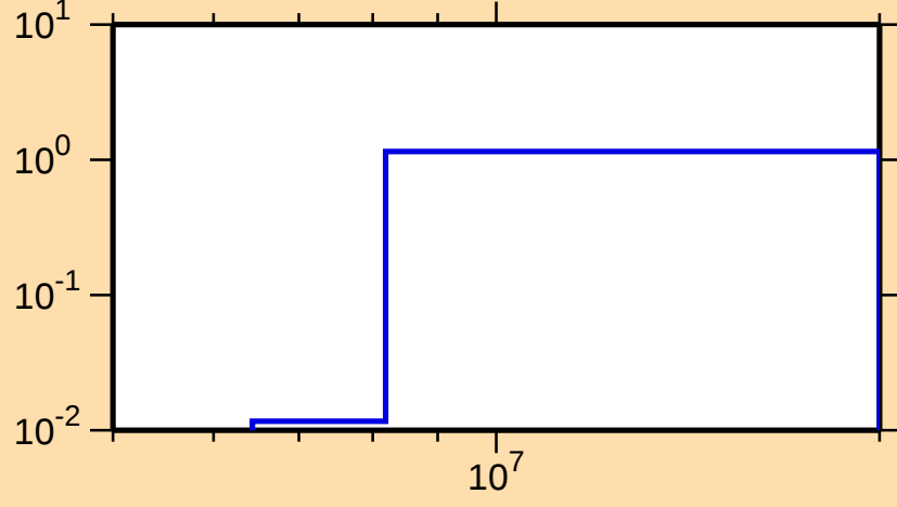
\sigma vs. E for ^{175}\text{W}(n,2n)
