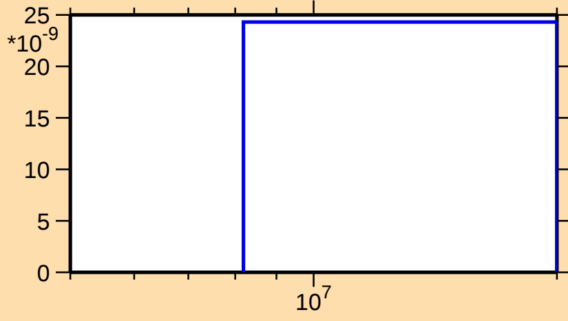
\sigma vs. E for ^{175}\text{W}(n,\text{He3})
