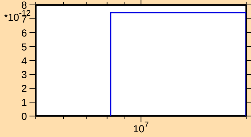
\sigma vs. E for ^{175}\text{W}(\text{mt } 45)
