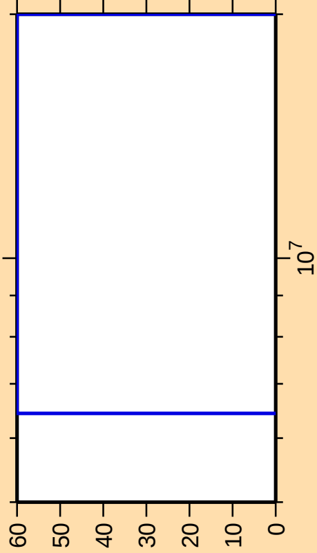
\Delta\sigma/\sigma vs. E for ^{175}\text{W}(n,\gamma)
