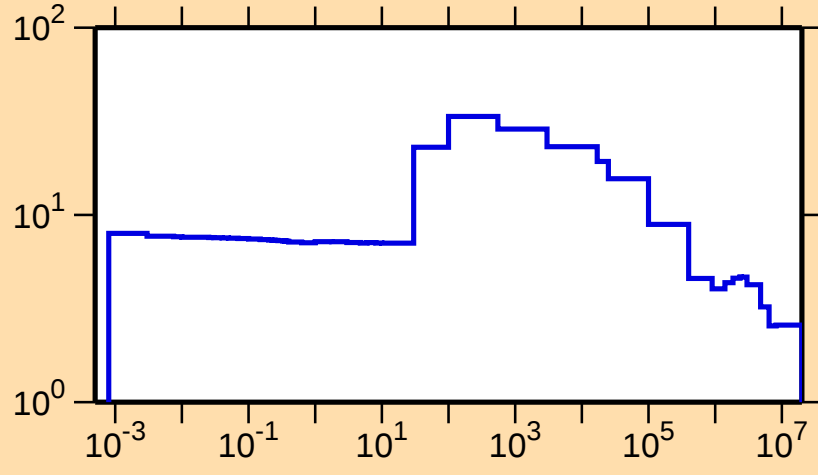
\sigma vs. E for ^{175}\text{W}(\text{n,el.})
