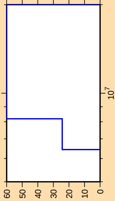
\Delta\sigma/\sigma vs. E for ^{175}\text{W}(n,n\text{cont.})
