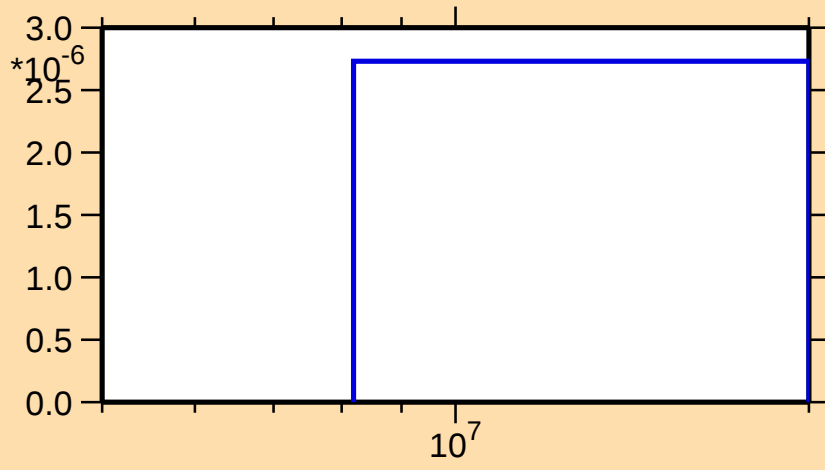
\sigma vs. E for ^{175}\text{W}(n,2n\alpha)
