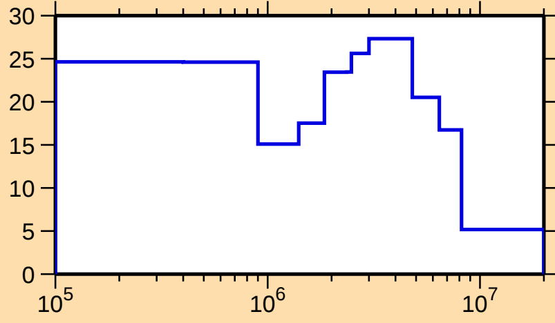
\Delta\sigma/\sigma vs. E for ^{175}\text{W}(\text{n},\text{el.})
