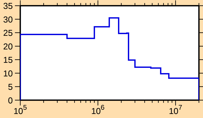
\Delta\sigma/\sigma vs. E for ^{175}\text{W}(\text{n},\text{nonel.})
