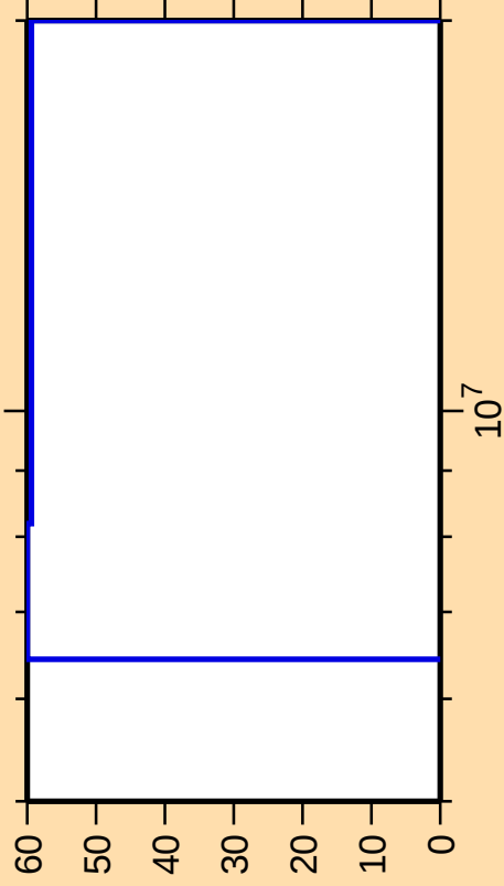
\Delta\sigma/\sigma vs. E for ^{175}\text{W}(n,2n)
