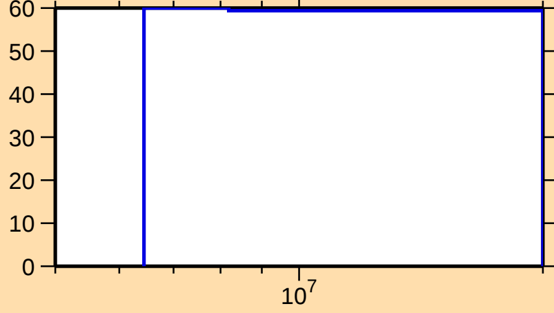
\Delta\sigma/\sigma vs. E for ^{175}\text{W}(n,2n)
