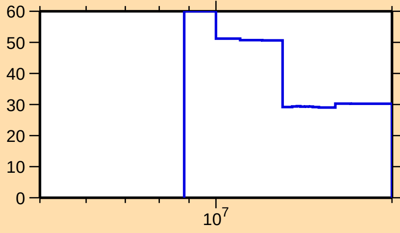
\Delta\sigma/\sigma vs. E for ^{176}\text{W}(n,2n)
