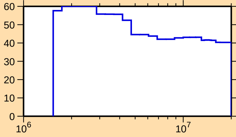
\Delta\sigma/\sigma vs. E for ^{176}\text{W}(n,n_1)
