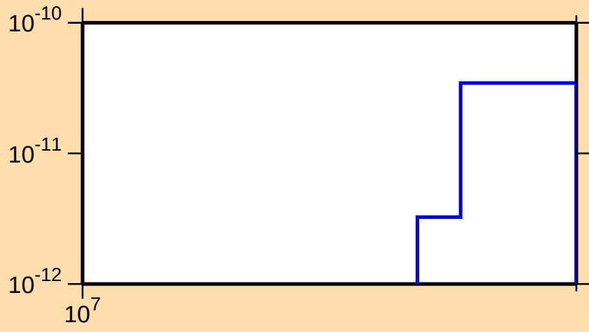
\sigma vs. E for ^{176}\text{W}(\text{mt117})
