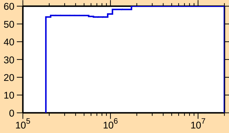
\Delta\sigma/\sigma vs. E for ^{176}\text{W}(n,\gamma)
