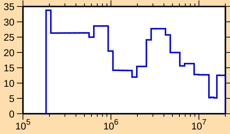
\Delta\sigma/\sigma vs. E for ^{176}\text{W}(n,\text{el.})
