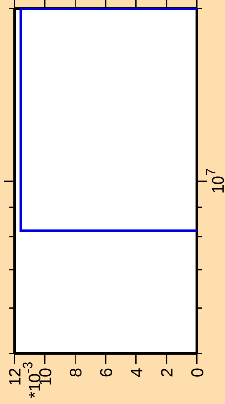
\Delta\sigma/\sigma vs. E for ^{176}\text{W}(\text{n},\text{pt})
