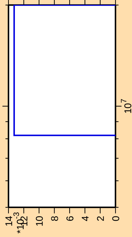
\Delta\sigma/\sigma vs. E for ^{176}\text{W}(\text{mt } 34)
