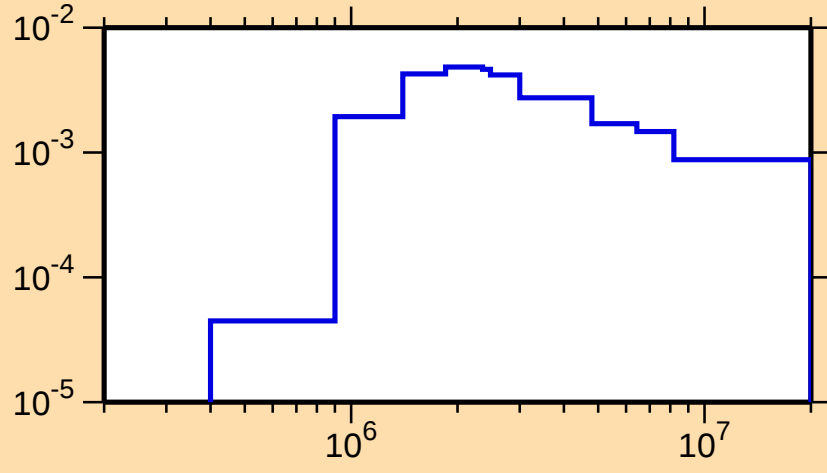
\sigma vs. E for ^{176}\text{W}(n,n_3)
