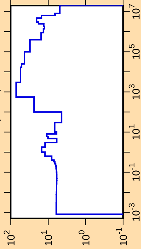
\Delta\sigma/\sigma vs. E for ^{176}\text{W}(n,\text{tot.})
