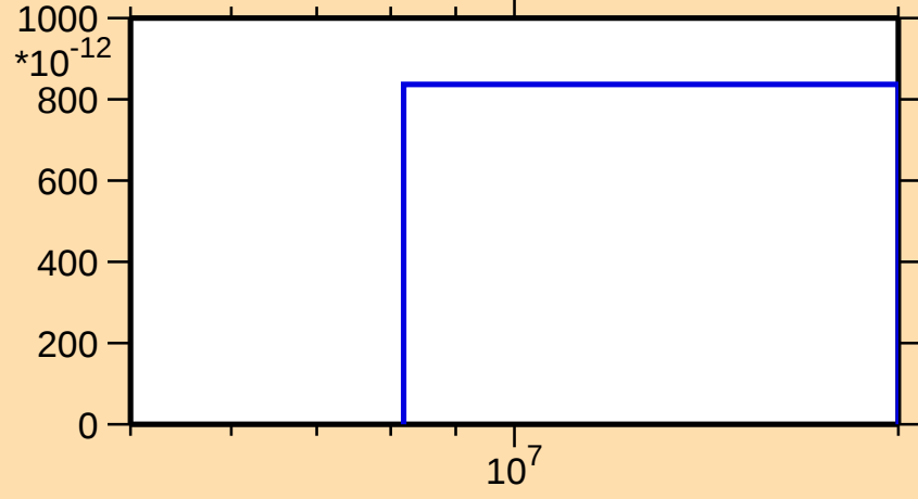
\sigma vs. E for ^{176}\text{W}(\text{n},\text{nd})
