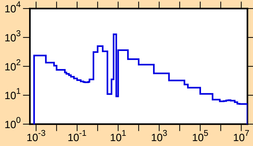
\sigma vs. E for ^{176}\text{W}(n,\text{tot.})
