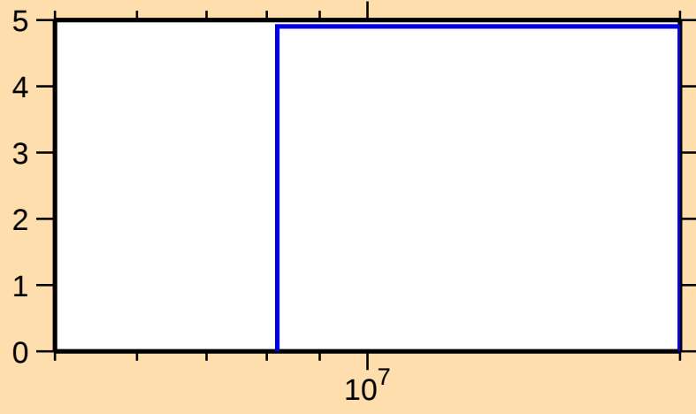
\Delta\sigma/\sigma vs. E for ^{176}\text{W}(n,\text{tot.})
