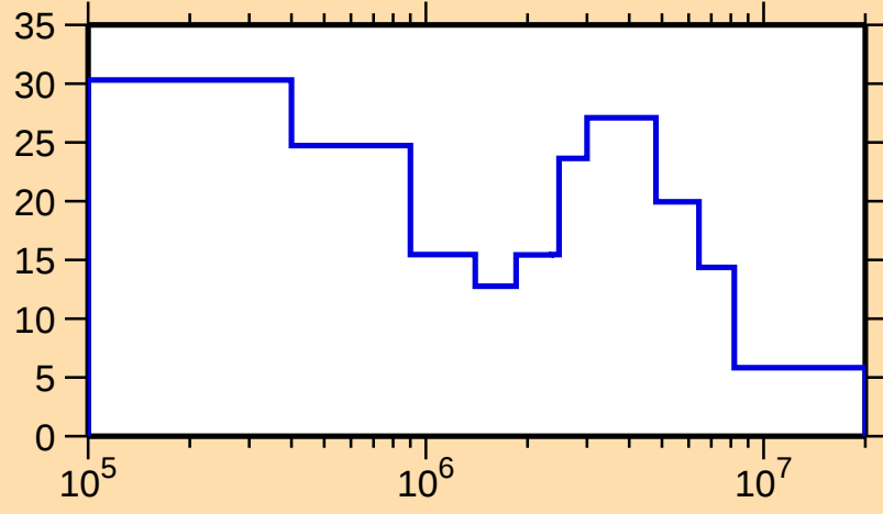
\Delta\sigma/\sigma vs. E for ^{176}\text{W}(\text{n,el.})
