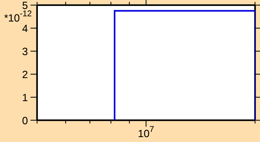
\sigma vs. E for ^{176}\text{W}(n,\text{nt})
