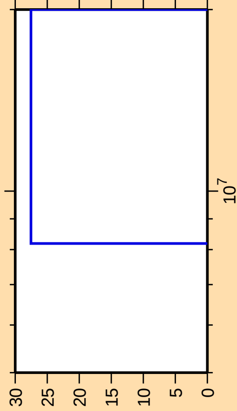
\Delta\sigma/\sigma vs. E for ^{176}\text{W}(n,\text{nt})
