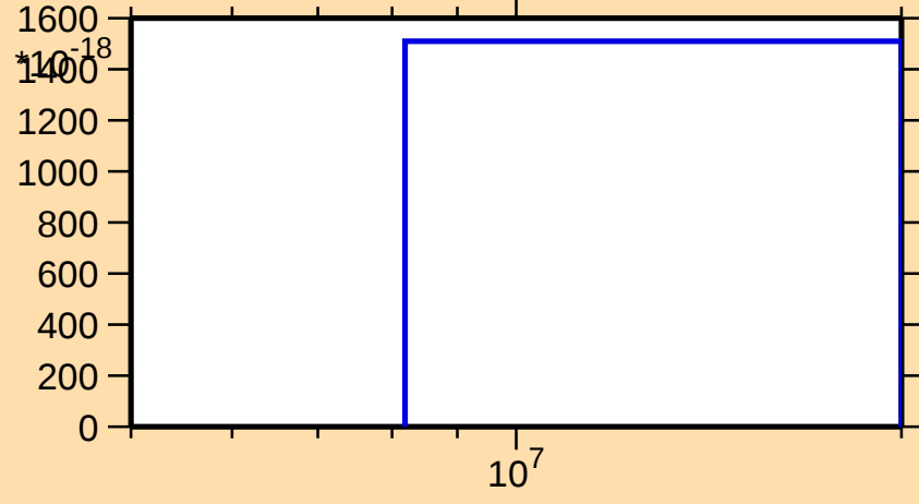
\sigma vs. E for ^{176}\text{W}(\text{n},\text{pt})
