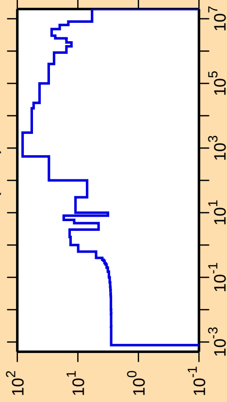
\Delta\sigma/\sigma vs. E for ^{176}\text{W}(\text{n,el.})
