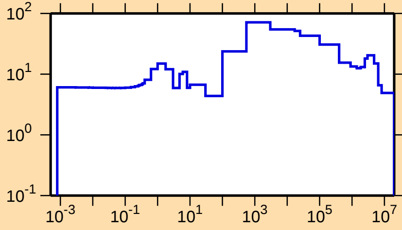
\Delta\sigma/\sigma vs. E for ^{176}\text{W}(\text{n,tot.})
