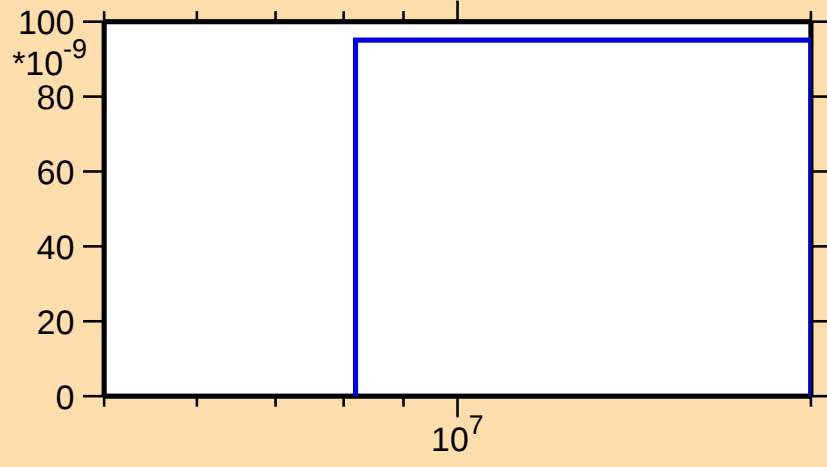
\sigma vs. E for ^{176}\text{W}(n,2n\alpha)
