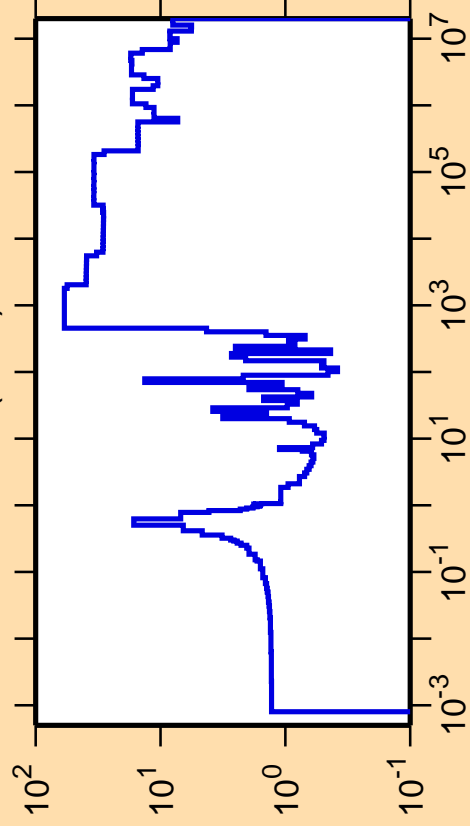
\Delta\sigma/\sigma vs. E for ^{178}\text{W}(n,\text{el.})
