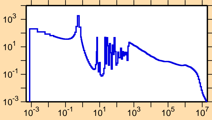
\sigma vs. E for ^{178}\text{W}(n,\gamma)
