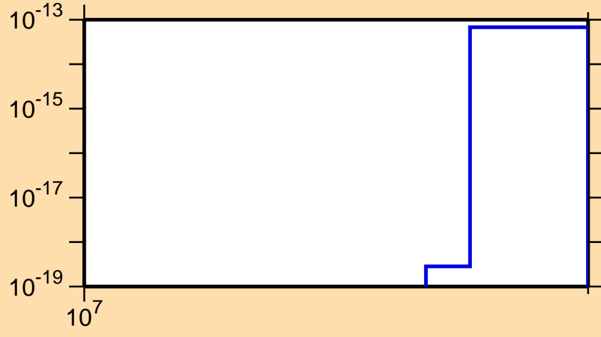
\sigma vs. E for ^{178}\text{W}(n,3n\alpha)
