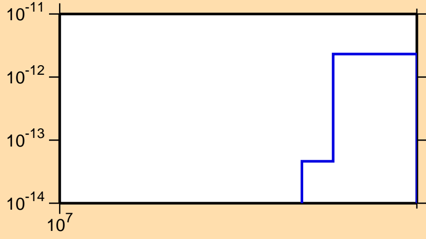
\sigma vs. E for ^{178}\text{W}(n,\text{pd})
