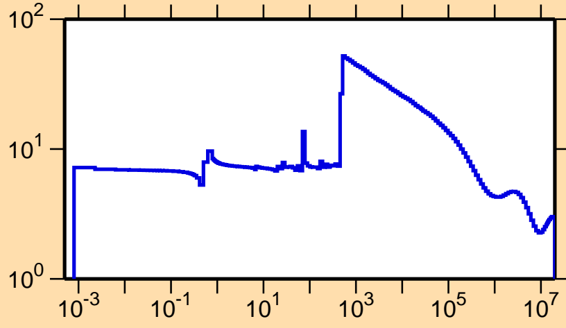
\sigma vs. E for ^{178}\text{W}(n,\text{el.})
