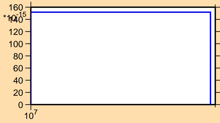
\sigma vs. E for ^{178}\text{W} (mt 45)
