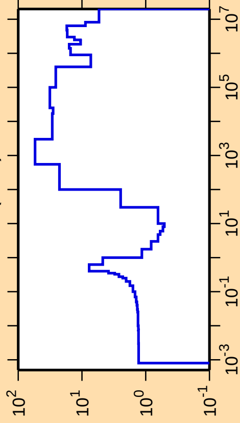
\Delta\sigma/\sigma vs. E for ^{178}\text{W}(\text{n,el.})
