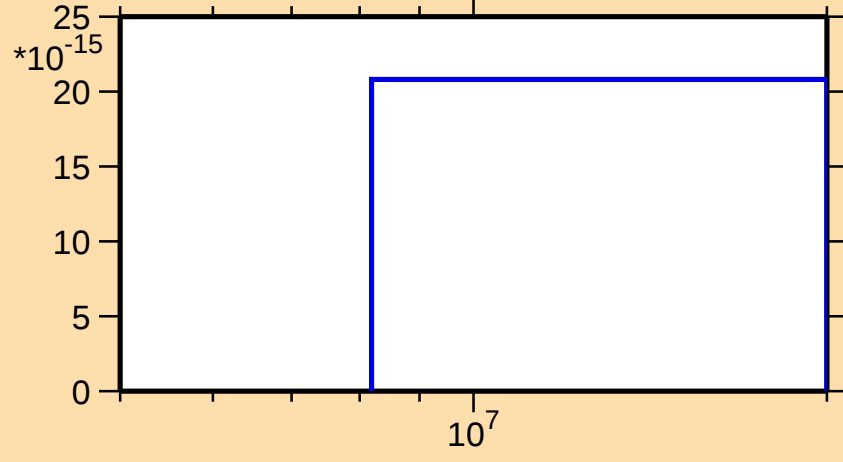
\sigma vs. E for ^{178}\text{W}(\text{n,pd})
