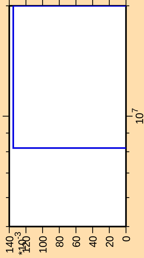
\Delta\sigma/\sigma vs. E for ^{178}\text{W}(\text{n,pd})
