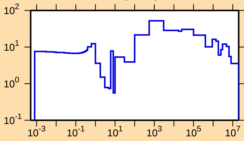
\Delta\sigma/\sigma vs. E for ^{178}\text{W}(\text{n,tot.})
