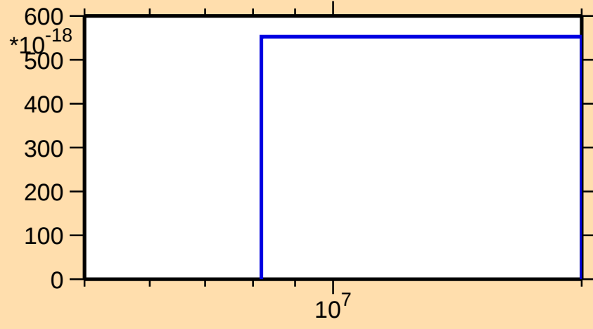
\sigma vs. E for ^{178}\text{W}(n,3n\alpha)
