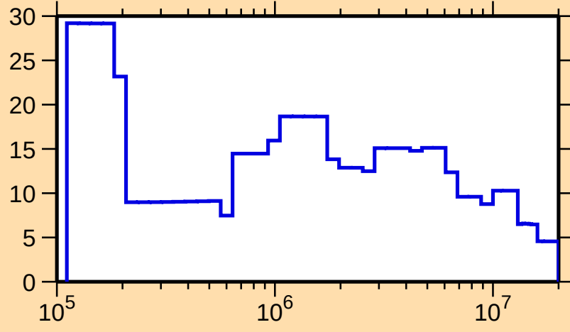
\Delta\sigma/\sigma vs. E for ^{179}\text{W}(\text{n,el.})
