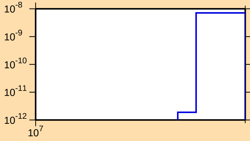
\sigma vs. E for ^{179}\text{W}(n,nt)
