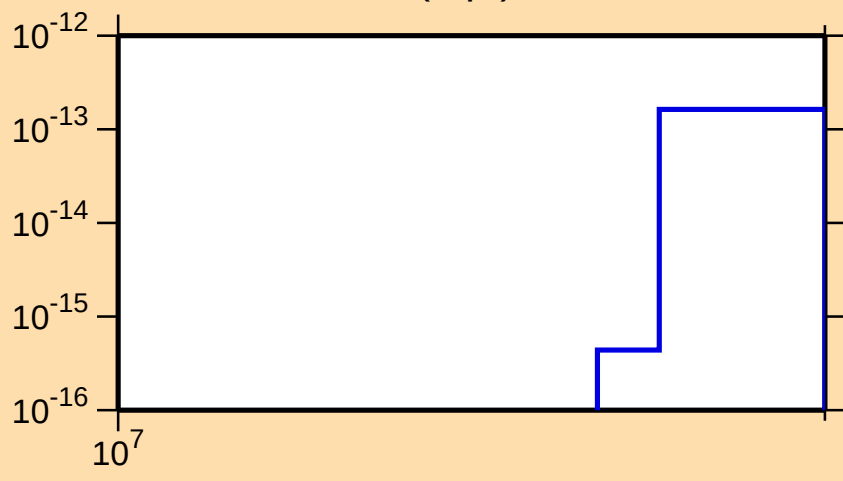
\sigma vs. E for ^{179}\text{W}(n,\text{pt})
