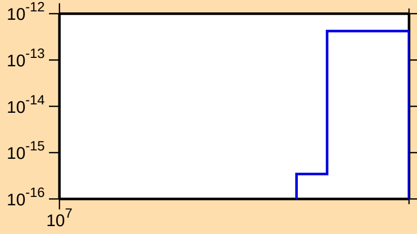
\sigma vs. E for ^{179}\text{W}(\text{mt 34})
