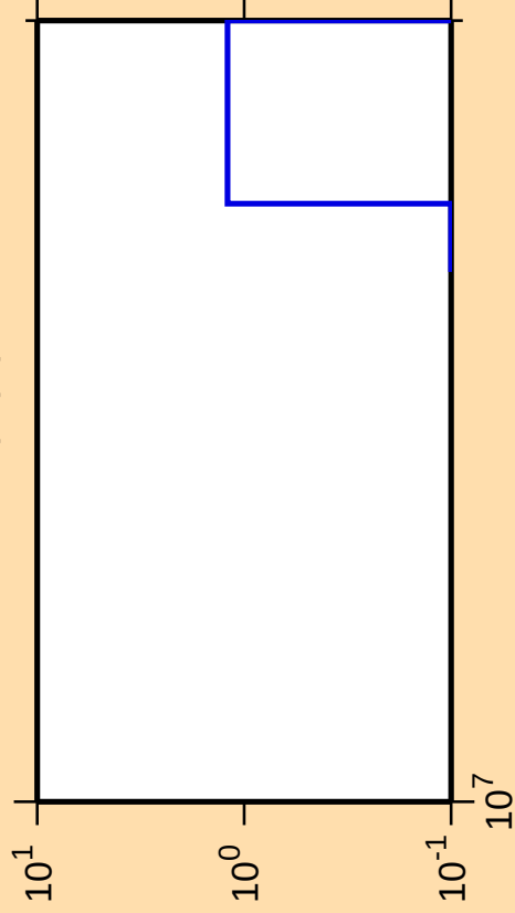
\Delta\sigma/\sigma vs. E for ^{179}\text{W}(n,\text{pt})
