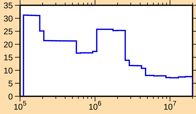
\Delta\sigma/\sigma vs. E for ^{179}\text{W}(n,\text{nonel.})
