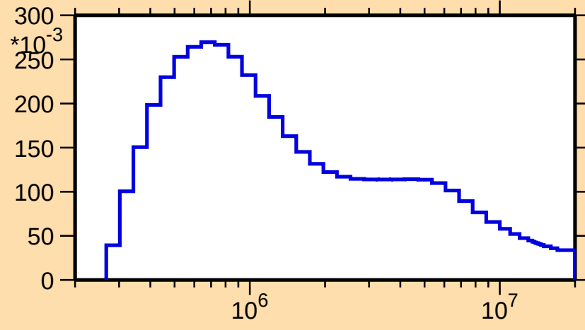
\sigma vs. E for ^{179}\text{W}(n,n_3)
