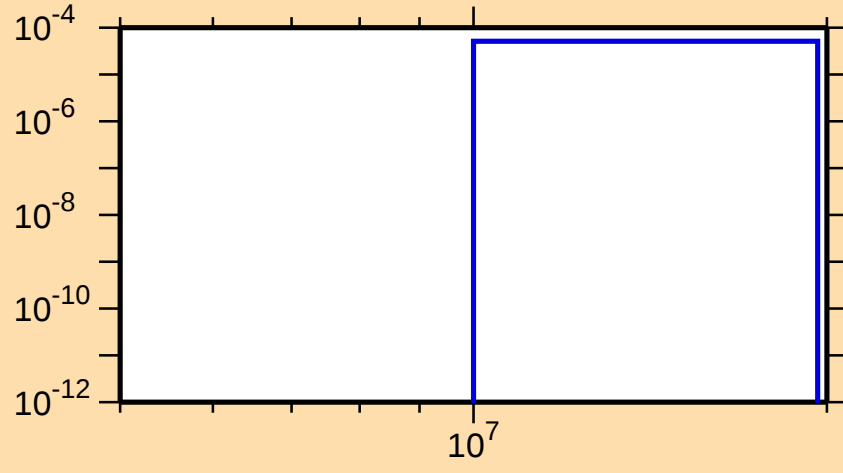
\sigma vs. E for ^{179}\text{W}(n,t)
