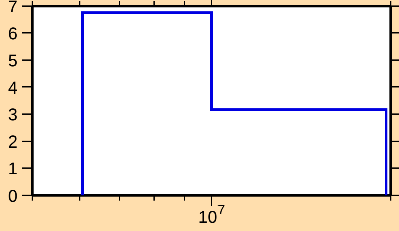
\Delta\sigma/\sigma vs. E for ^{179}\text{W}(n,\text{tot.})
