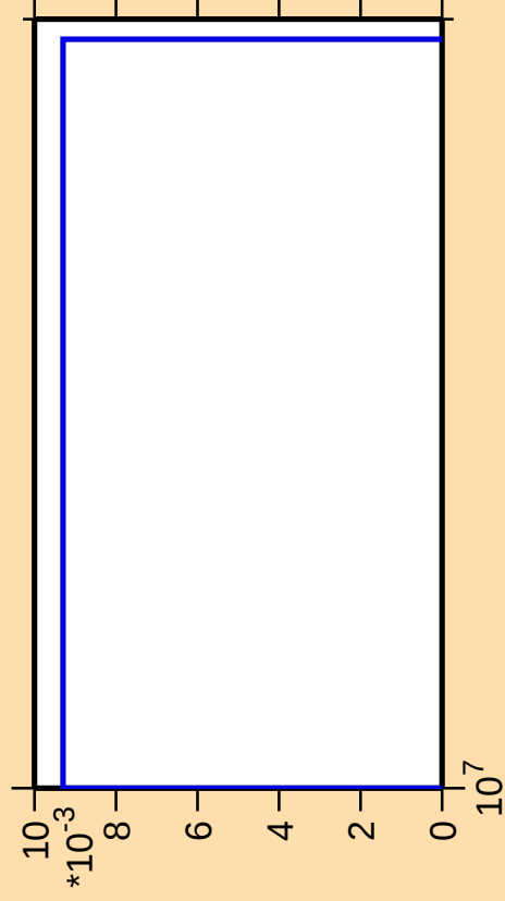
\Delta\sigma/\sigma vs. E for ^{179}\text{W}(\text{n,pt})
