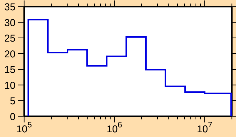
\Delta\sigma/\sigma vs. E for ^{179}\text{W}(\text{n,nonel.})
