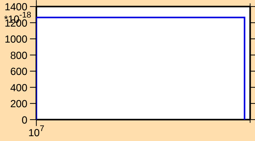
\sigma vs. E for ^{179}\text{W}(\text{n,pt})
