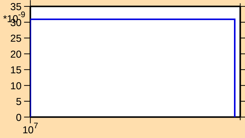
\sigma vs. E for ^{179}\text{W}(\text{n},\text{nd})
