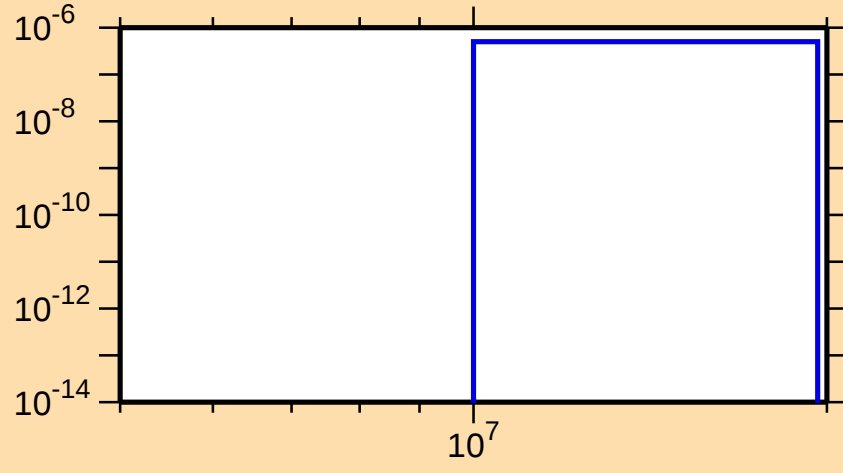
\sigma vs. E for ^{179}\text{W}(n,2n\alpha)
