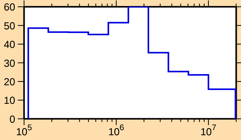
\Delta\sigma/\sigma vs. E for ^{179}\text{W}(n,n_1)
