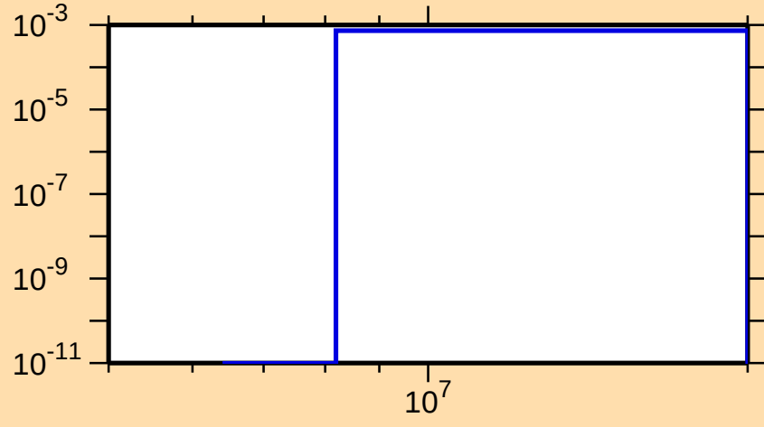
\sigma vs. E for ^{179}\text{W}(n,d)
