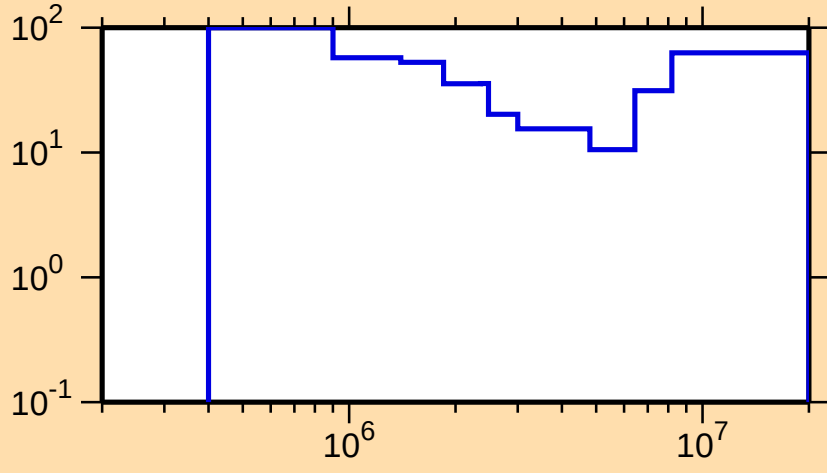
\Delta\sigma/\sigma vs. E for ^{179}\text{W}(n,ncont.)
