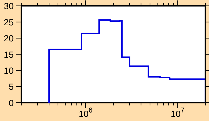
\Delta\sigma/\sigma vs. E for ^{179}\text{W}(n,n\text{onel.})
