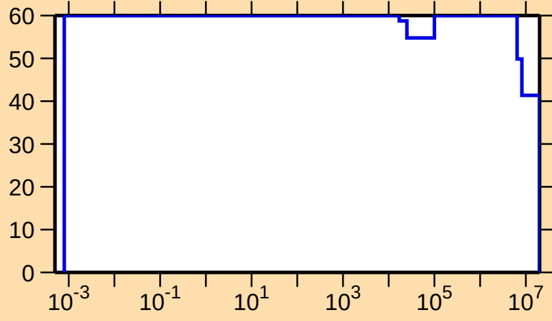
\Delta\sigma/\sigma vs. E for ^{179}\text{W}(n,p)
