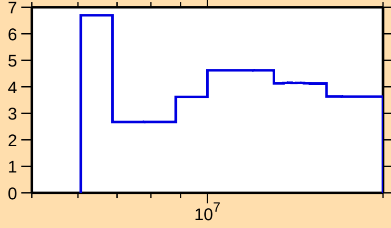
\Delta\sigma/\sigma vs. E for ^{179}\text{W}(n,\text{el.})
