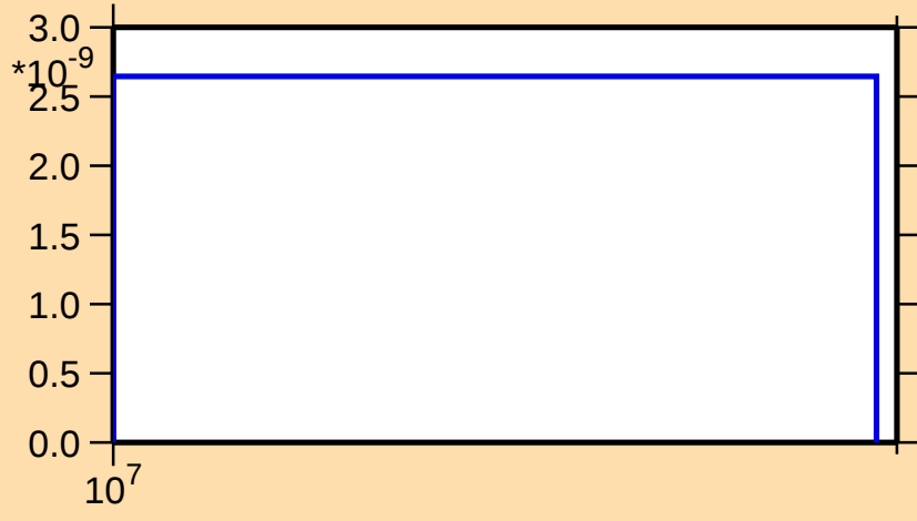
\sigma vs. E for ^{180}\text{W}(\text{n},\text{nd})
