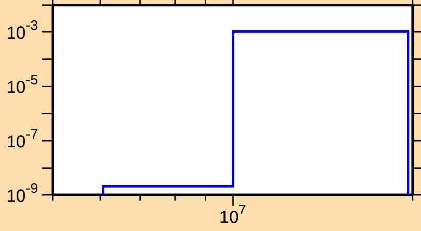
\sigma vs. E for ^{180}\text{W}(n,np)
