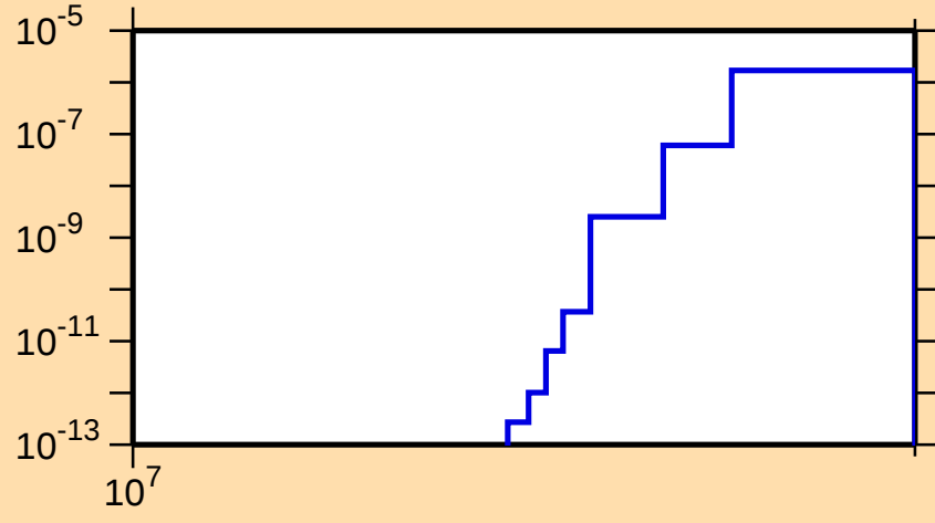
\sigma vs. E for ^{181}\text{W}(n,\text{nd})
