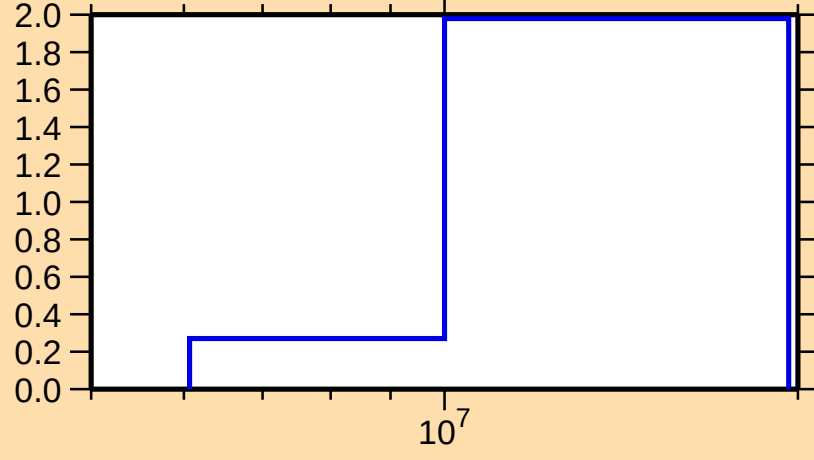
\sigma vs. E for ^{181}\text{W}(n,2n)
