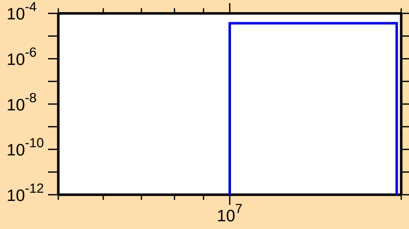
\sigma vs. E for ^{181}\text{W}(n,t)
