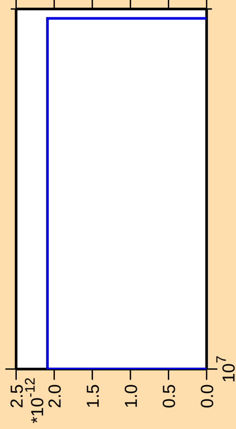
\Delta\sigma/\sigma vs. E for ^{181}\text{W}(\text{mt 11})
