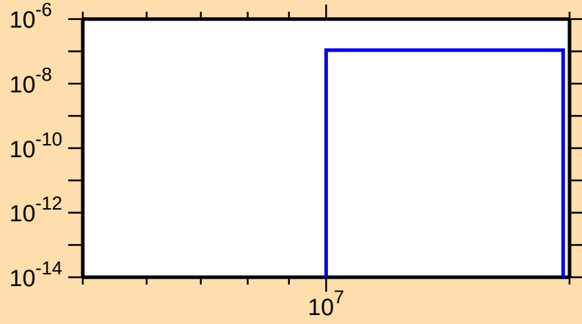
\sigma vs. E for ^{181}\text{W}(n,2n\alpha)
