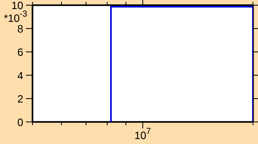
\sigma vs. E for ^{181}\text{W}(n,3n)
