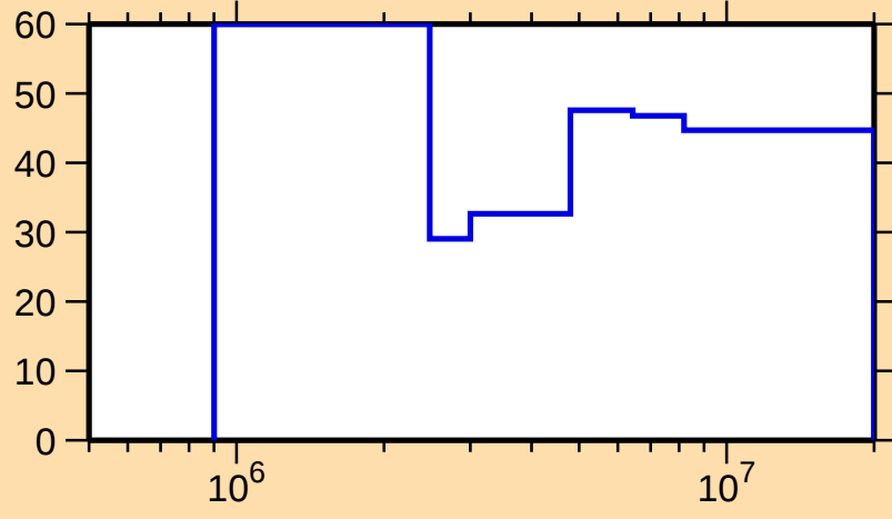
\Delta\sigma/\sigma vs. E for ^{181}\text{W}(n,n_1)
