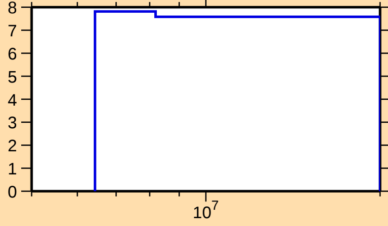
\Delta\sigma/\sigma vs. E for ^{181}\text{W}(n,\text{nonel.})
