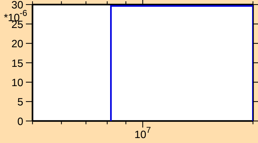
\sigma vs. E for ^{181}\text{W}(n,t)
