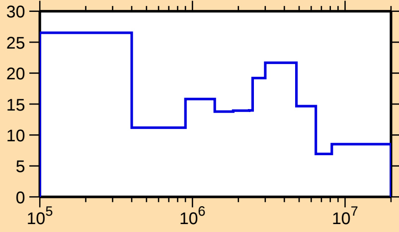
\Delta\sigma/\sigma vs. E for ^{181}\text{W}(n,\text{el.})
