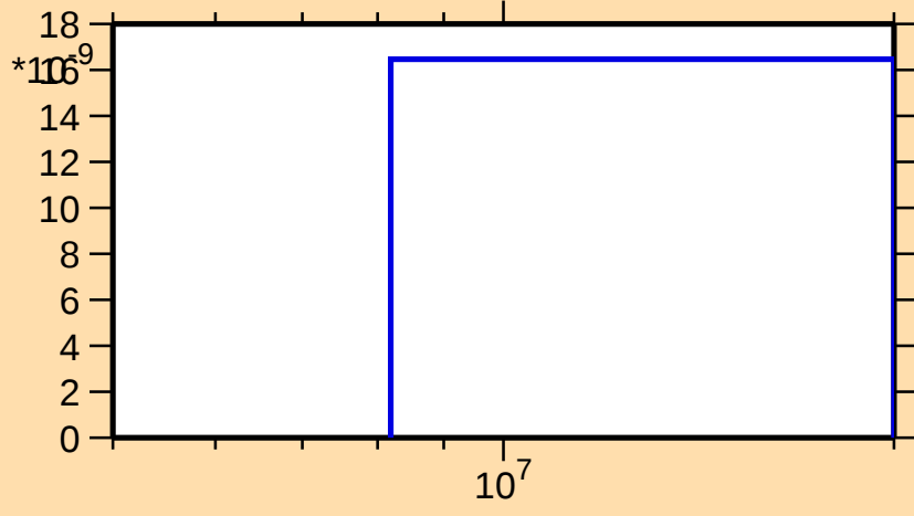
\sigma vs. E for ^{181}\text{W}(\text{n},\text{nd})
