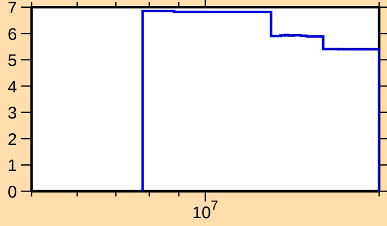
\Delta\sigma/\sigma vs. E for ^{182}\text{W}(n,2n)
