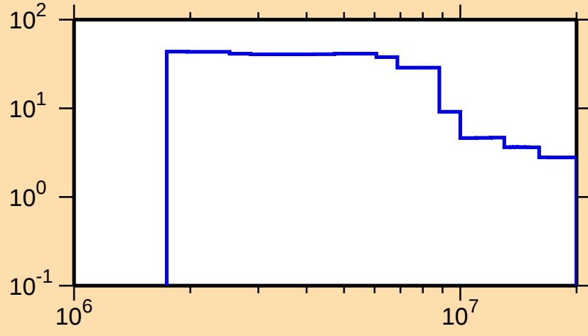
\Delta\sigma/\sigma vs. E for ^{182}\text{W}(\text{n},\text{nonel.})
