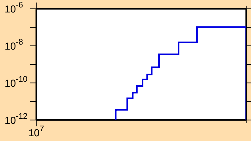
\sigma vs. E for ^{182}\text{W}(n,2n\alpha)
