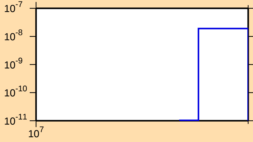
\sigma vs. E for ^{182}\text{W}(n,nt)
