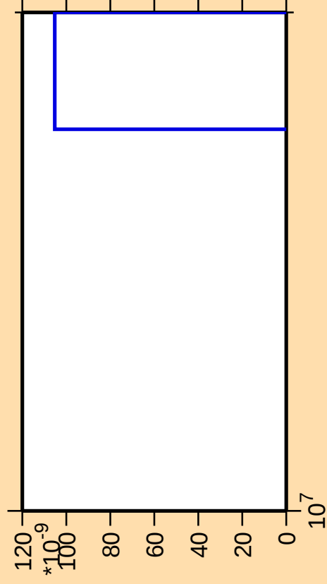
\Delta\sigma/\sigma vs. E for ^{182}\text{W} (mt 11)
