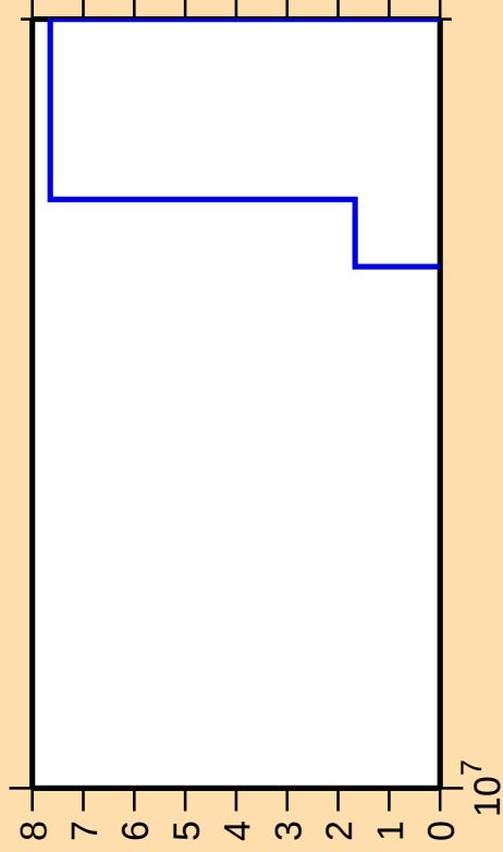
\Delta\sigma/\sigma vs. E for ^{182}\text{W}(n,p\alpha)
