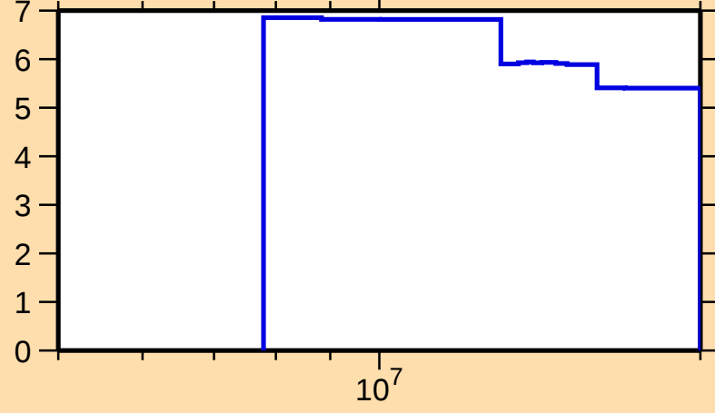
\Delta\sigma/\sigma vs. E for ^{182}\text{W}(n,2n)
