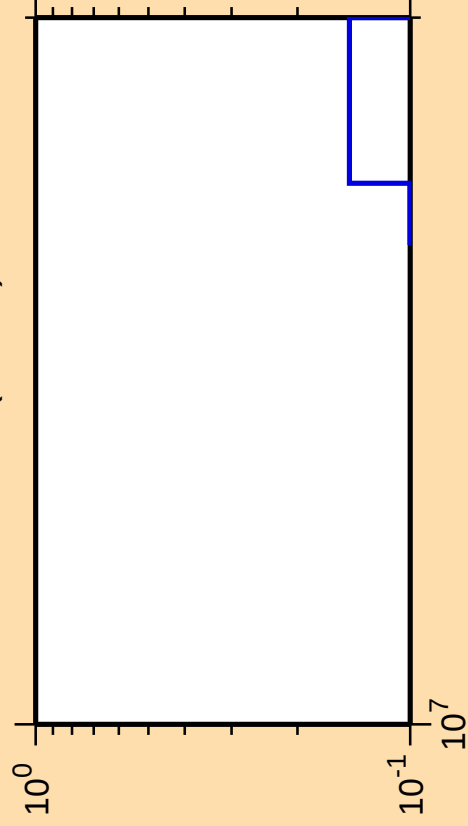
\Delta\sigma/\sigma vs. E for ^{182}\text{W}(n,3n\alpha)
