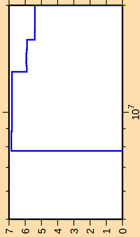
\Delta\sigma/\sigma vs. E for ^{182}\text{W}(n,2n)
