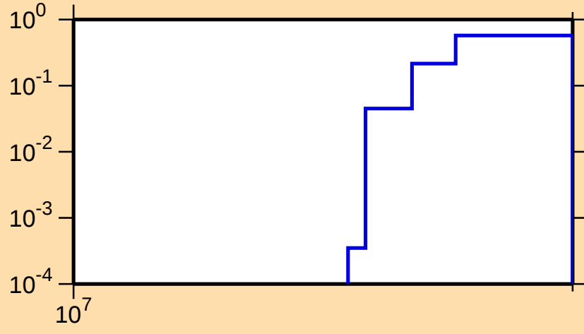
\sigma vs. E for ^{182}\text{W}(n,3n)
