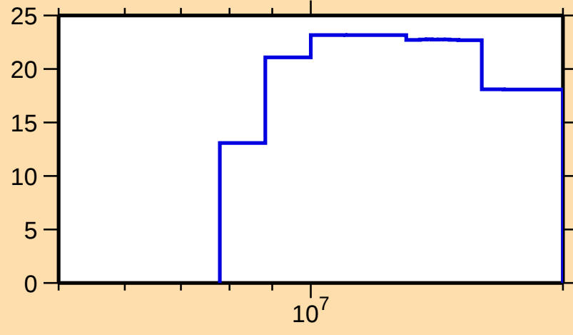
\Delta\sigma/\sigma vs. E for ^{182}\text{W}(n,\text{el.})
