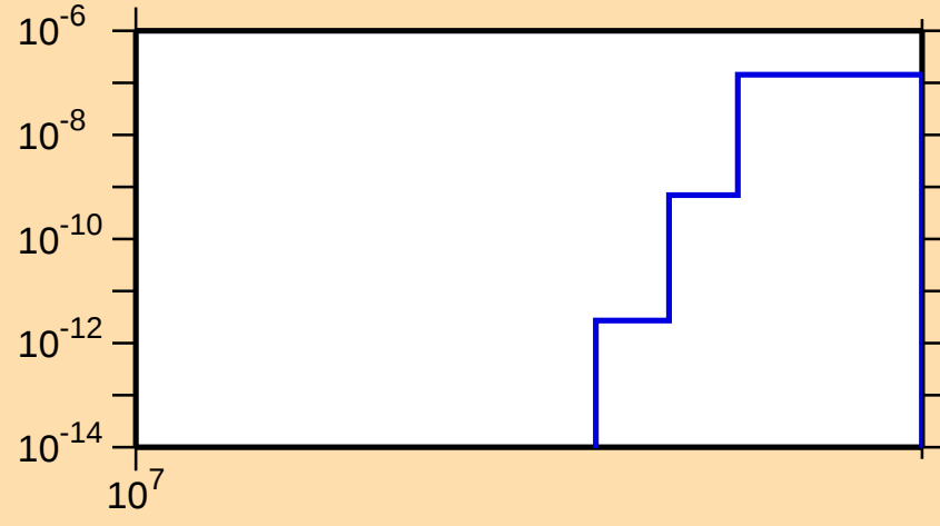
\sigma vs. E for ^{182}\text{W}(n,\text{nd})
