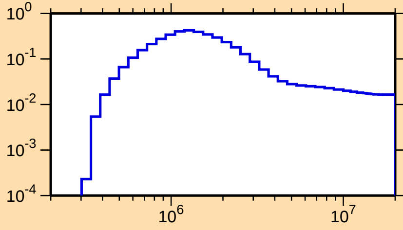
\sigma vs. E for ^{182}\text{W}(n,n_2)
