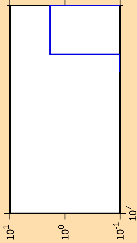
\Delta\sigma/\sigma vs. E for ^{183}\text{W}(n,3n\alpha)
