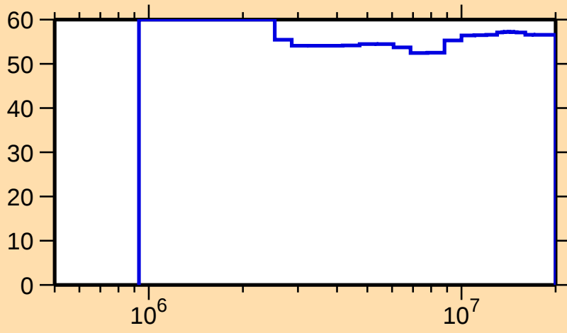
\Delta\sigma/\sigma vs. E for ^{183}\text{W}(n,n\text{cont.})
