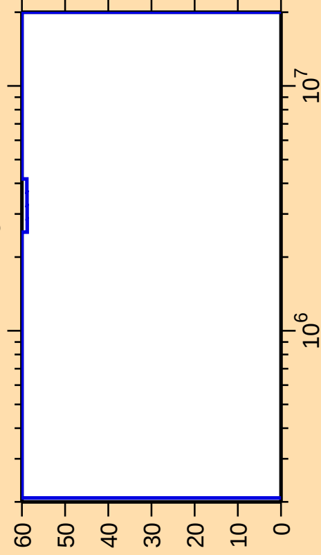
\Delta\sigma/\sigma vs. E for ^{183}\text{W}(n,n_3)
