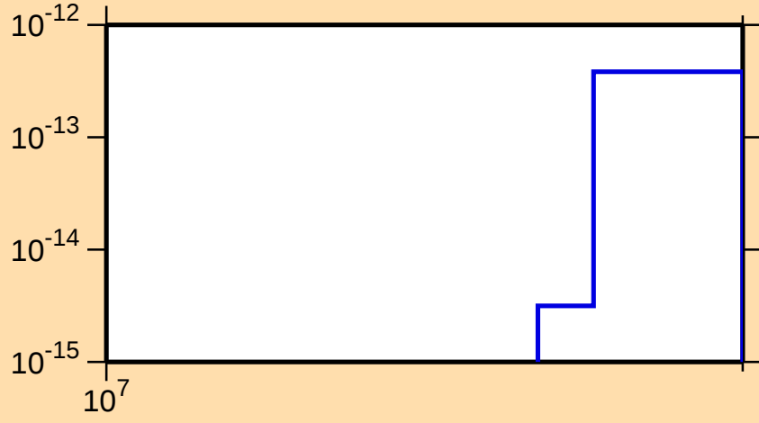
\sigma vs. E for ^{183}\text{W}(n,3n\alpha)
