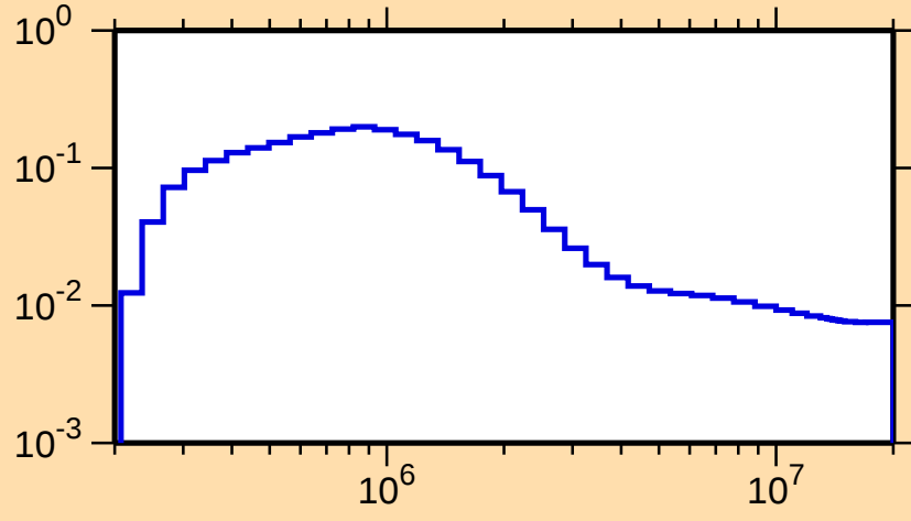
\sigma vs. E for ^{183}\text{W}(n,n_3)
