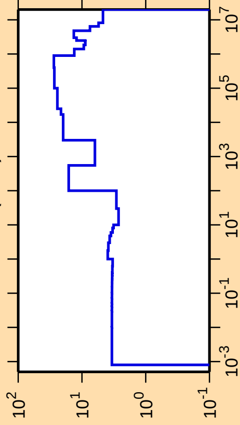
\Delta\sigma/\sigma vs. E for ^{183}\text{W}(\text{n,el.})
