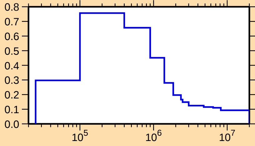
\sigma vs. E for ^{183}\text{W}(n,n_1)
