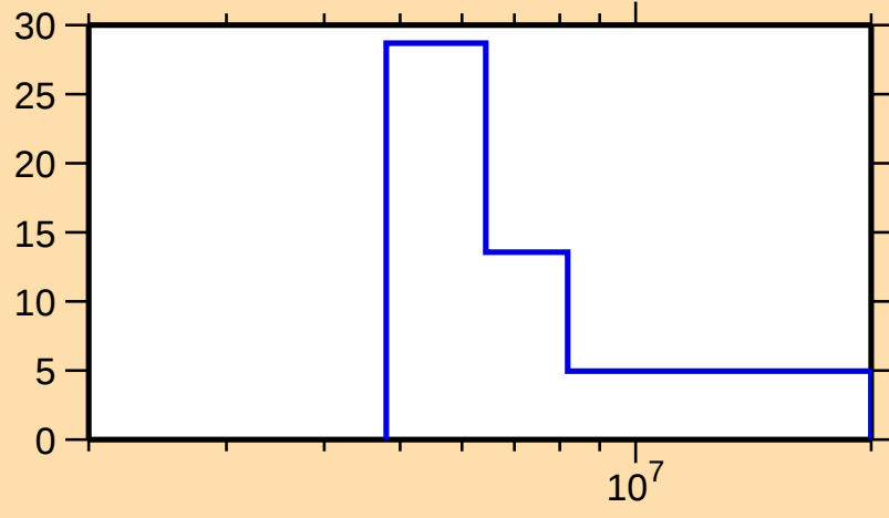
\Delta\sigma/\sigma vs. E for ^{183}\text{W}(n,\text{tot.})
