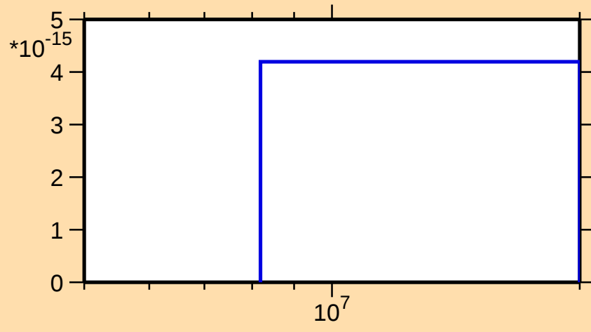
\sigma vs. E for ^{183}\text{W}(n,3n\alpha)
