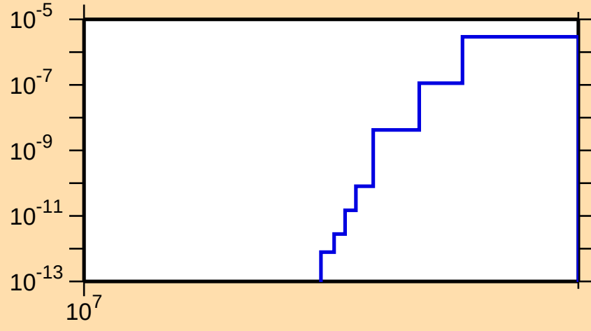
\sigma vs. E for ^{183}\text{W}(n,\text{nd})
