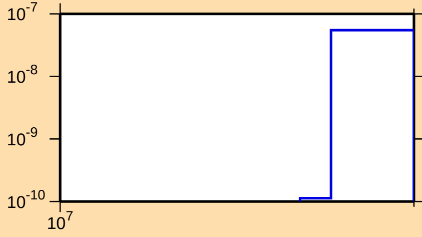
\sigma vs. E for ^{183}\text{W}(n,\text{nt})
