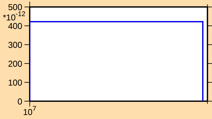
\sigma vs. E for ^{183}\text{W}(n,nt)
