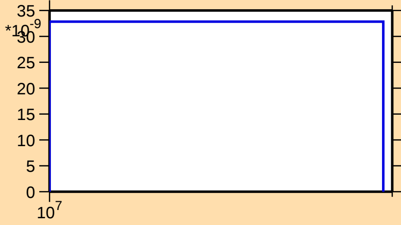
\sigma vs. E for ^{183}\text{W}(n,\text{nd})
