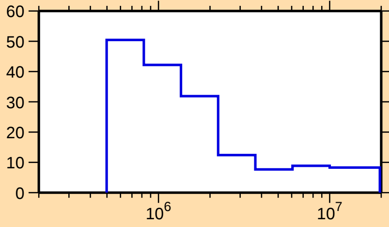
\Delta\sigma/\sigma vs. E for ^{183}\text{W}(\text{n},\text{nonel.})
