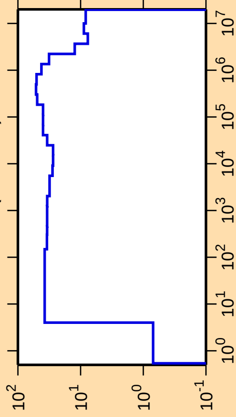
\Delta\sigma/\sigma vs. E for ^{183}\text{W}(n,\text{nonel.})
