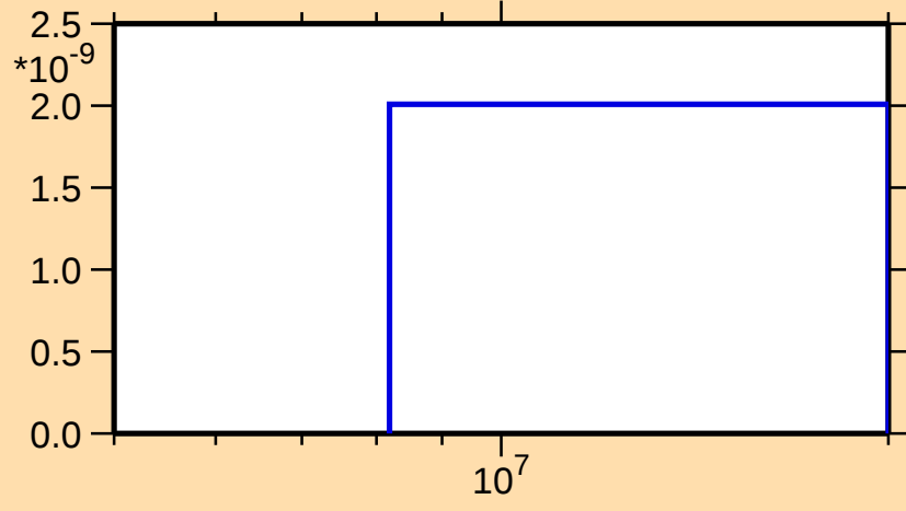
\sigma vs. E for ^{184}\text{W}(n,2n\alpha)
