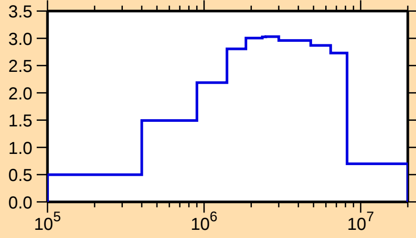
\sigma vs. E for ^{184}\text{W}(\text{n,inel.})
