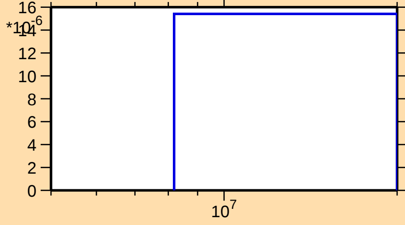
\sigma vs. E for ^{184}\text{W}(n,t)
