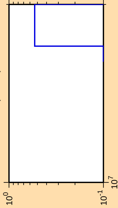
\Delta\sigma/\sigma vs. E for ^{185}\text{W}(n,3n\alpha)
