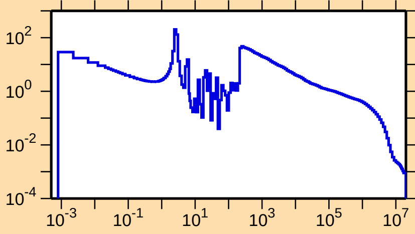
\sigma vs. E for ^{185}\text{W}(n,\gamma)
