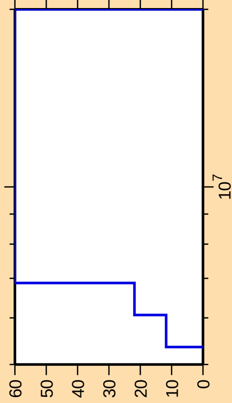
\Delta\sigma/\sigma vs. E for ^{185}\text{W}(n,\text{ncont.})
