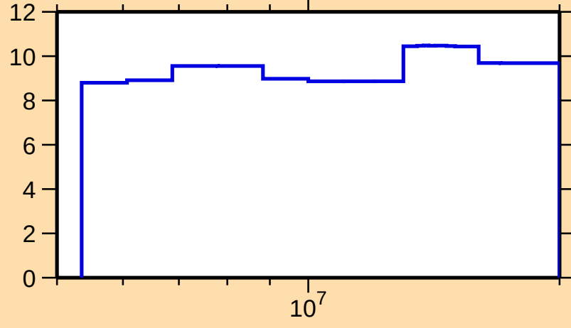
\Delta\sigma/\sigma vs. E for ^{185}\text{W}(n,\text{nonel.})
