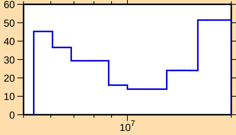
\Delta\sigma/\sigma vs. E for ^{185}\text{W}(n,2n)
