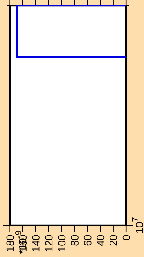
\Delta\sigma/\sigma vs. E for ^{185}\text{W} (mt 11)
