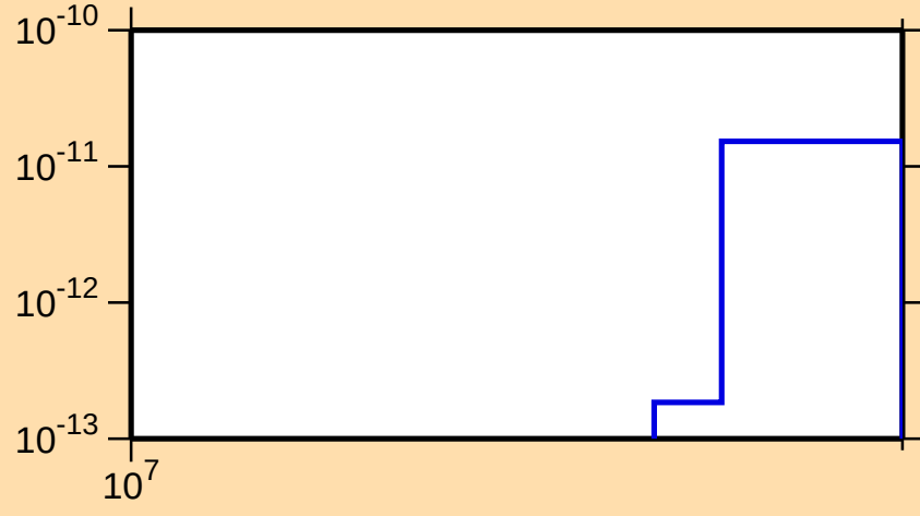
\sigma vs. E for ^{185}\text{W}(n,\text{He3})
