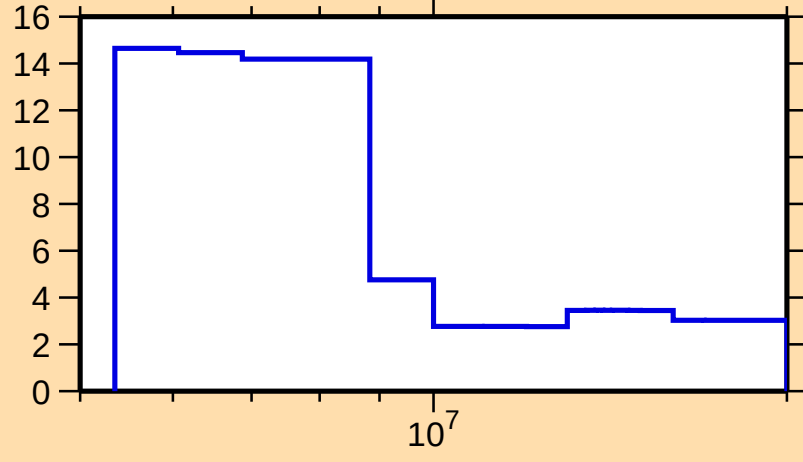
\Delta\sigma/\sigma vs. E for ^{185}\text{W}(n,\text{tot.})
